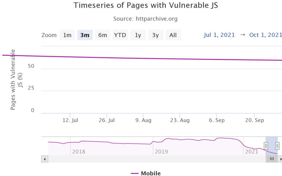
Figure 1.1 – Web pages with vulnerable JavaScript code (source: https://httparchive.org/reports/state-of-the-web )
