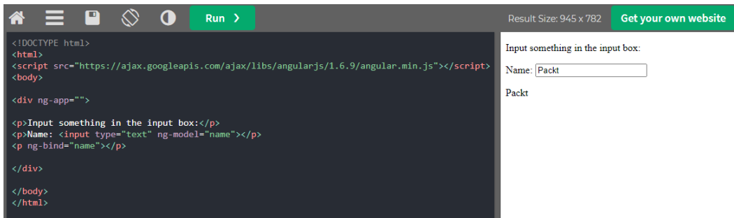
Figure 5.5 – Basic AngularJS web application code snippet (source: https://www.w3schools.com/angular/tryit.asp?filename=try_ng_intro )
