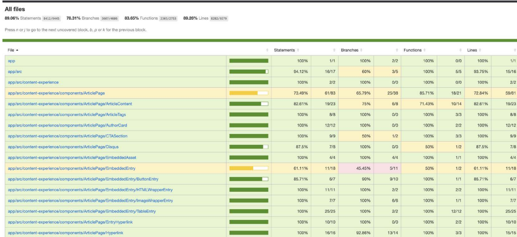
Figure 8.4 – Code coverage report for the Zoopla website using Cypress and the Istanbul plugin (source: https://www.mariedrake.com/post/generating-code-coverage-report-for-cypress )
