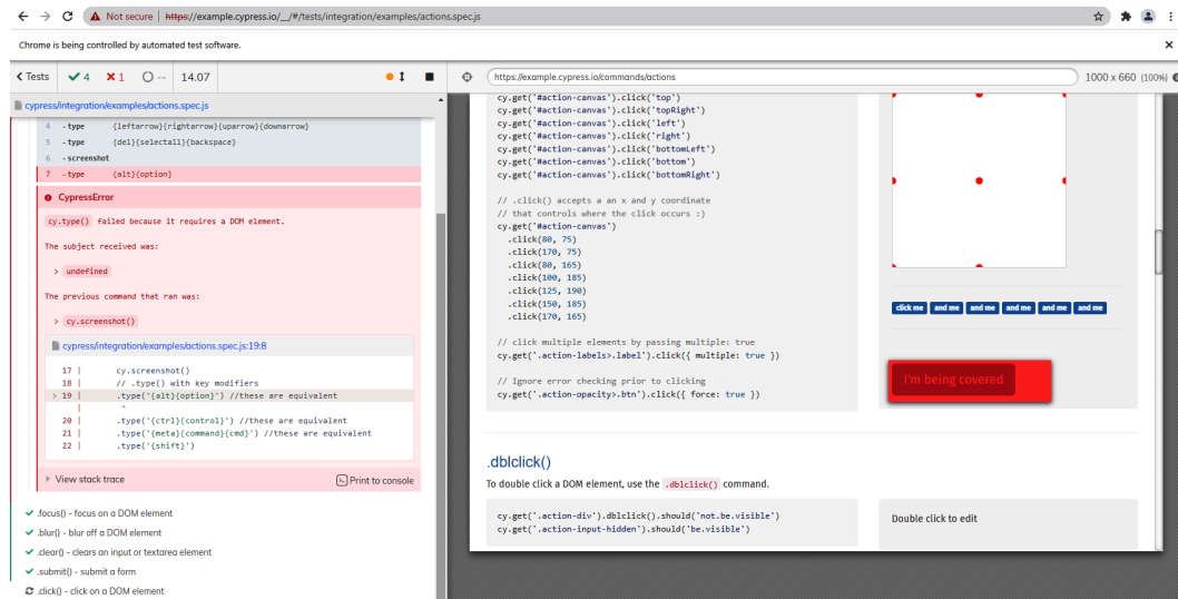
Figure 3.9 – Cypress live execution of a JavaScript test scenario on a local browser
