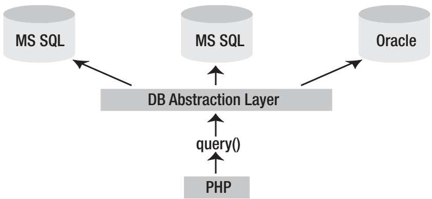
Figure 28-1. Using a database abstraction layer to decouple the application and data layers
