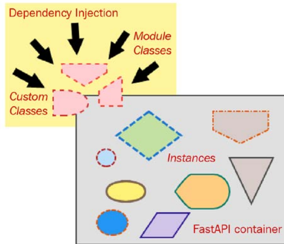
Figure 3.1 – The IoC principle
