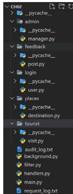
Figure 2.1 – The FastAPI project structure
