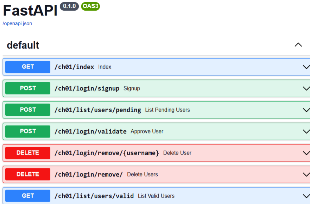
Figure 1.2 – A Swagger OpenAPI dashboard
