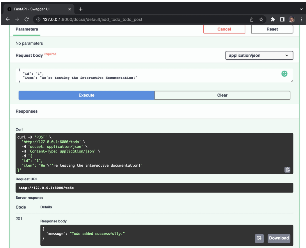
Figure 2.2 – Route test from interactive documentation
