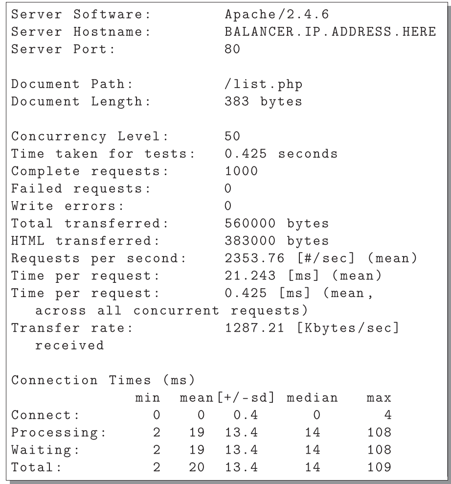
Figure 6-5. ApacheBench Output for Cached Configuration
