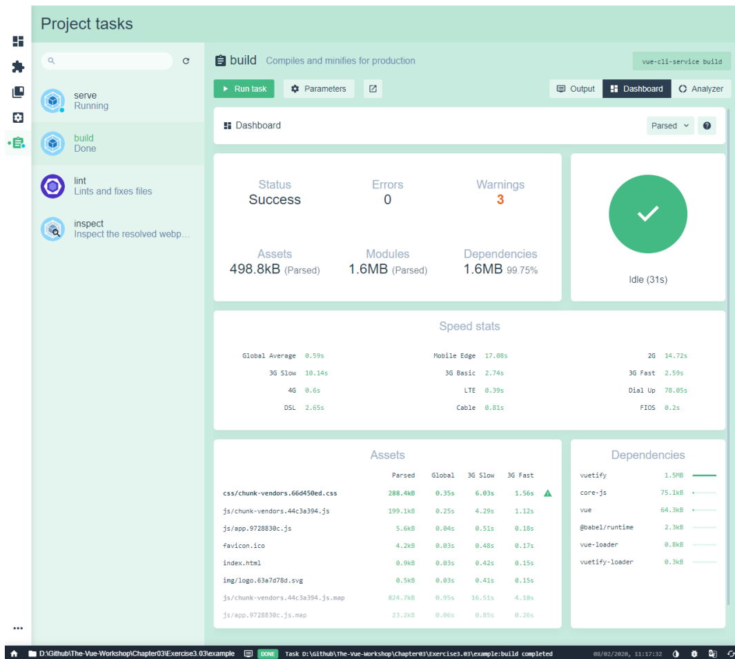
Figure 3.25: When a build is complete, you have a dashboard of useful analytics
