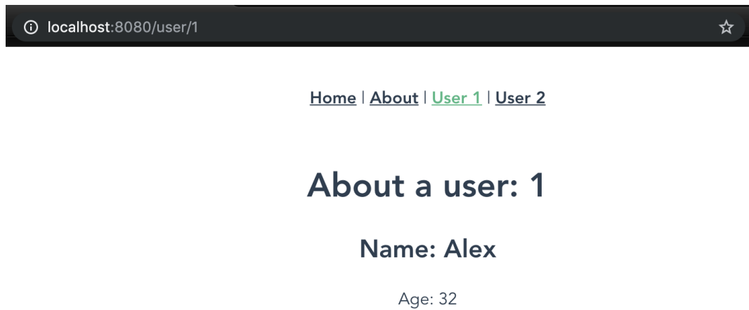
Figure 6.34: Navigate to /user/1 with updated UI
