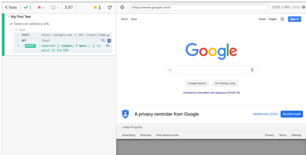
Figure 13.4: Cypress tests running in Chrome while visiting the Google home page
