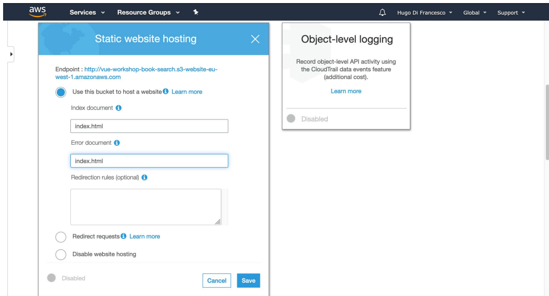
Figure 14.58: The S3 bucket properties page with web hosting enabled and configured with the index and error page set to index.html
