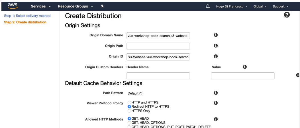
Figure 14.79: The CloudFront Distribution creation page with the origin domain set to the S3 bucket
