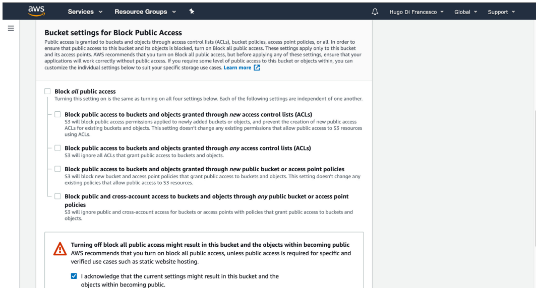
Figure 14.57: The S3 bucket creation page with public access enabled and the relevant disclaimer accepted
