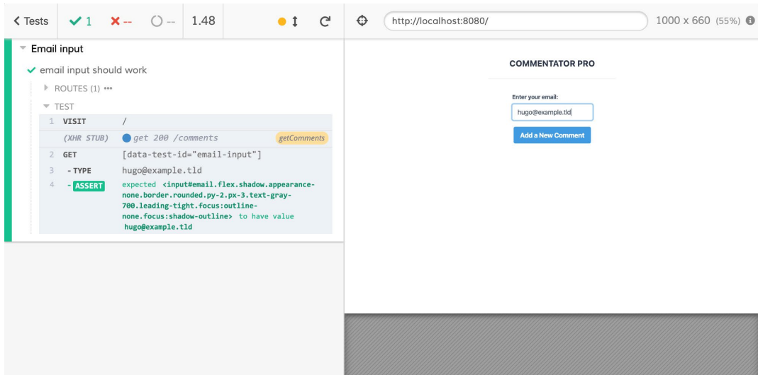
Figure 13.24: Cypress running "enter-email" tests, with the email input test
