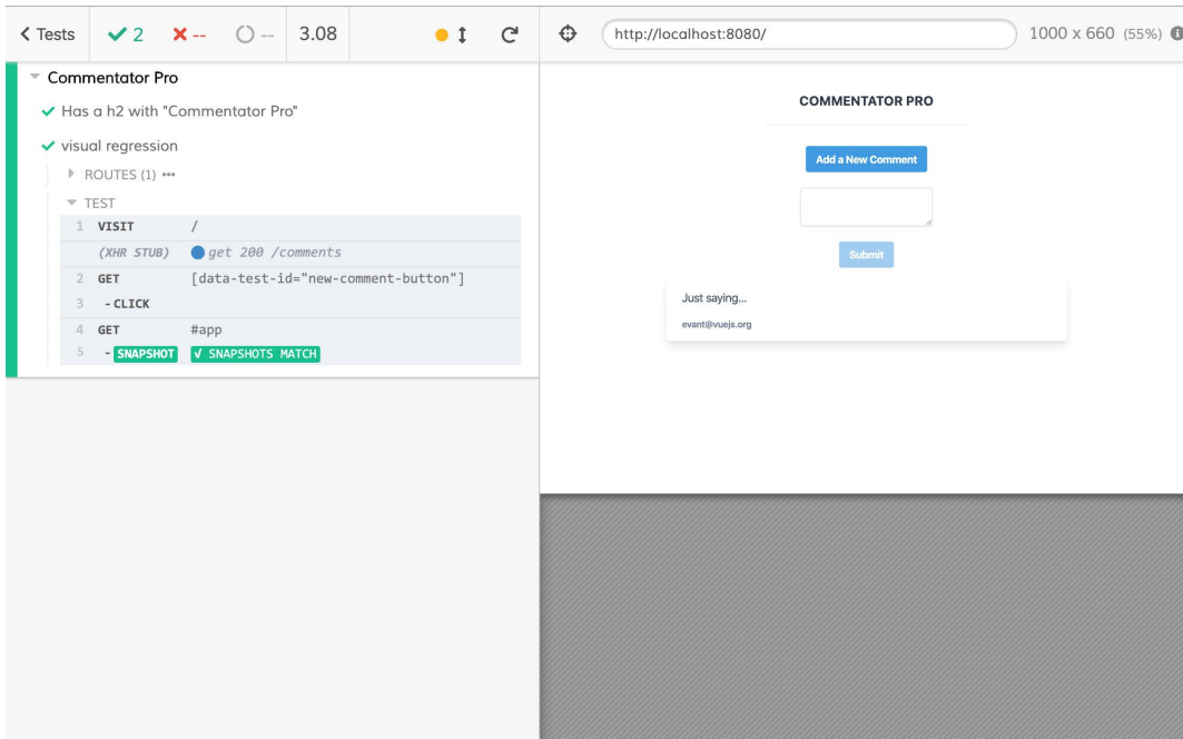
Figure 13.18: Cypress running tests, including the visual regression test
