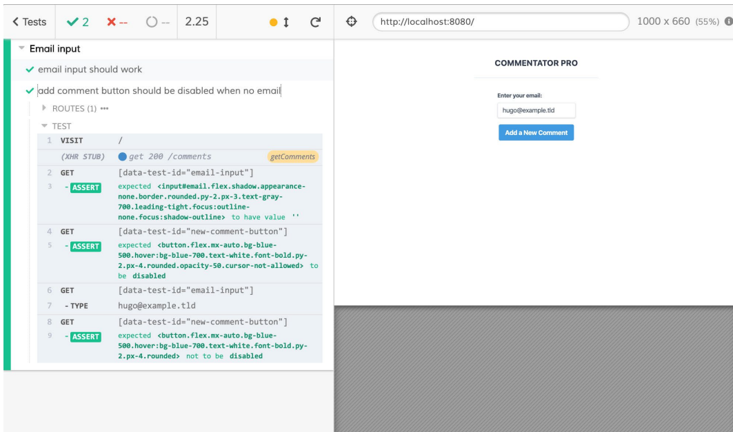
Figure 13.22: Cypress running "enter-email" tests, with the disabled add comment button test
