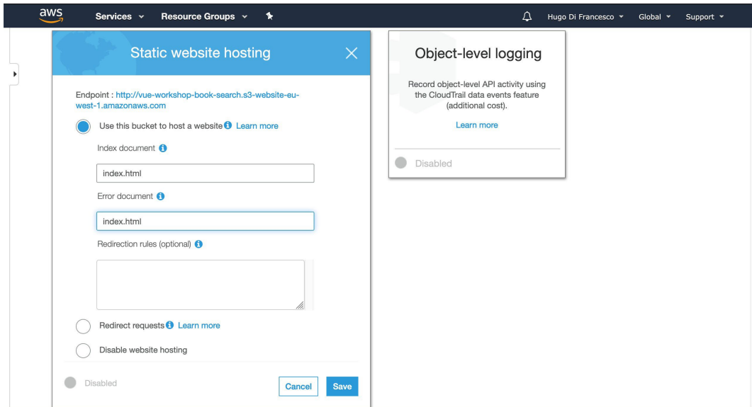
Figure 14.73: The S3 bucket properties page with web hosting enabled and configured with the index and error page set to index.html
