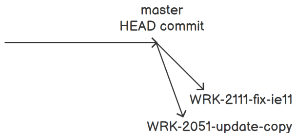
Figure 14.3: A sample trunk-based Git commit/branch tree with two feature branches branched off of the master
