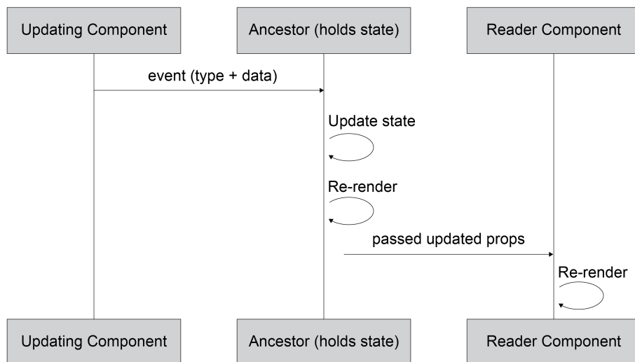
Figure 8.4: Updating a sibling component when the ancestor holds state
