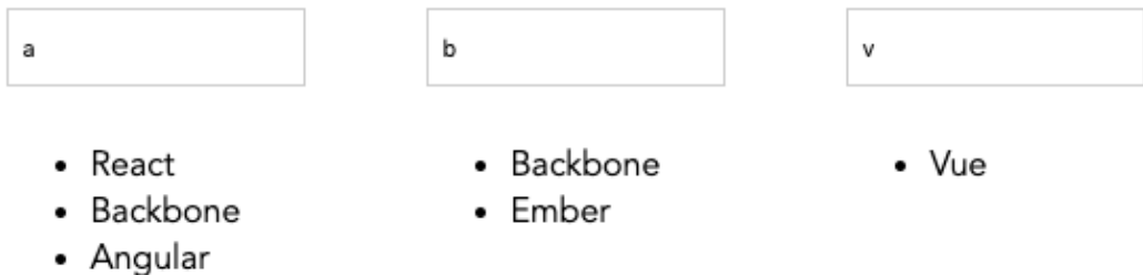
Figure 2.11: Filtering the list using a watcher in the third column
