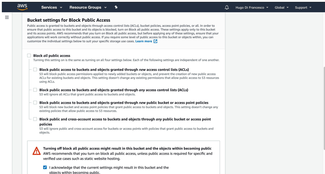
Figure 14.72: The S3 bucket creation page with public access enabled and the relevant disclaimer accepted
