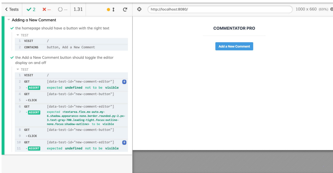
Figure 13.9: Cypress running "add-new-comment" tests, including the new editor-toggling test
