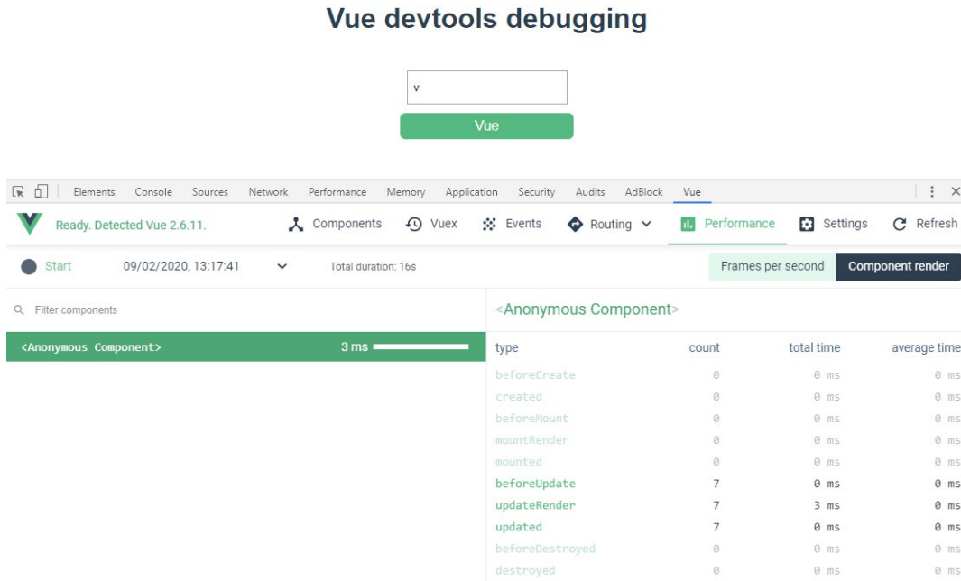
Figure 3.40: Selecting the component in the right-hand panel will open the lifecycle hooks on the left
