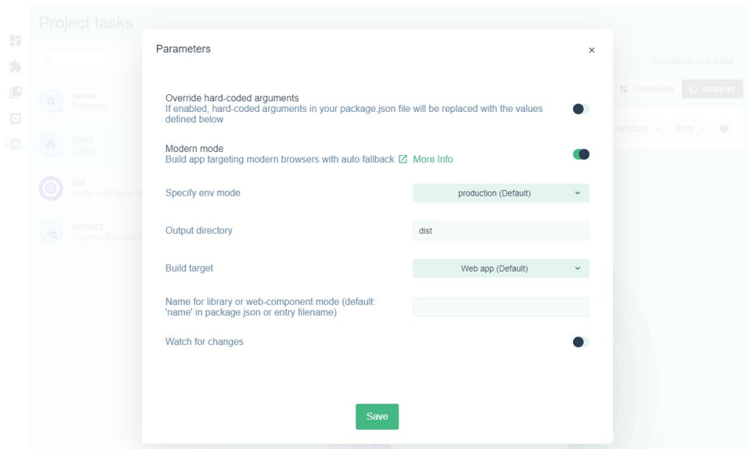
Figure 3.24: Vue-UI build parameters
