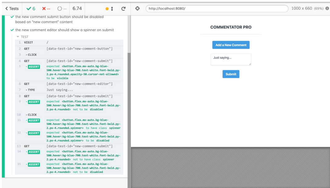
Figure 13.13: Cypress running "add-new-comment" tests, including the comment submission loading state test
