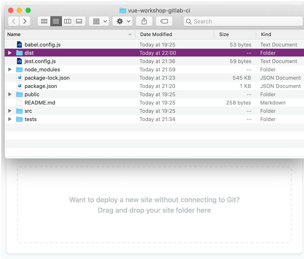
Figure 14.19: Dragging and dropping the dist folder onto the Netlify drag and drop deployment section
