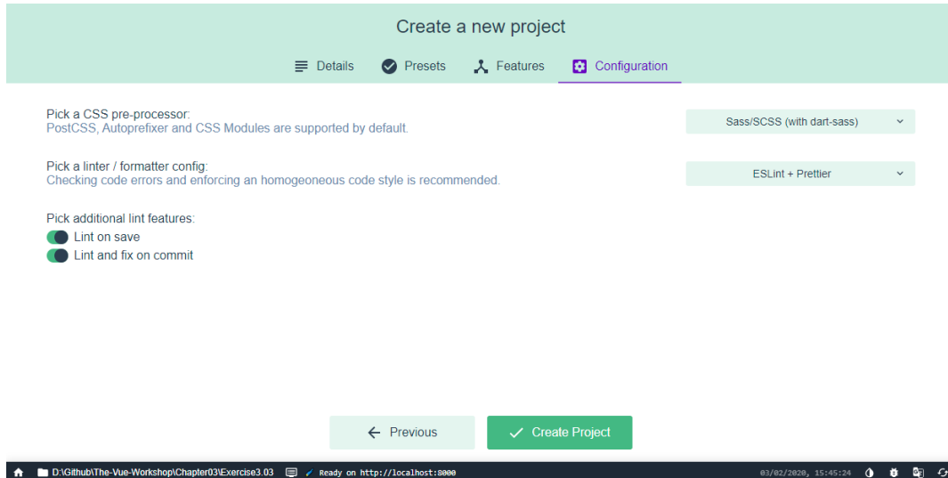
Figure 3.18: Enable configuration options for your new project in the Vue-UI
