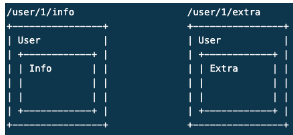
Figure 6.37: User with two nested views – Info and Extra
