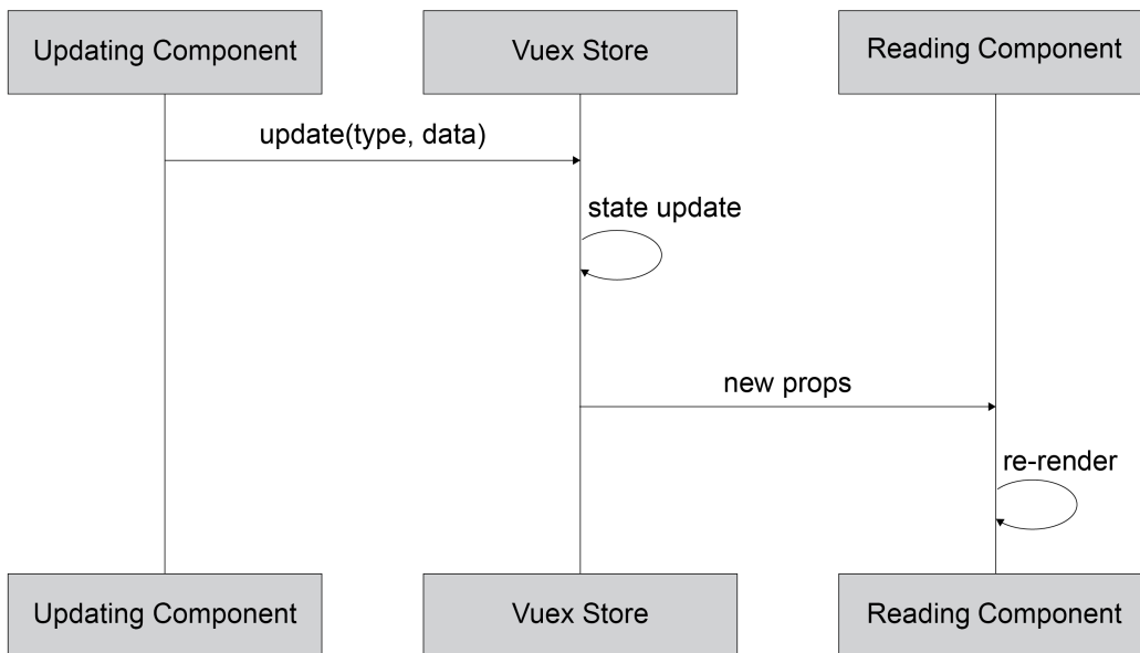
Figure 8.26: Sequence diagram of a global state update with Vuex
