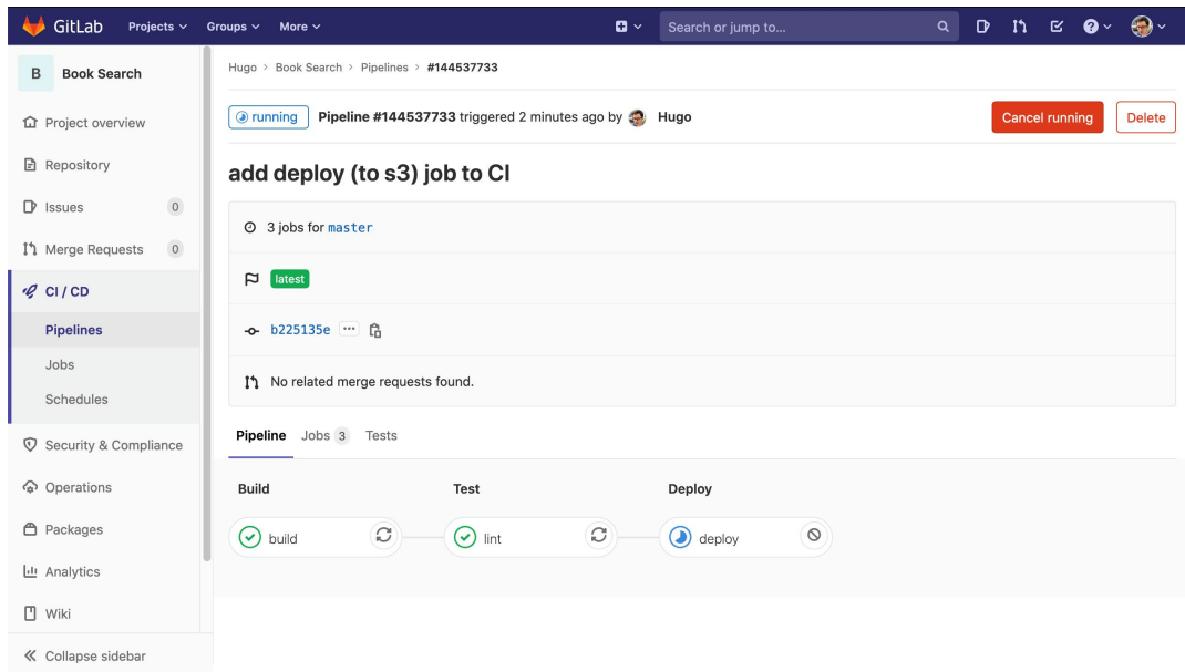
Figure 14.76: The GitLab CI/CD pipeline with the deploy job running
