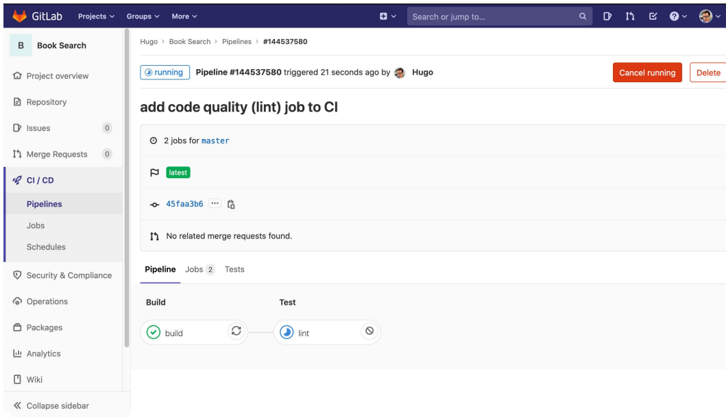
Figure 14.54: The GitLab CI/CD pipeline with the lint job running
