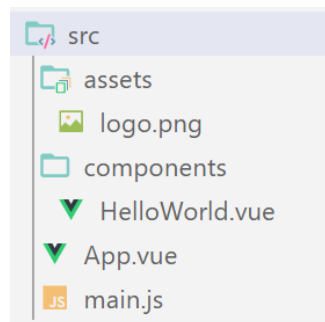
Figure 1.2: Default Vue application src folder structure
