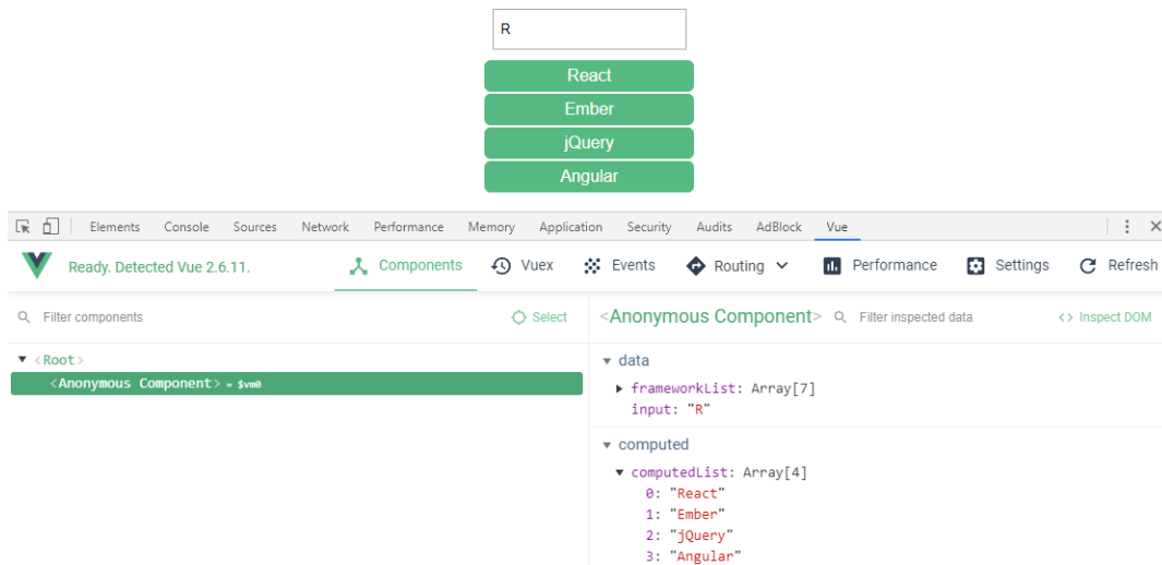
Figure 3.38: Computed list update to the value written inside of DevTools
