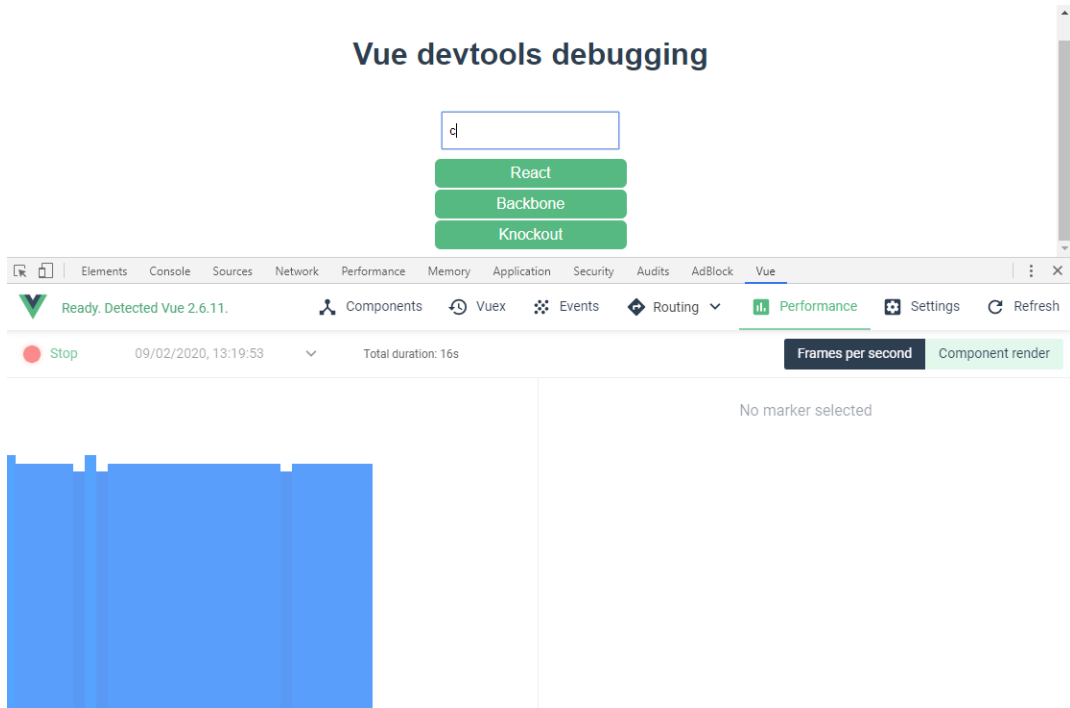
Figure 3.39: Computed list update to the value written inside of DevTools
