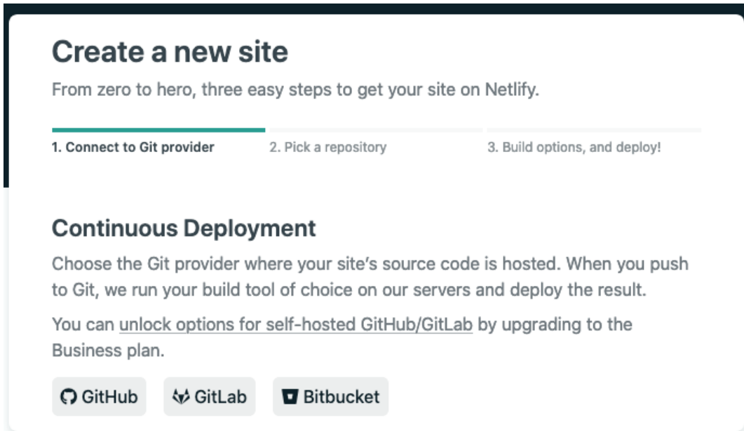
Figure 14.29: Continuous Deployment
