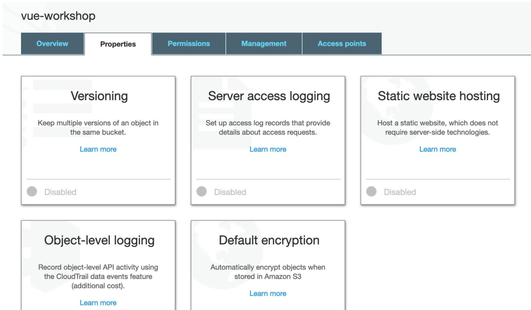
Figure 14.37: The Static website hosting option in the S3 bucket's Properties tab
