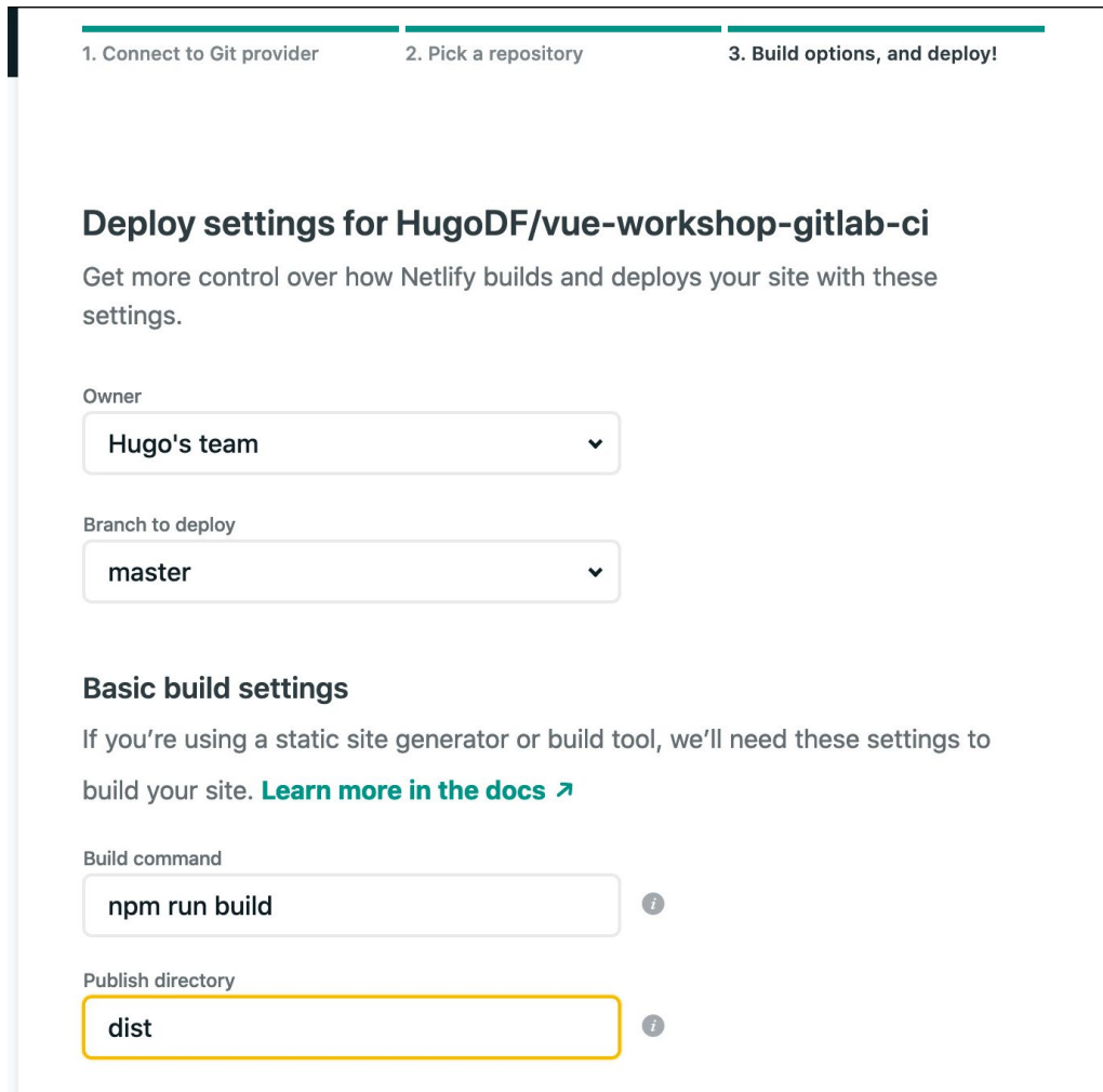
Figure 14.26: The Netlify build configuration tab, filled in with npm run build and dist for the build command and publish directory, respectively
