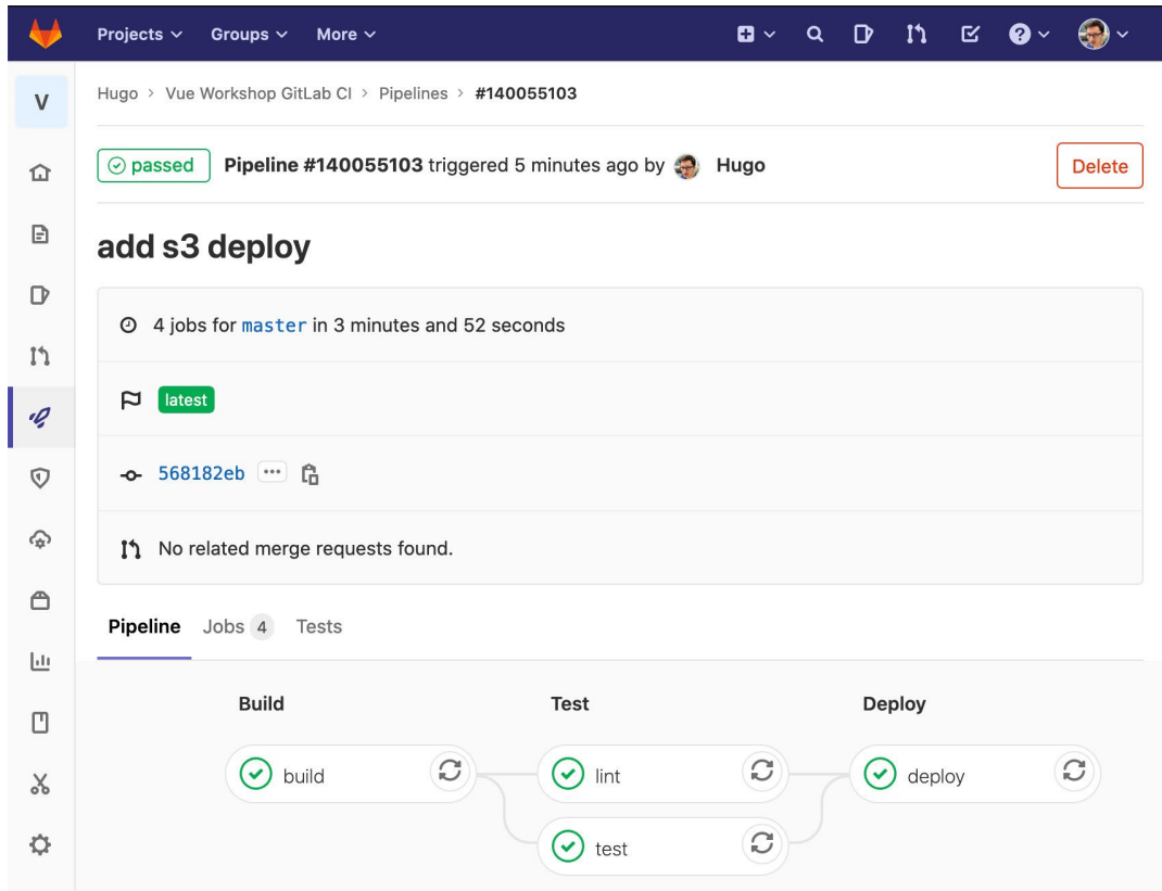
Figure 14.50: Passing build, test, and deploy jobs
