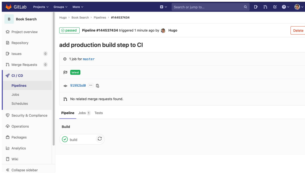
Figure 14.68: The GitLab CI/CD pipeline with the build job passed
