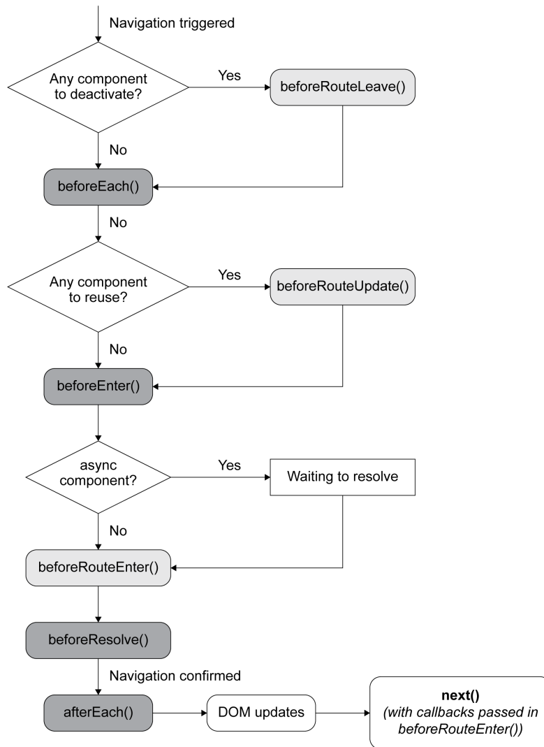
Figure 6.23: Navigation resolution flow diagram
