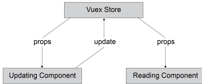
Figure 8.25: Vuex props and state updates hierarchy
