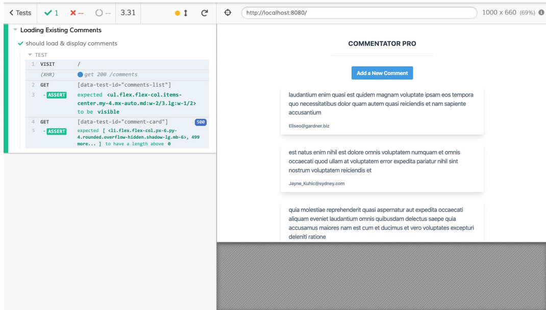
Figure 13.14: Cypress running "load-comments" tests, including a generic load and display test
