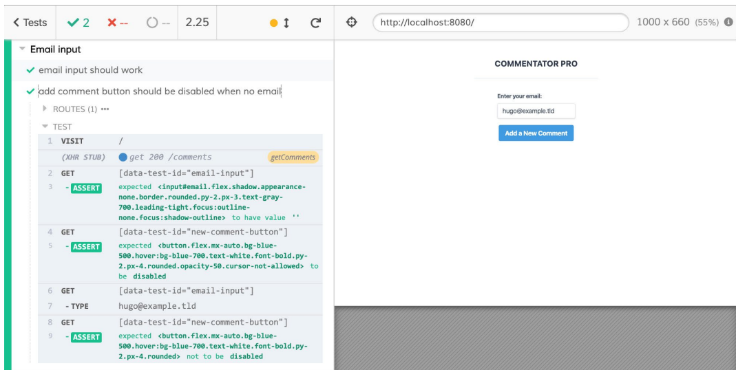
Figure 13.25: Cypress running "enter-email" tests, with the disabled add comment button test
