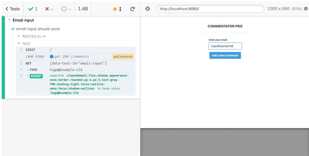
Figure 13.21: Cypress running "enter-email" tests, with the email input test
