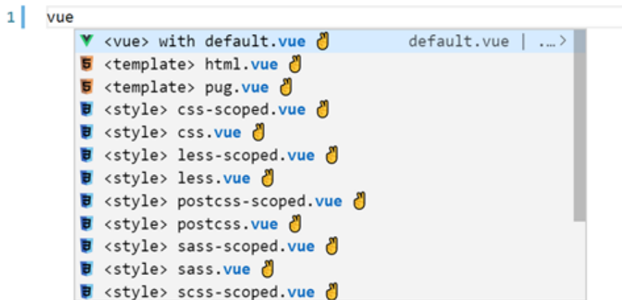
Figure 1.5: VSCode Vetur
