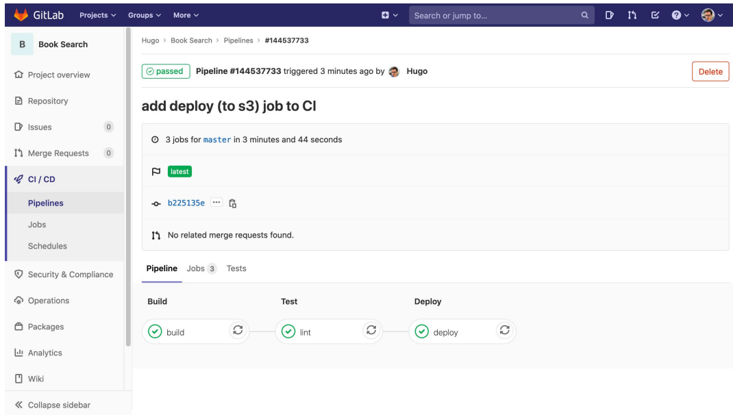
Figure 14.61: The GitLab CI/CD pipeline with the deploy job passed
