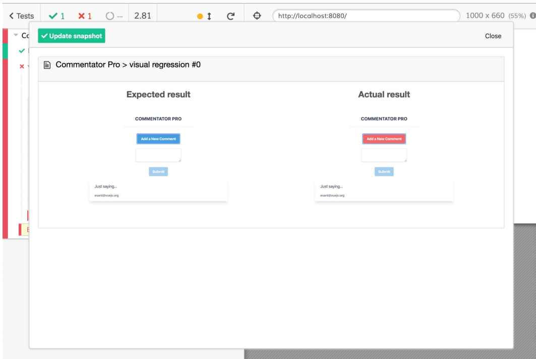
Figure 13.20: Cypress' failing visual regression test diff view
