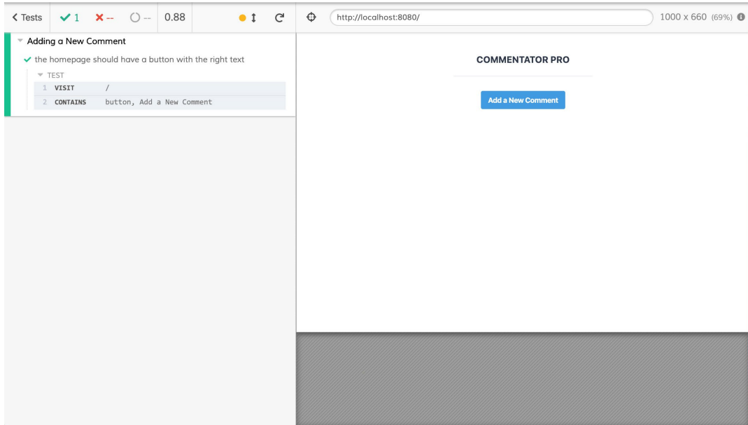
Figure 13.10: Cypress running "add-new-comment" tests, including the new editor text input test
