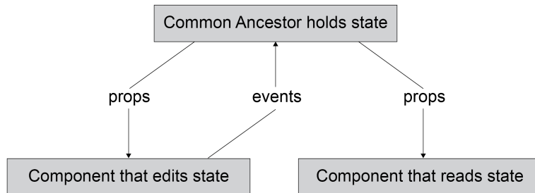
Figure 8.3: Common ancestor component holds state with props and event propagation
