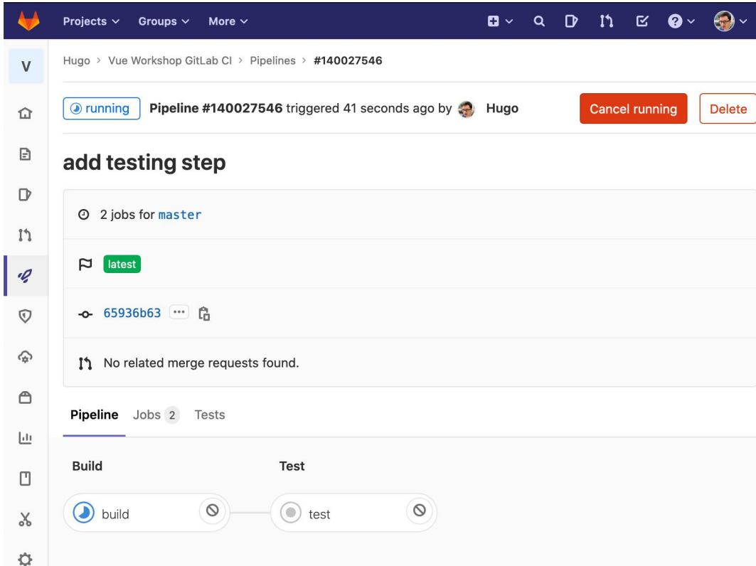
Figure 14.14: GitLab CI/CD pipeline view with a failed build job that stops the test job/stage from running
