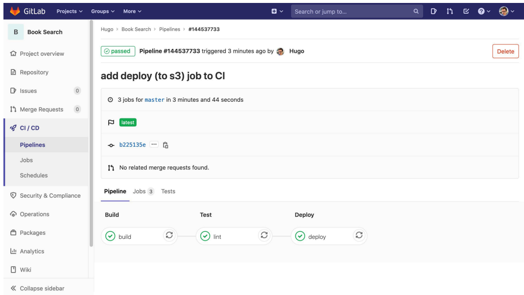
Figure 14.77: The GitLab CI/CD pipeline with the deploy job passed
