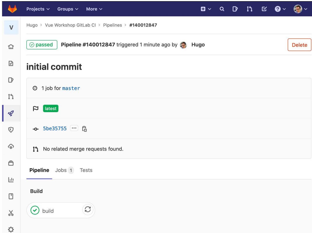
Figure 14.11: GitLab CI pipeline view with the build job passing
