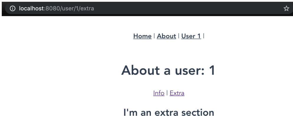
Figure 6.39: User page with nested UserExtra view
