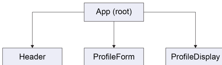
Figure 8.2: Representation of a profile card application component tree
