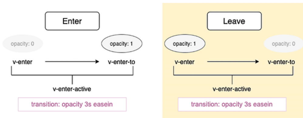
Figure 7.1: Diagram of transition phases
