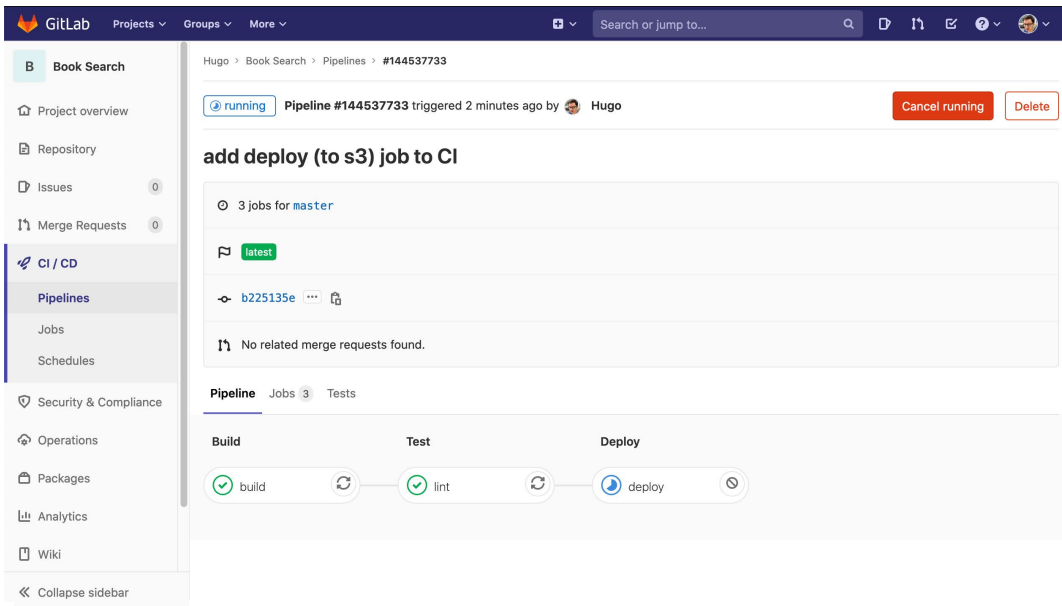
Figure 14.60: The GitLab CI/CD pipeline with the deploy job running
