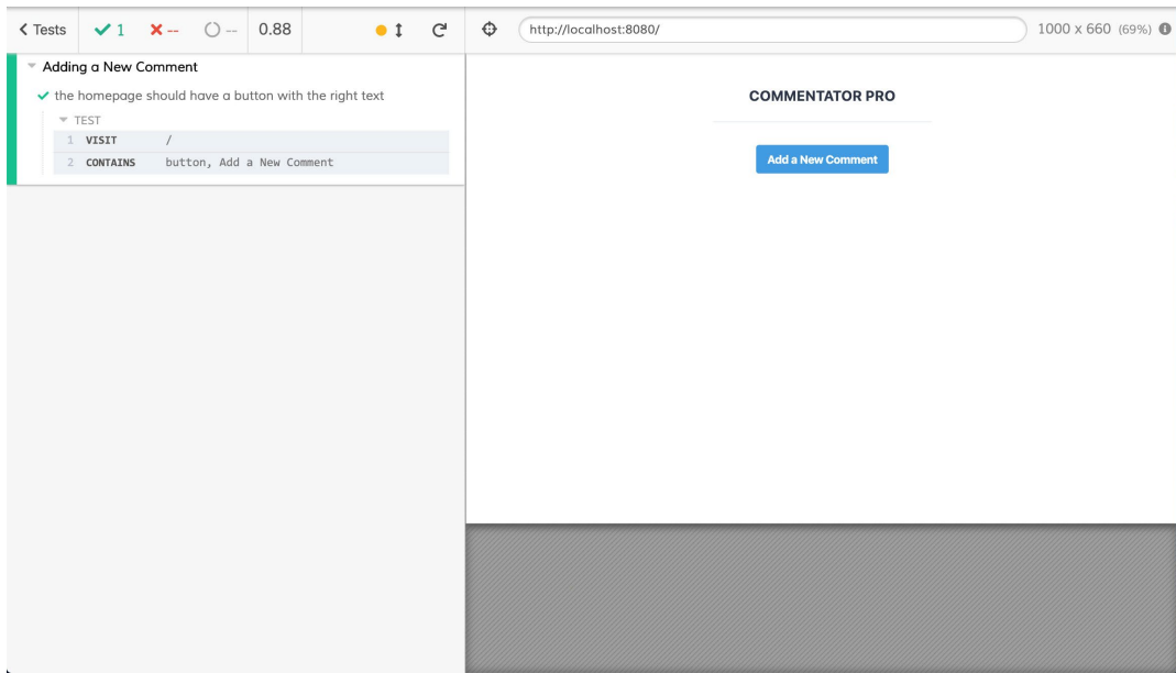
Figure 13.8: Cypress running our "add-new-comment" test in Chrome
