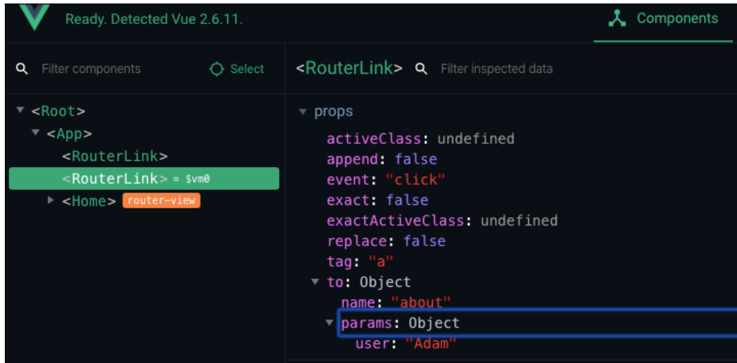
Figure 6.16: The params of the to object in Vue DevTools
