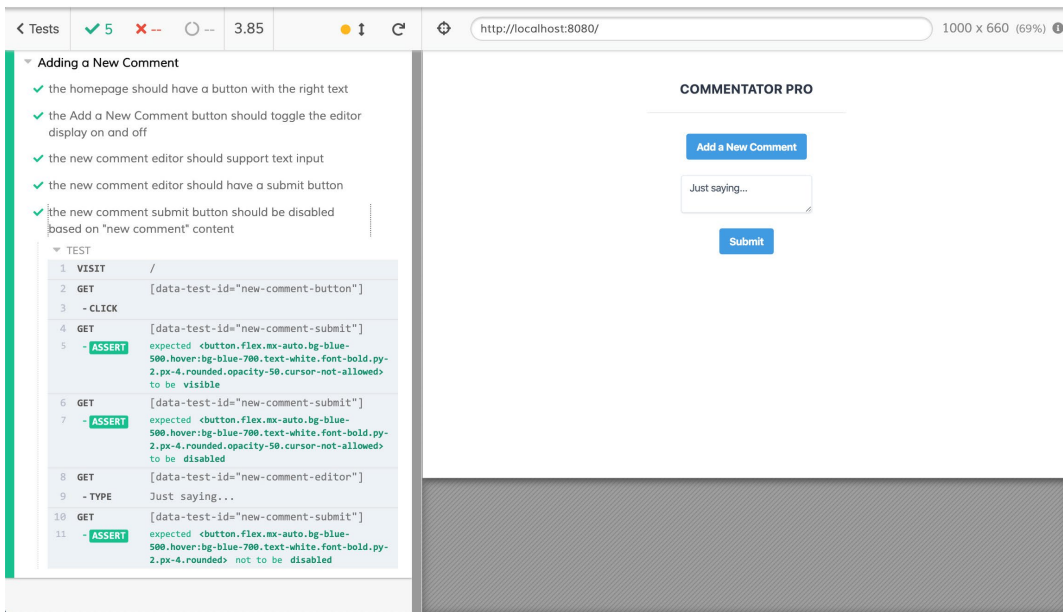
Figure 13.12: Cypress running "add-new-comment" tests, including the new comment submit button disabled test
