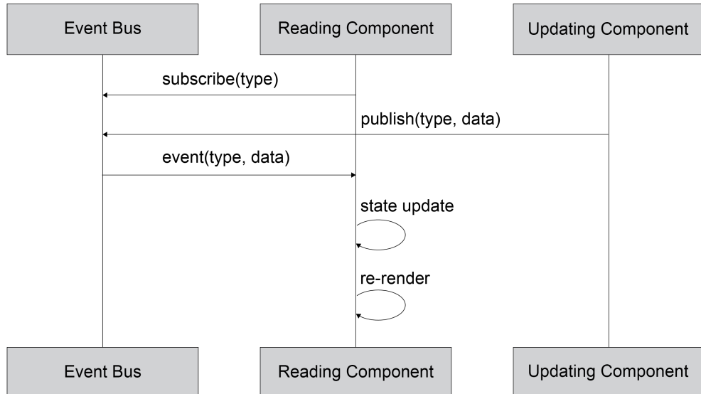
Figure 8.17: Sequence diagram of a reader component and an updating component leveraging an event bus
