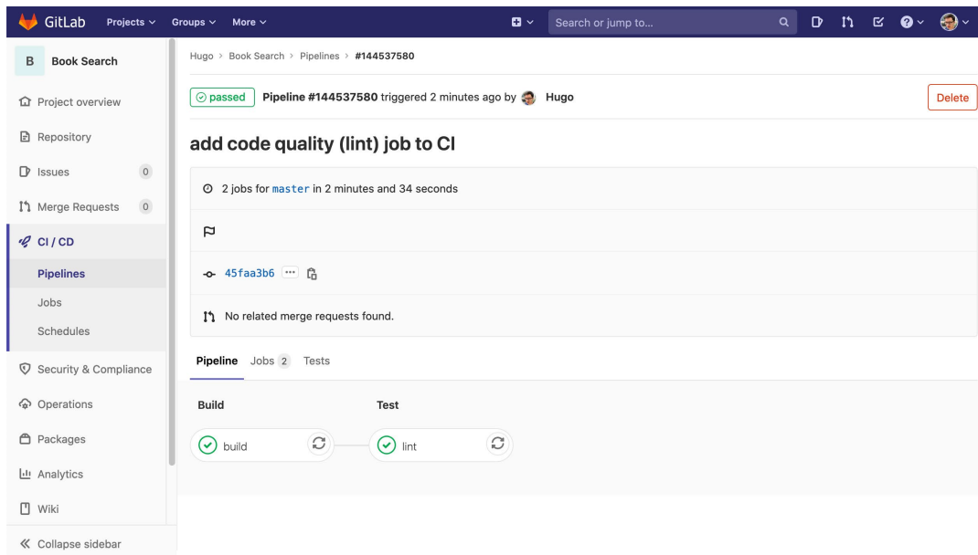
Figure 14.55: GitLab CI/CD pipeline with the lint job passed
