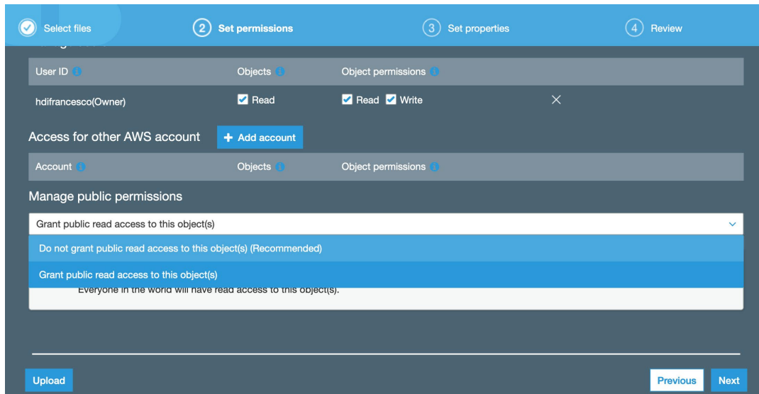
Figure 14.40: Setting file permissions to public on files being uploaded to the S3 bucket
