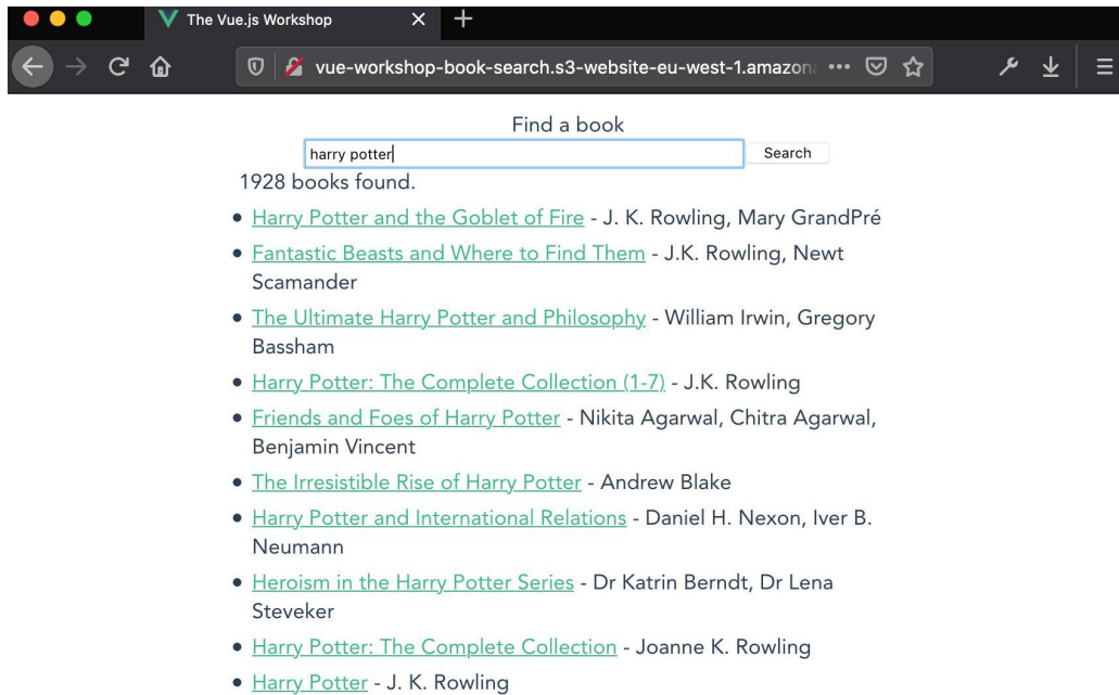
Figure 14.78: Book search accessed through the S3 web endpoint URL
