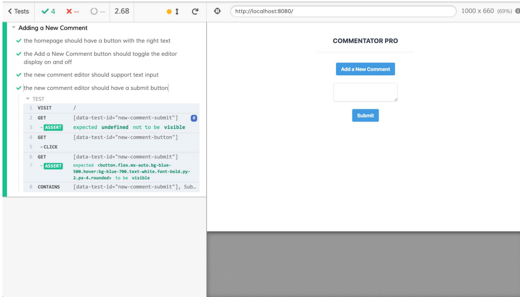
Figure 13.11: Cypress running "add-new-comment" tests, including the new submit button test
