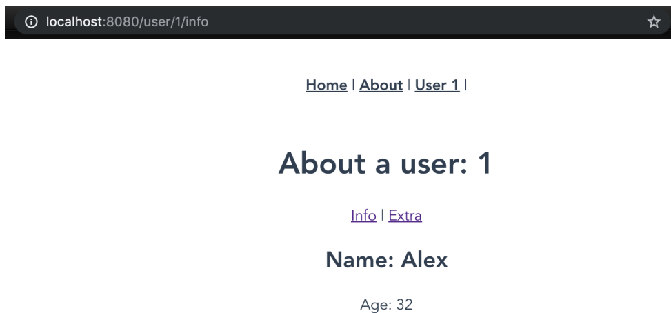
Figure 6.38: User page with nested UserInfo view
