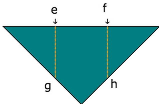
Figure 7-12. Dividing a line into thirds and folding
