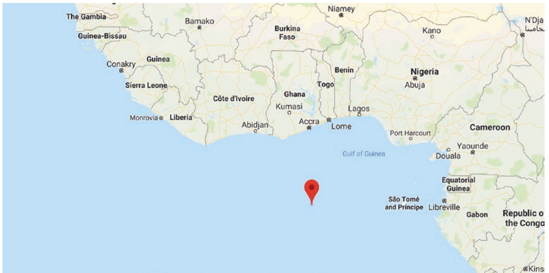
Figure 4-14. The equator at the Greenwich prime meridian
