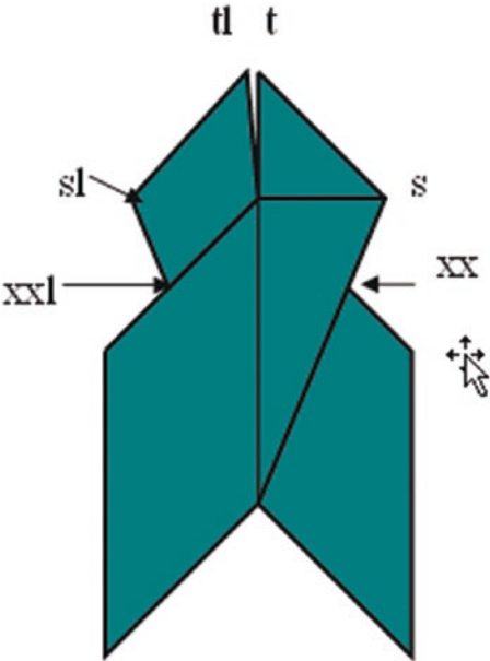
Figure 7-17. After wraparound steps
