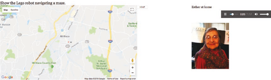
Figure 5-4. Image-and-audio combination
