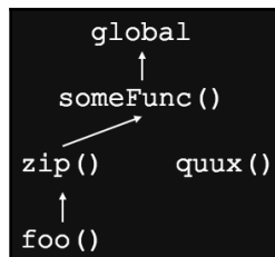
Figure 5.4 – Scope chain
