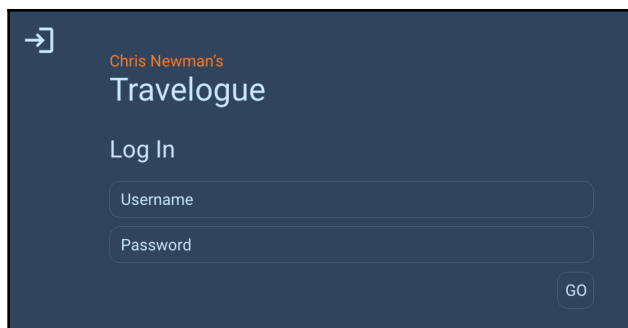
Figure 19.2 – Log In
