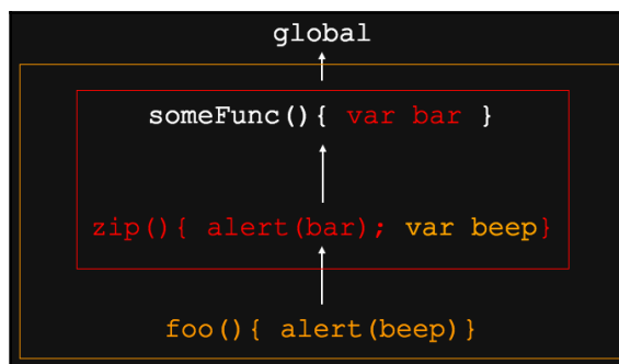
Figure 5.5 – Closures
