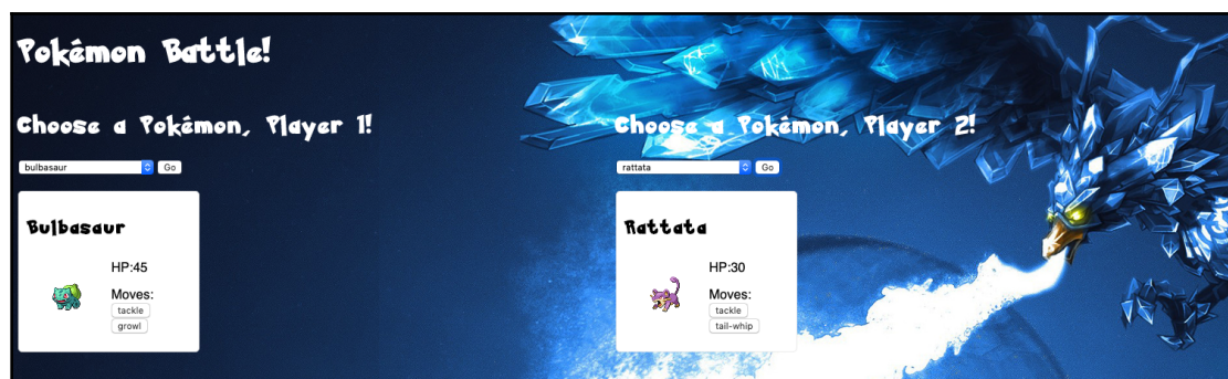
Figure 7.7 – Pokémon game
