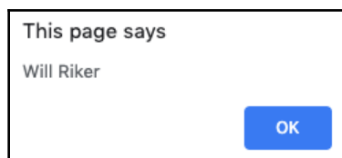
Figure 5.2 – Alert message
