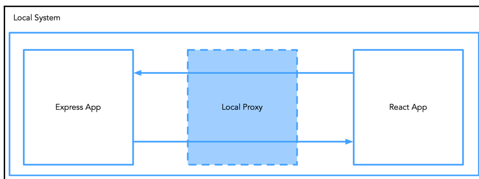
Figure 15.2 - Proxying
