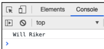
Figure 5.1 – Console output
