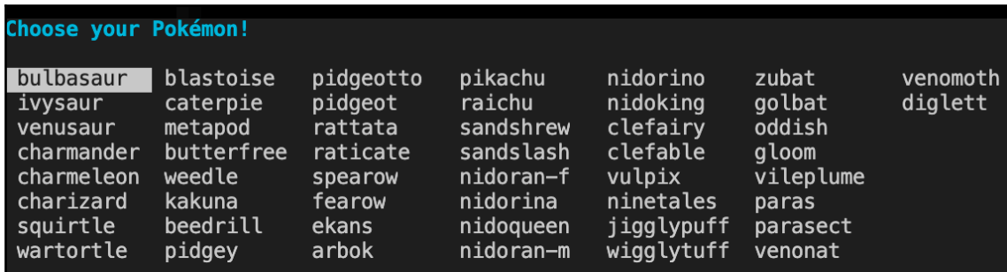
Figure 11.7 - Menu
