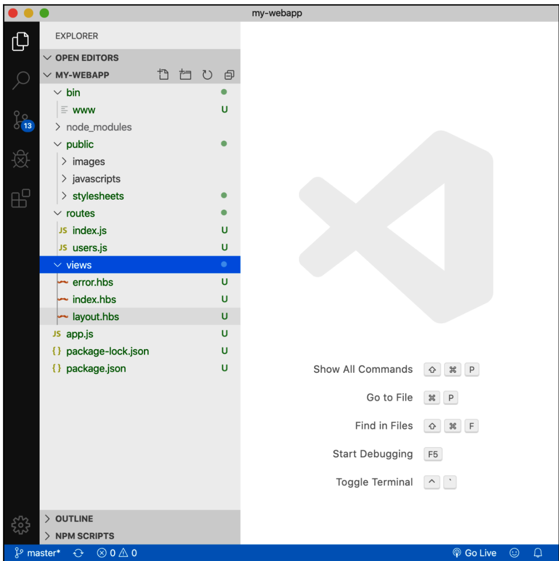
Figure 13.4 - VS Code
