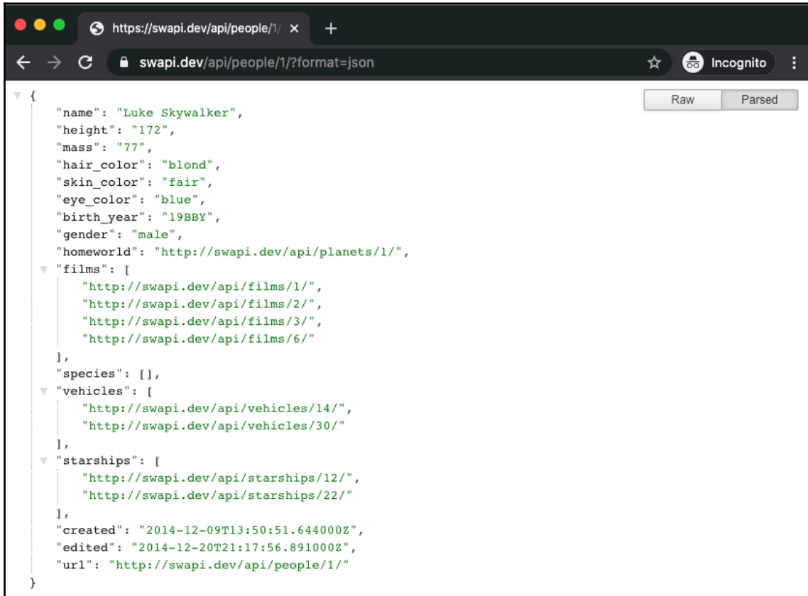
Figure 9.3 - JSON from https://swapi.dev/api/people/1/
