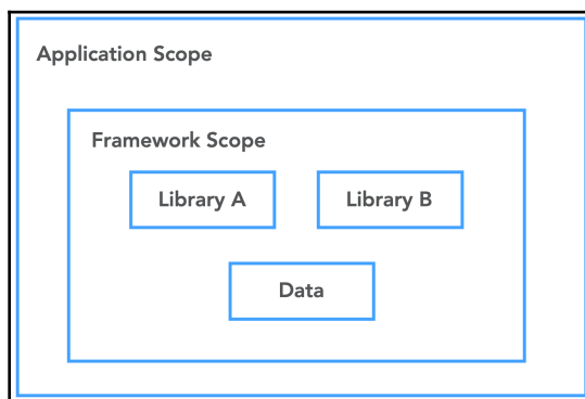
Figure 8.2 – Framework composition
