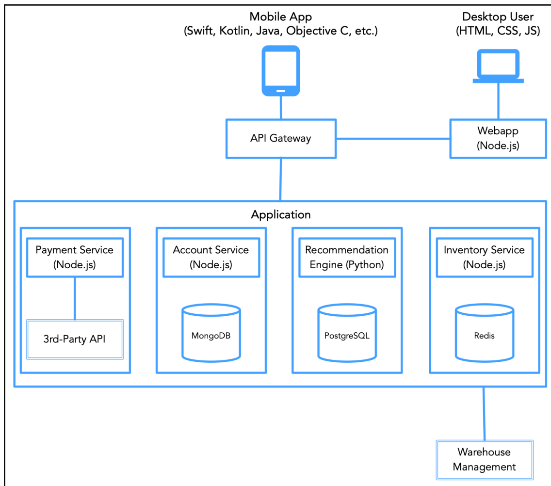
Figure 12.2 – High-level architecture
