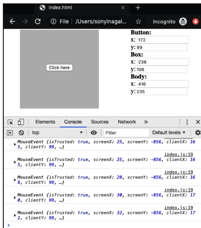
Figure 7.4 – Logging events
