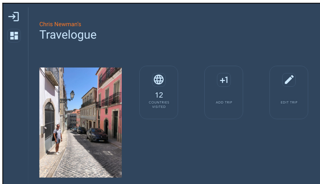
Figure 19.3 – Dashboard
