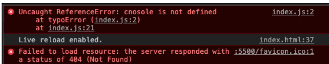
Figure 9.2 - Non-blocking error
