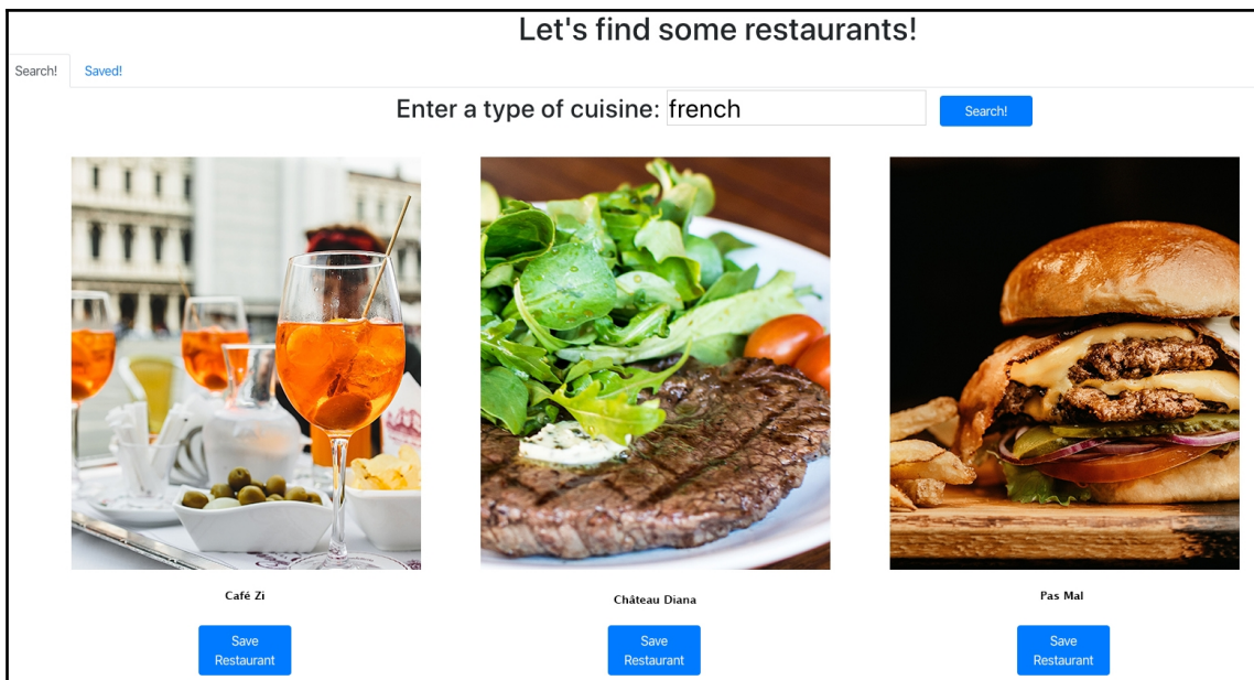
Figure 15.6 - Restaurant finder
