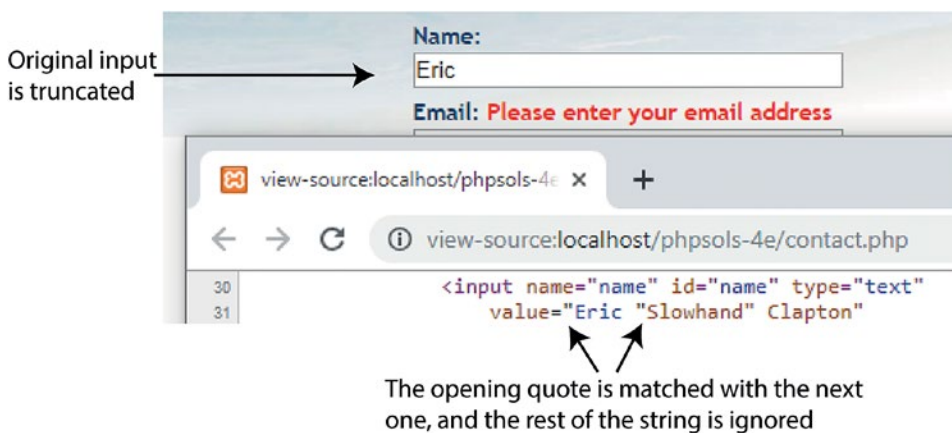
Figure 6-6. Quotes need special treatment before form fields can be redisplayed
