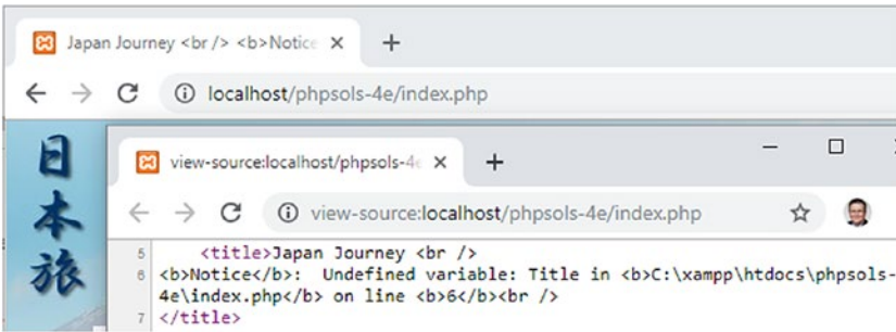
Figure 5-10. Misspelling the variable generates an error notice that appears in the browser tab
