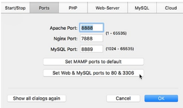
Figure 2-2. Changing the Apache and MySQL ports
