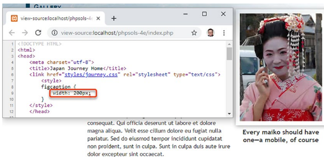
Figure 5-13. The ugly gap is removed by creating a style rule directly related to the image size
