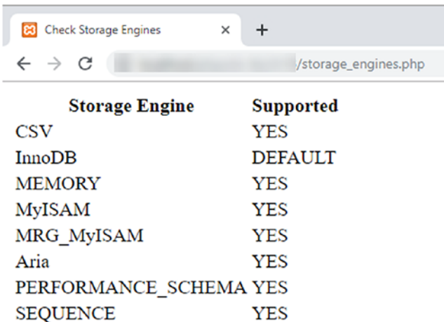
Figure 18-5. The SQL query in storage_engines.php reports which ones are supported
