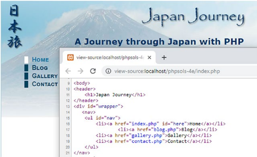
Figure 5-3. There’s no output from the PHP code, so only the HTML is sent to the browser
