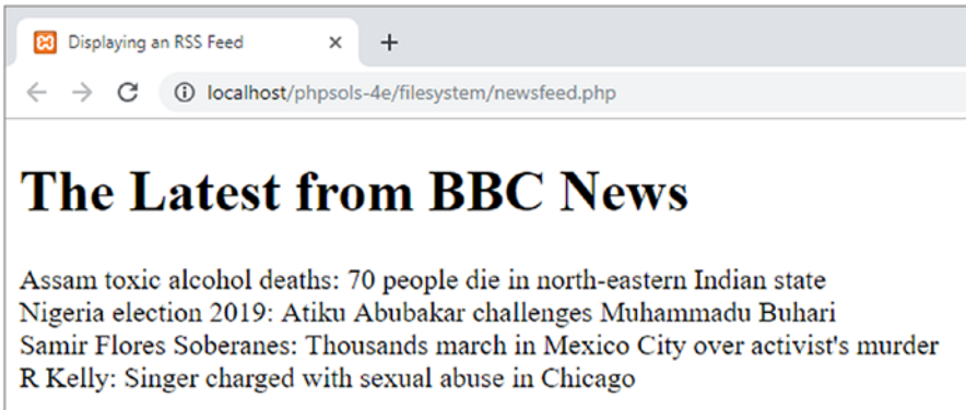
Figure 7-5. The LimitIterator restricts the number of items displayed
