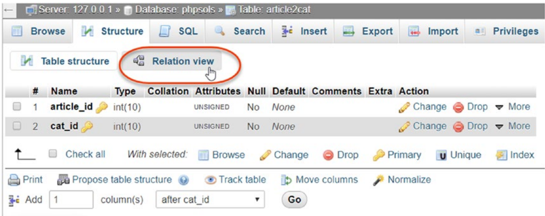
Figure 18-12. Foreign-key constraints are defined in phpMyAdmin’s Relation view
