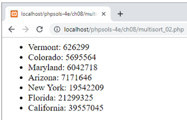
Figure 8-4. The population numbers are now in ascending order, keeping the correct state names with them
