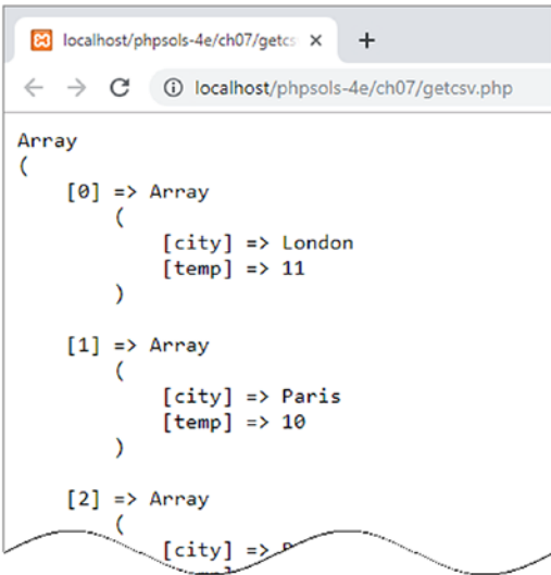
Figure 7-1. The CSV data has been converted into a multidimensional associative array
