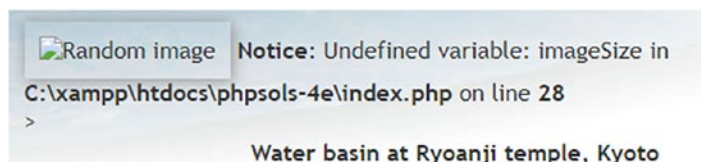
Figure 5-14. An error in an include file can destroy the look of your page
