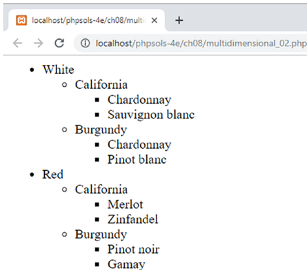
Figure 8-7. ListBuilder extends RecursiveIteratorIterator to automate building nested lists from a multidimensional associative array
