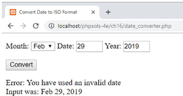
Figure 16-8. The convertDateToISO() function rejects invalid dates
