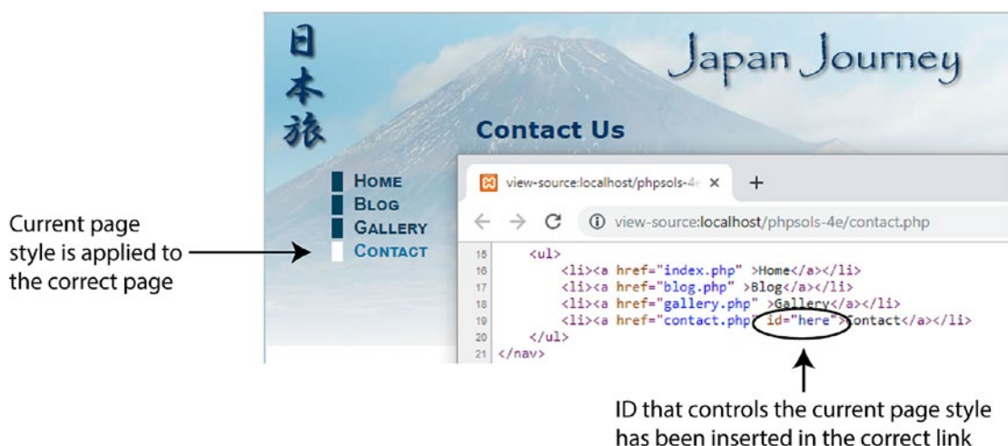
Figure 5-5. Conditional code in the include file produces different output for each page
