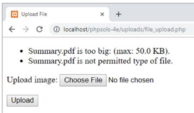
Figure 9-5. The class now reports errors with invalid size and MIME types
