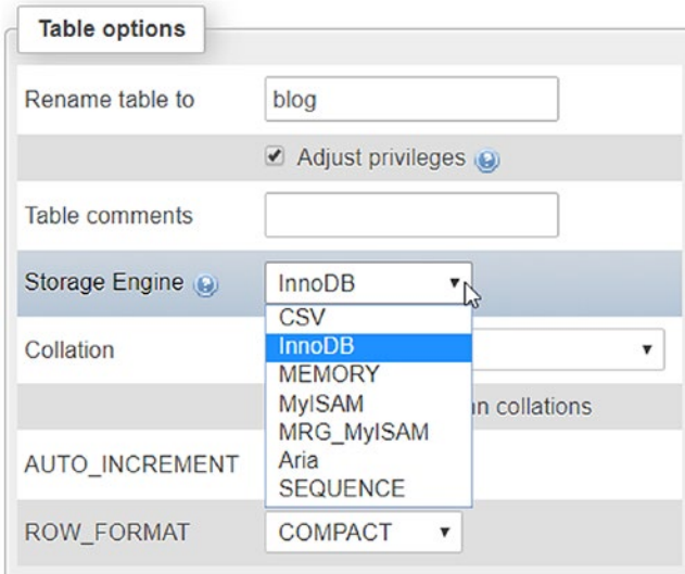
Figure 18-4. The available storage engines are listed in the Table options
