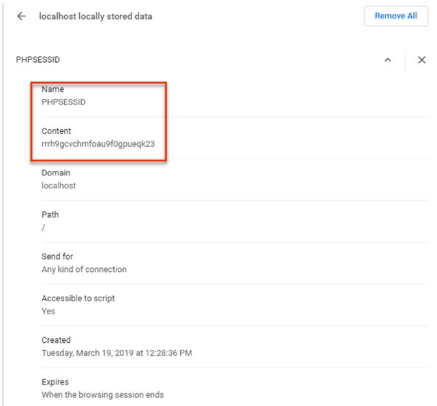
Figure 11-1. PHP sessions store a unique identifier as a cookie in the browser
