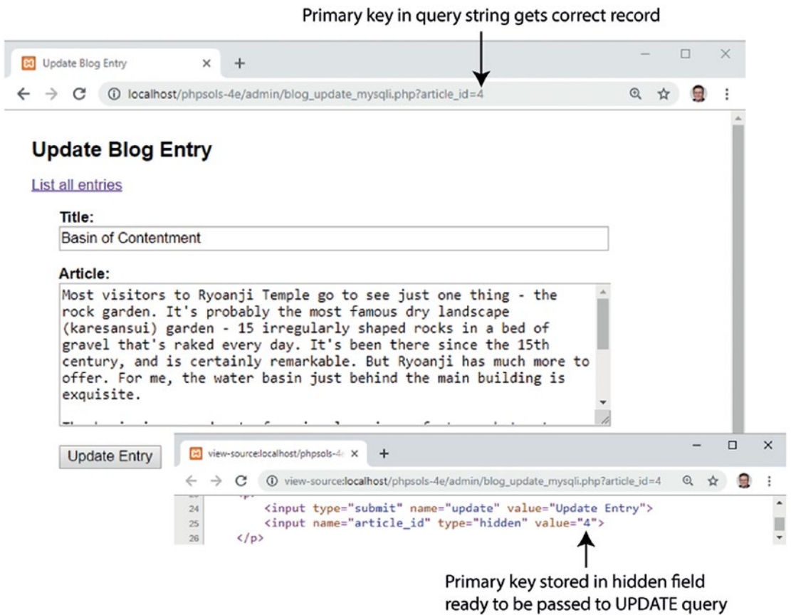
Figure 15-3. The primary key keeps track of a record during the update process
