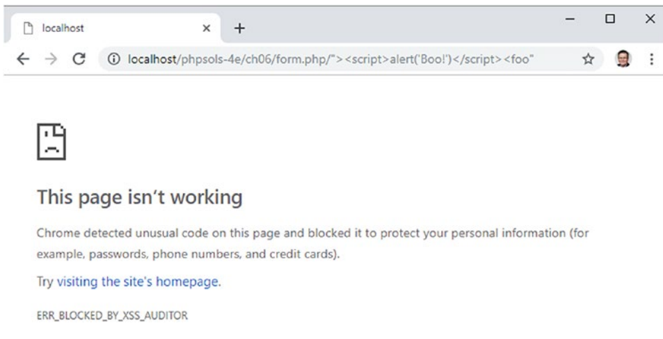
Figure 6-3. Google Chrome automatically blocks suspected XSS attacks
