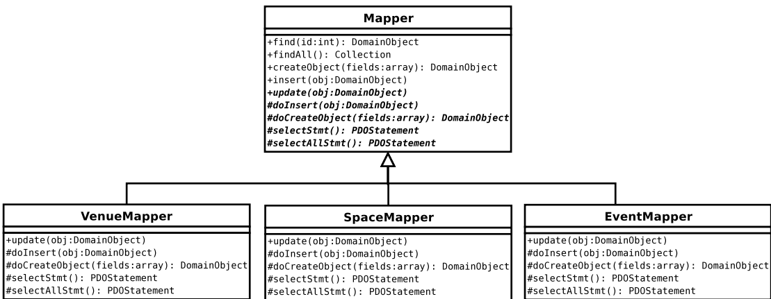
Figure 13-1. Mapper classes
