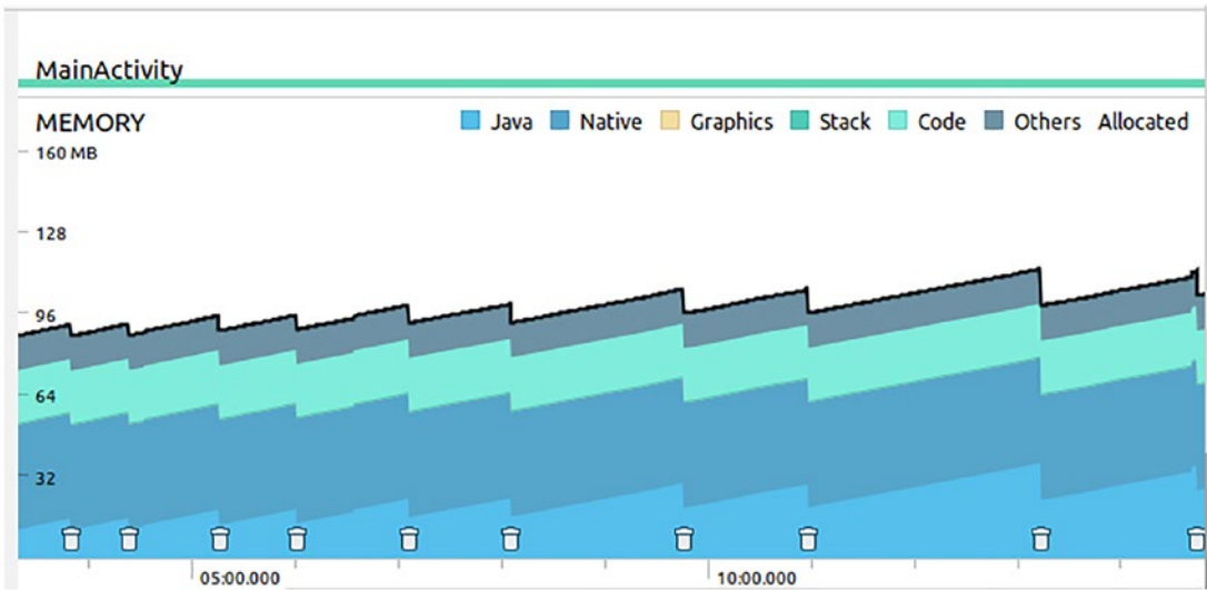
Figure 16-5. Memory Profiling, Longer Period
