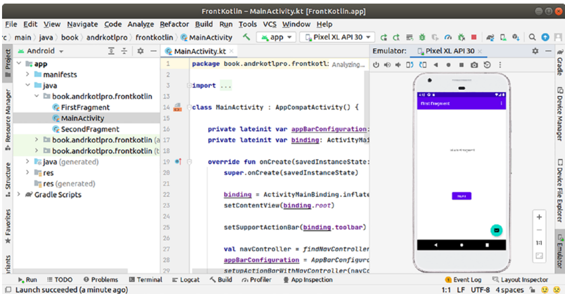
Figure 1-2. Android Studio
