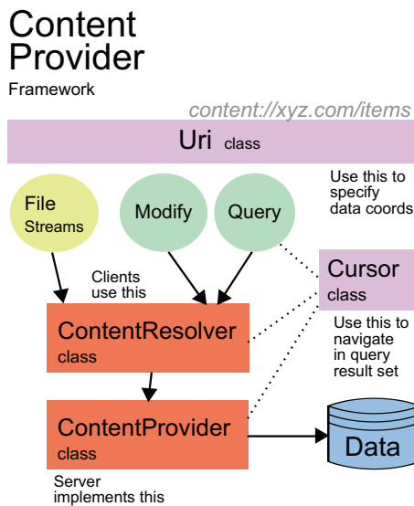
Figure 6-1. Content Provider Framework
