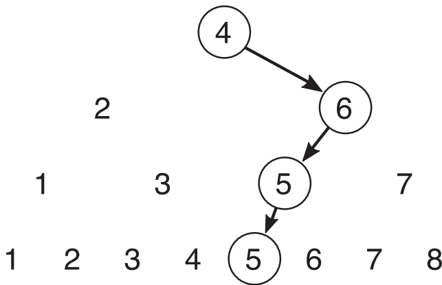
Figure 9-1. A binary search to find the number 5
