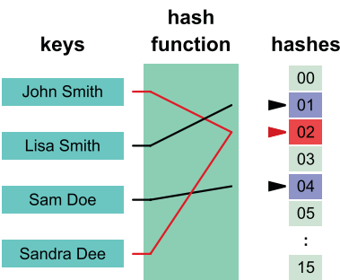
Figure 16-4. Description of different hash functions. Images were created by Jorge Stolfi and are in the public domain
