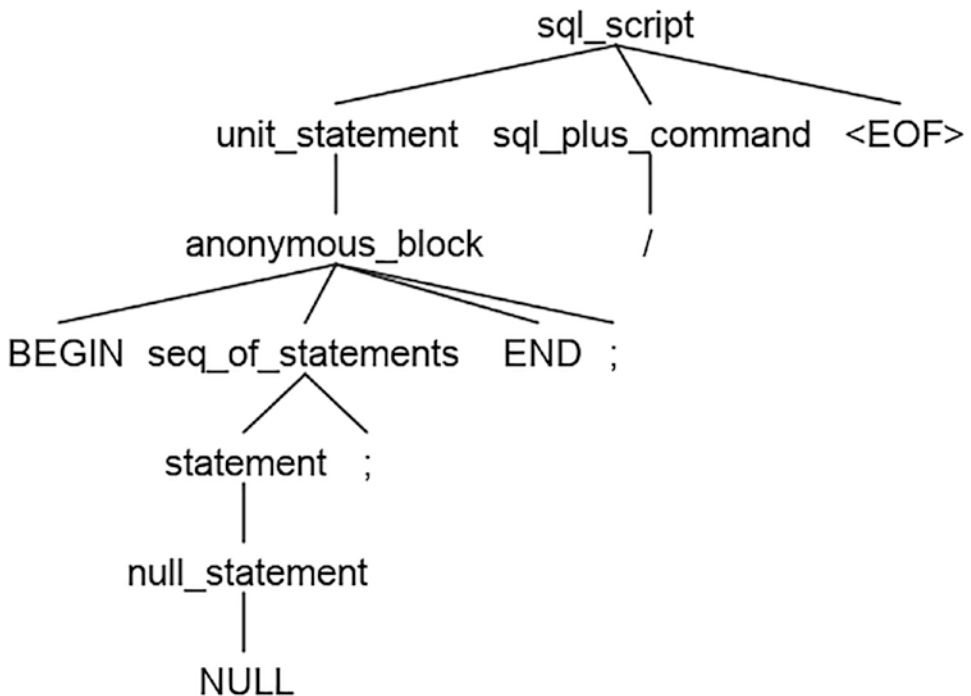
Figure 20-1. ANTLR parse tree for a simple PL/SQL program
