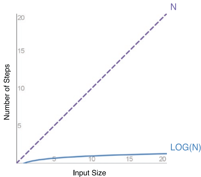
Figure 16-6. Compare O(\log(N)) index read vs. O(N) full table scan
