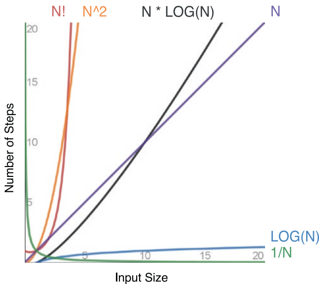
Figure 16-2. Functions that represent important Oracle operations
