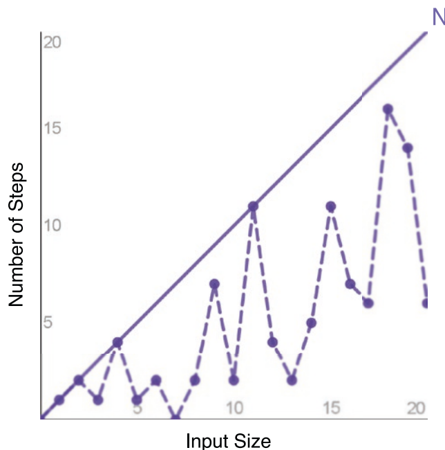
Figure 16-1. Number of steps vs. input size for linear search algorithm, including an asymptote
