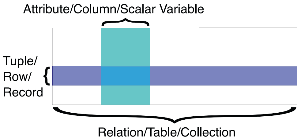
Figure 21-1. Relational, SQL, and PL/SQL terminology for similar concepts. Based on an image created by Chris Martin and is in the public domain
