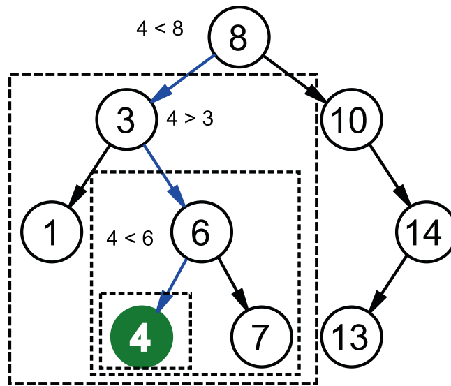
Figure 16-5. Binary search algorithm. Image was created by Chris Martin and is in the public domain
