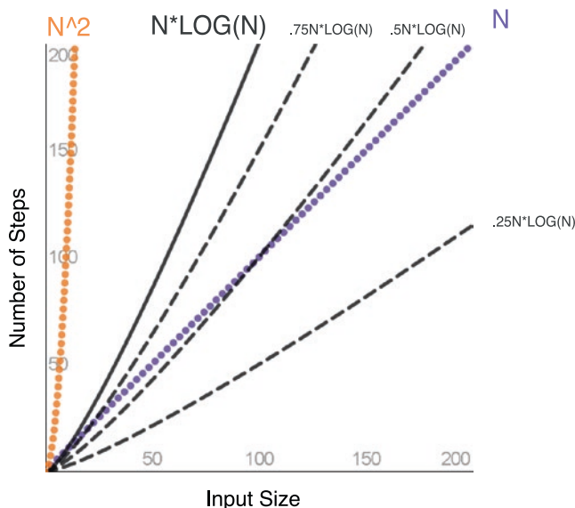
Figure 16-9. Comparing N^2 , N \cdot \log(N) , and N
