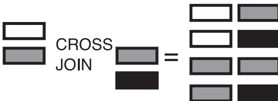
Figure 1-2. Visualizing joins with join diagrams and Venn diagrams
