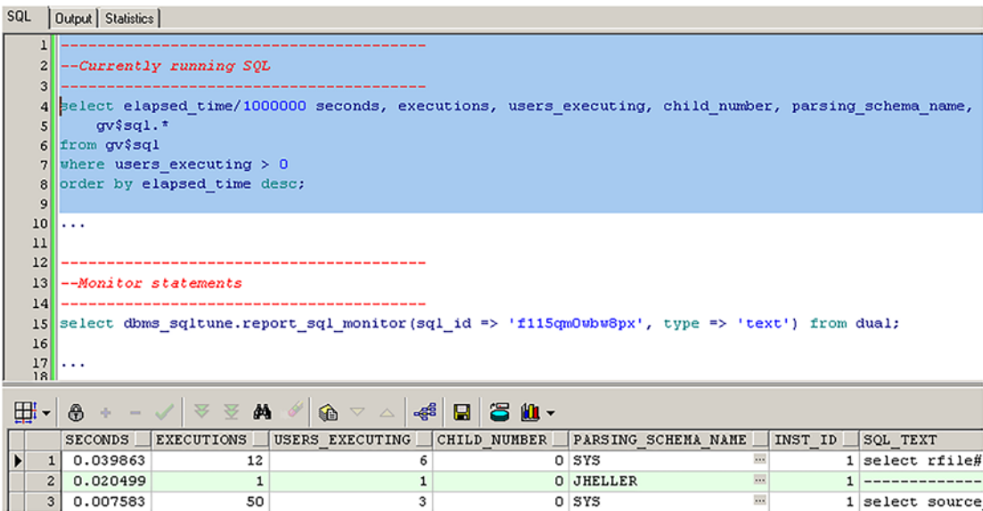
Figure 5-5. Example of a SQL performance worksheet
