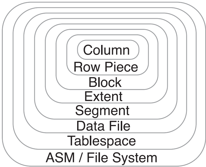
Figure 10-1. Storage structure hierarchy
