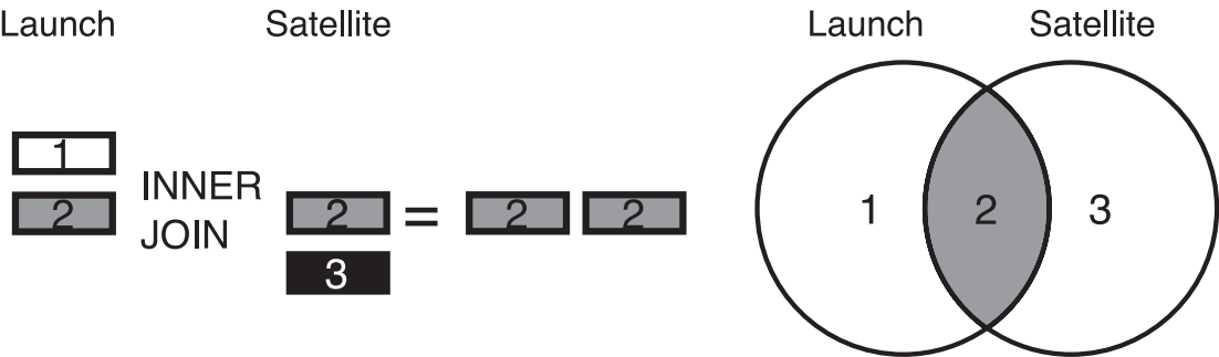
Figure 1-3. Visualizing joins with join diagrams and Venn diagrams, drilling down into INNER JOIN and showing values
