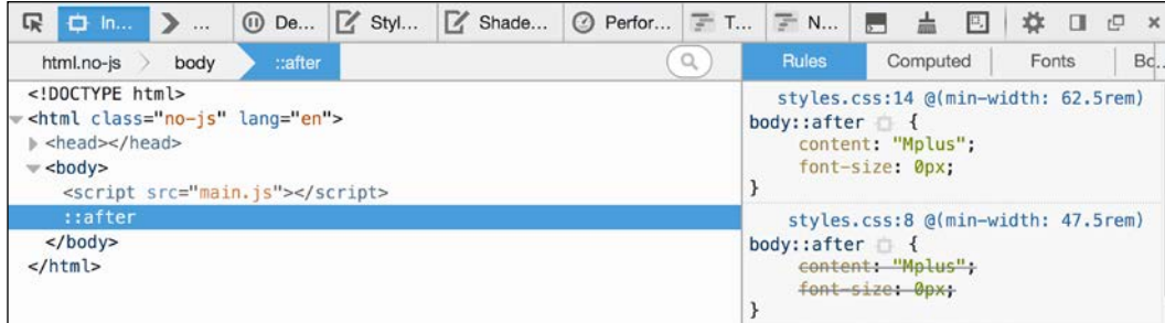
Figure 11.7: We can use pseudo-elements to communicate to JavaScript
