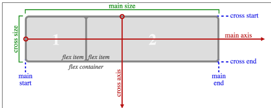
Figure 4.6: This image from the specification shows that the main axis always relates to the direction the flex container is heading
