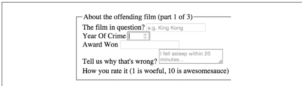
Figure 10.8: On desktop browsers, "spinners" are shown for number inputs
