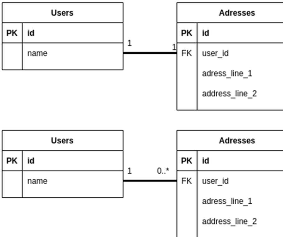
Figure 9-7. ERD
