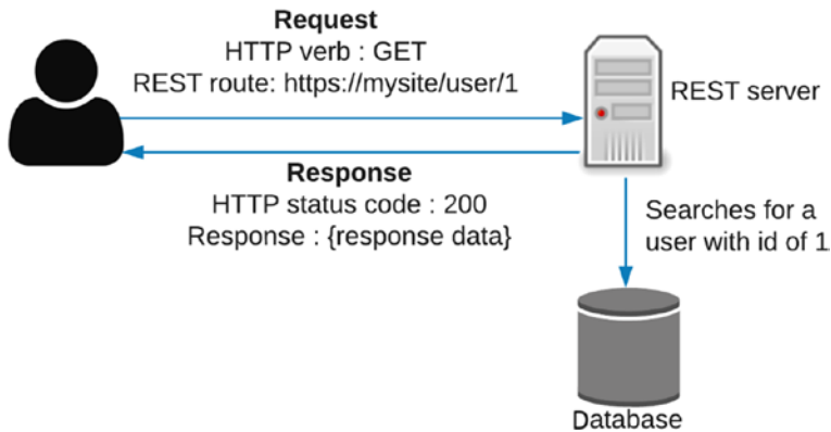
Figure 7-1. Request/response relationship
