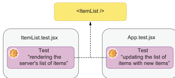
Figure 8.3 The tests that break if you decide to change the format of the text rendered by ItemList
