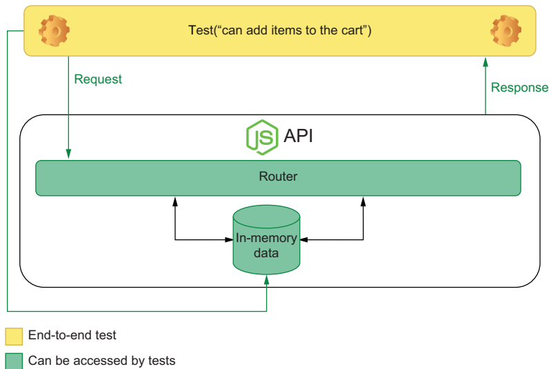
Figure 4.3 What's been exposed to the test for addItemToCart
