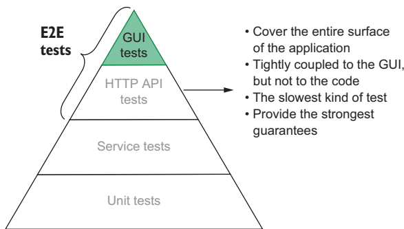
Figure 2.13 GUI tests' placement in the testing pyramid
