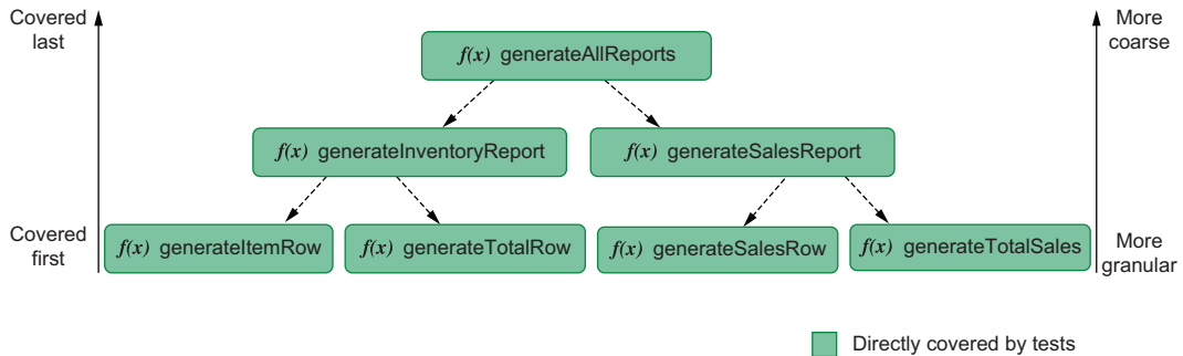
Figure 9.7 Taking a bottom-up approach to testing means covering granular individual functions first and then moving up toward more coarse pieces of software.
