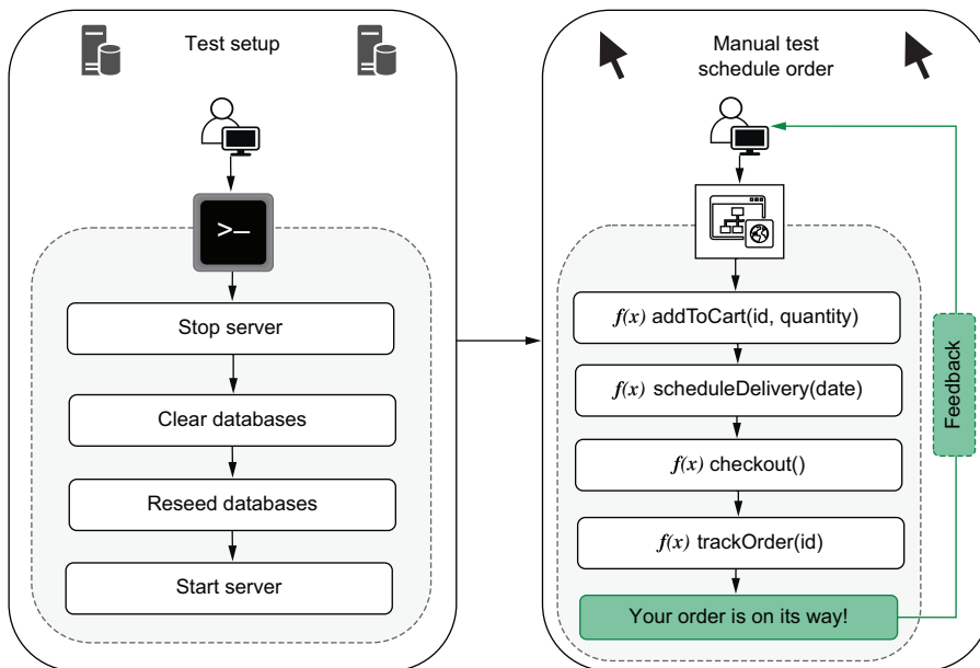
Figure 1.6 The steps to test tracking an order
