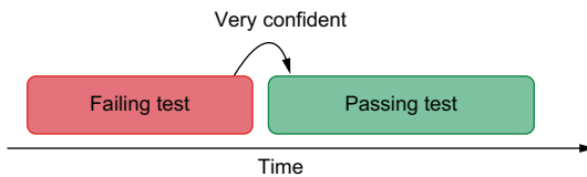
Figure 9.4 If you feel very confident that you know how to implement a particular piece of code, you can write a full-blown test and the final implementation straightaway.
