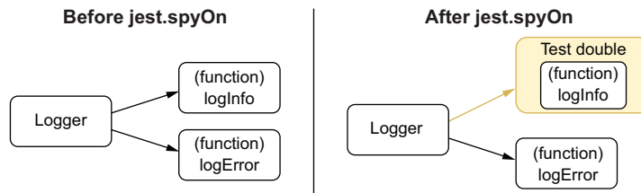
Figure 3.11 What happens when using spyOn
