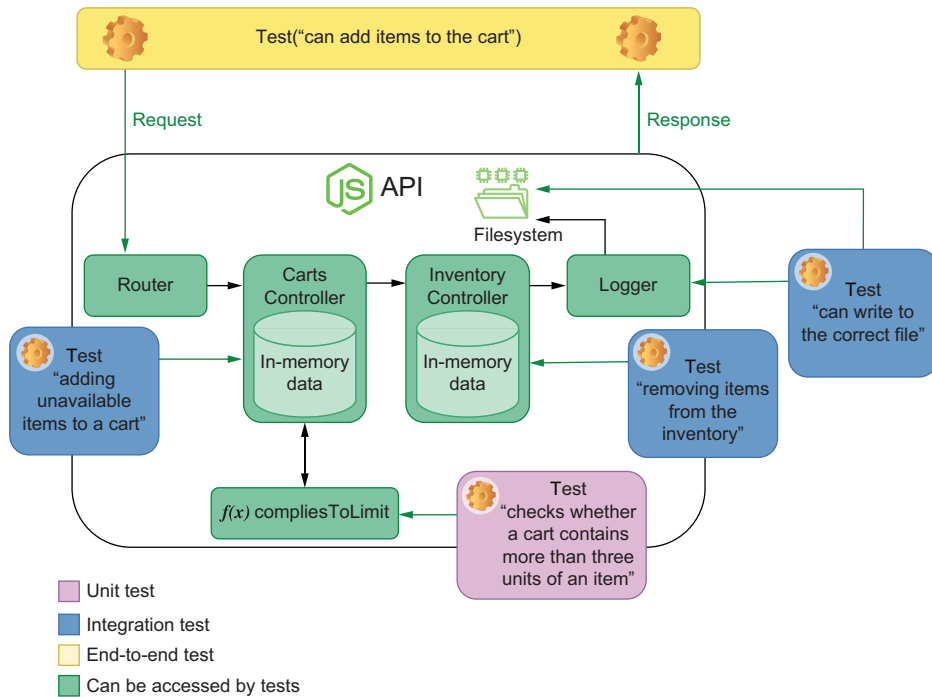
Figure 4.6 Integration tests will have access to all the dependencies with which your application interacts.
