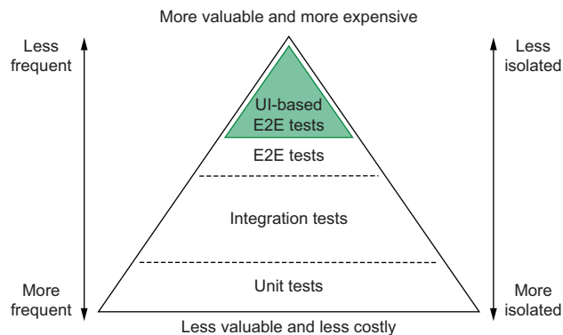
Figure 10.3 Within the end-to-end tests section of the testing pyramid, UI-based end-to-end tests go at the very top.
