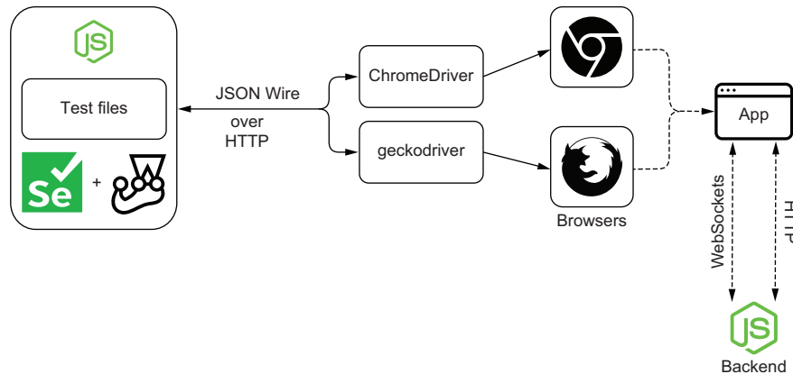
Figure 10.7 If you want to use Selenium for testing, you must pair it with a testing framework, such as Jest.
