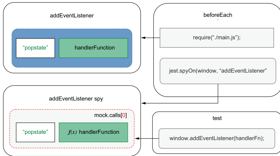
Figure 6.8 Your spy should capture the calls that happen only after executing main.js .
