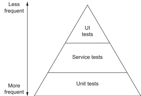
Figure 2.1 Mike Cohn's test pyramid
