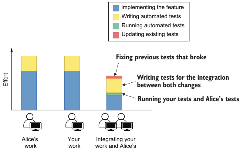
Figure 1.11 The effort necessary to verify changes in each stage of the development process when automated tests exist
