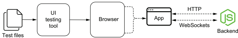
Figure 10.1 An end-to-end test for the entire application covers all parts of its stack by interacting with it through a browser.
