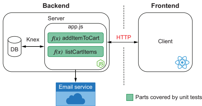
Figure 2.4 Unit tests' scope
