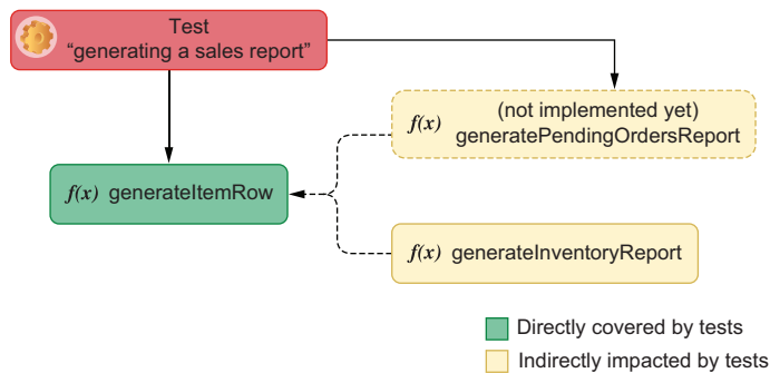
Figure 9.15 To avoid adding a new function and extra tests for it, you can update the generateItemRow function's tests and reuse them in multiple places.
