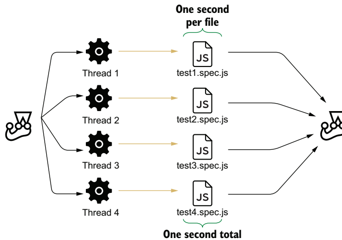
Figure 3.6 What happens when running tests in parallel
