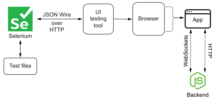
Figure 10.5 Selenium sends HTTP requests to the Webdrivers that control browsers. These requests adopt the JSON Wire protocol.
