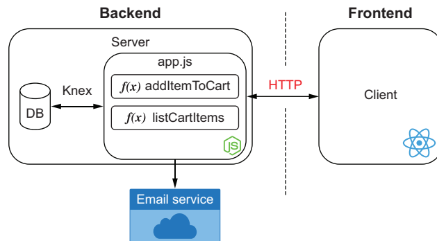
Figure 2.3 The bakery's website infrastructure
