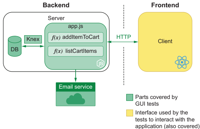
Figure 2.12 GUI tests' scope
