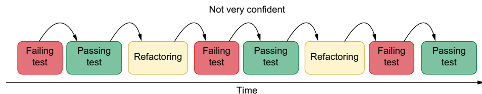
Figure 9.2 The less confident you feel, the smaller your steps should be, and the more times you'll go through the test-driven development cycle.
