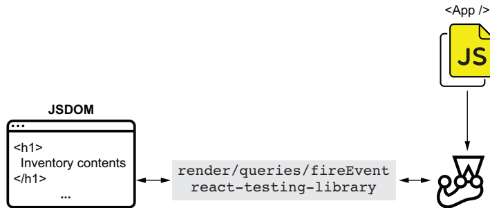
Figure 7.5 How your tests interact with your components when you use onlyreact-testing-library . This library is capable of rendering components, finding elements, and interacting with them.
