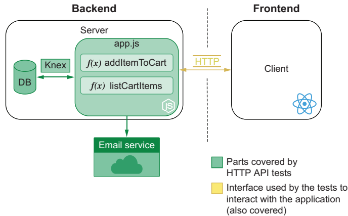
Figure 2.10 The scope of tests that address your backend through its HTTP API
