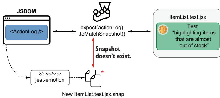
Figure 8.10 The serializer included in jest-emotion causes Jest to write snapshots that include actual CSS rules instead of cryptic class names.
