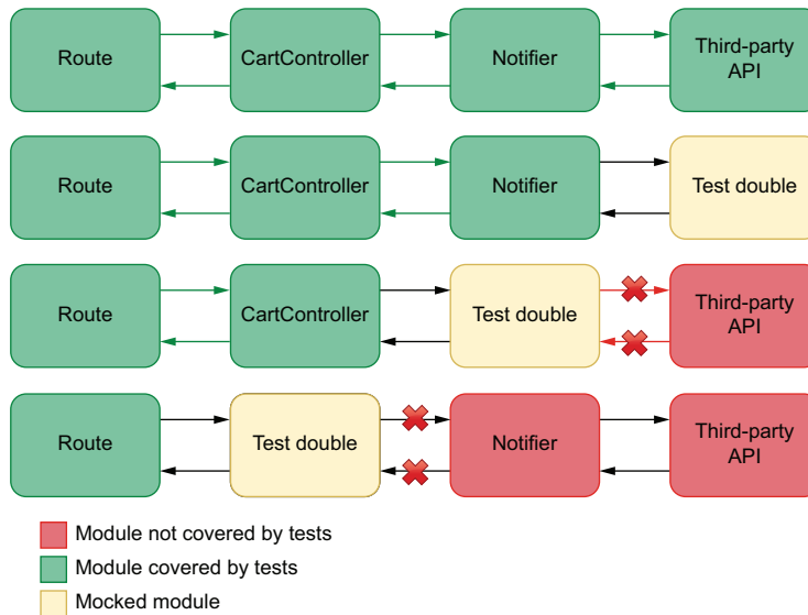
Figure 3.13 How much complexity is hidden by mocking each layer of your application
