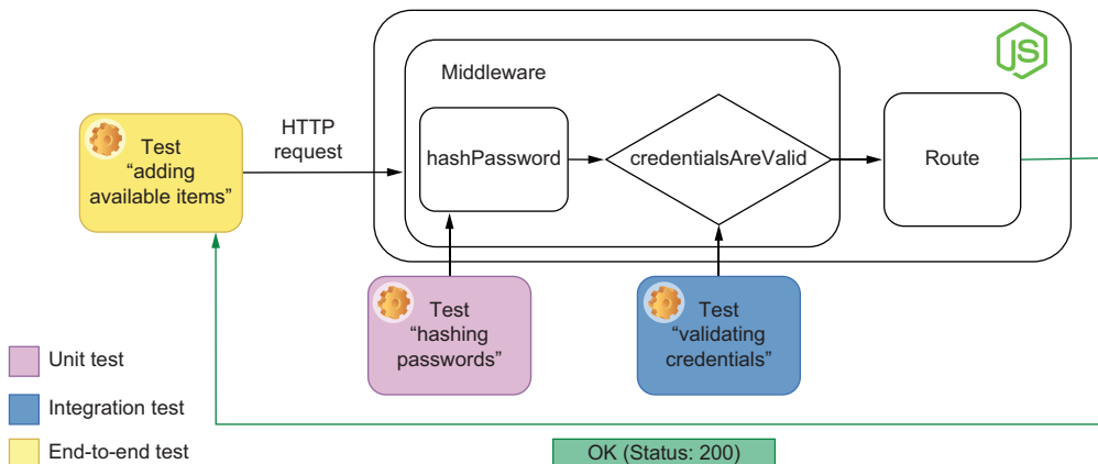
Figure 4.11 The part of the middleware with which this integration test interacts
