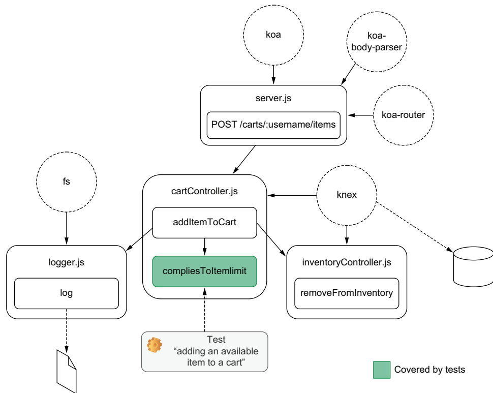
Figure 5.5 A unit-test for compliesToItemLimit covers only that function.
