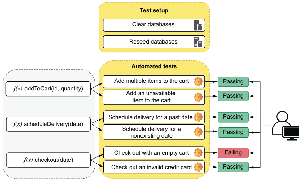
Figure 1.8 Automated tests can check parts of your code individually and give you precise feedback on what's broken as soon as you break it.
