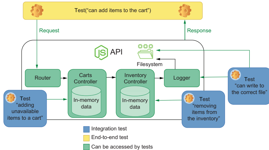
Figure 4.5 Integration tests will have access to all the dependencies with which your application interacts.
