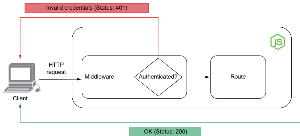
Figure 4.8 The role of authentication middleware
