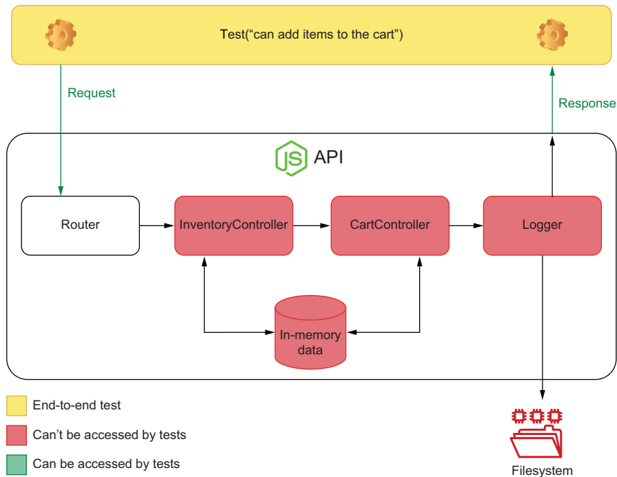
Figure 4.1 What tests can access if an application isn't designed with testing in mind
