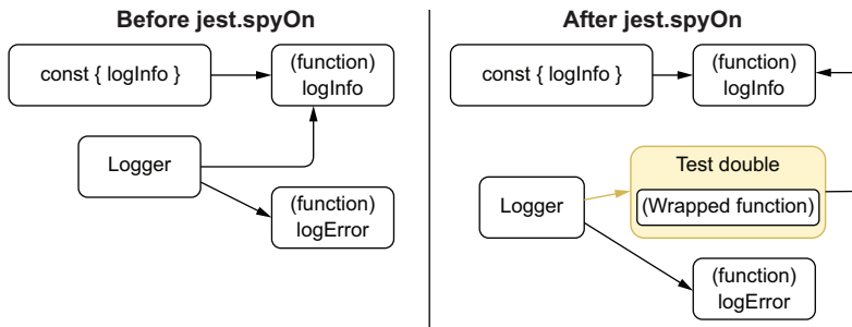
Figure 3.12 What happens when using spyOn when you have direct references
