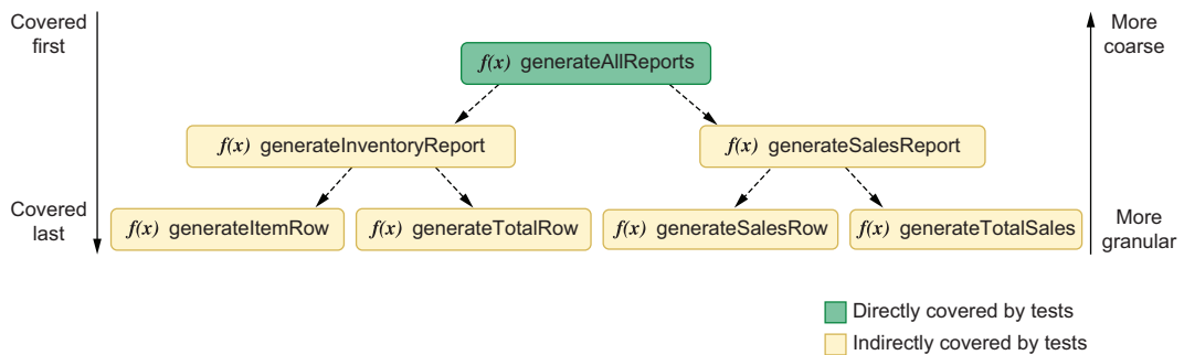
Figure 9.9 Testing the topmost function indirectly attests to the quality of its dependencies.
