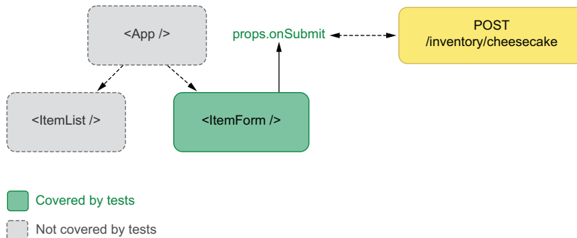
Figure 8.1 This test for ItemForm can validate only the component itself. It can’t check whether its parent or sibling components give it the correct props or that they update adequately.
