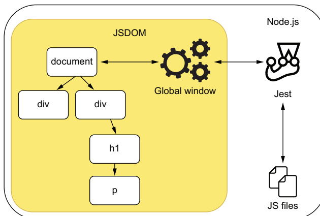
Figure 6.2 The JavaScript environment within Node.js
