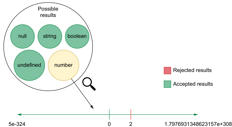
Figure 3.10 The range of results accepted by a negated assertion
