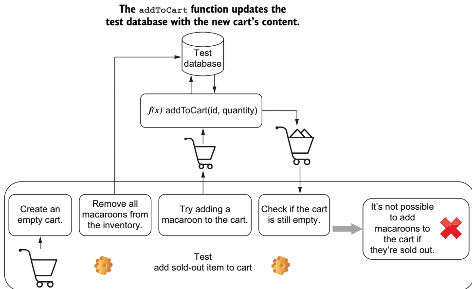
Figure 1.5 The necessary steps for a test to check whether we can add sold-out items to the cart
