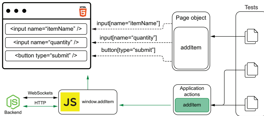
Figure 11.9 Application actions directly invoke the functions your application has attached to the global window.
