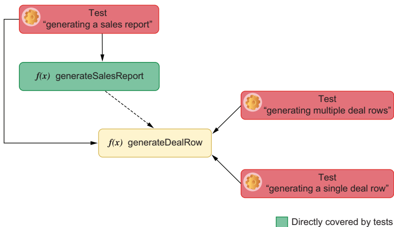
Figure 9.17 When performing test-driven development, you added tests that target the generateDealRow function itself. Because you also implemented a test for the topmost generateSalesReport , the tests for generateDealRow ended up being redundant.
