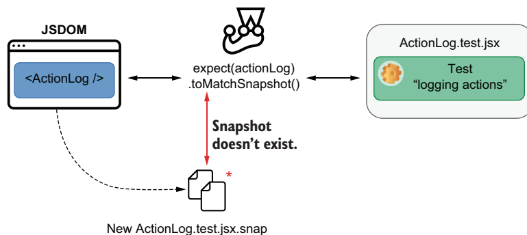
Figure 8.6 When Jest can't find a snapshot for a test, it creates one using the content of the assertion's target.
