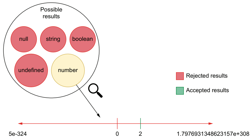
Figure 3.9 The range of results accepted by the tight toBe assertion
