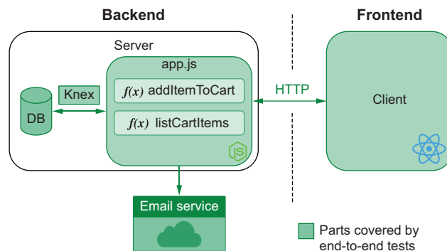
Figure 2.8 End-to-end tests' scope
