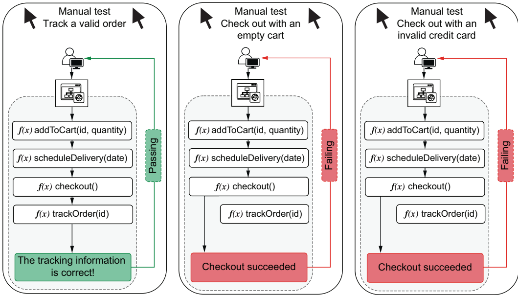
Figure 1.9 The steps that must be followed when testing each feature
