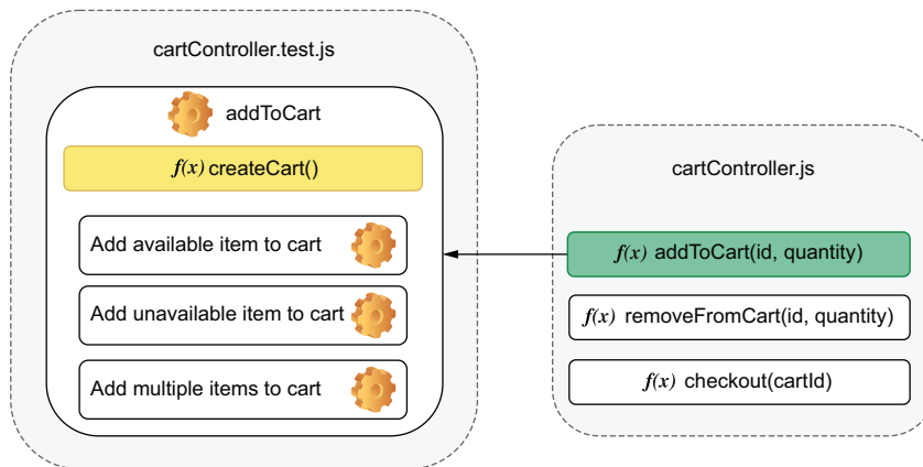
Figure 3.2 The grouping for addItemToCart 's tests and its helper function
