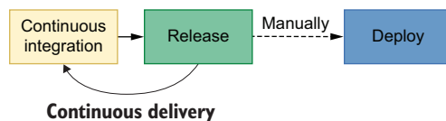
Figure 12.2 You must already perform continuous integration before implementing continuous delivery. When practicing continuous delivery, each change you integrate must be releasable so that you can deploy an up-to-date version of your software whenever you want.
