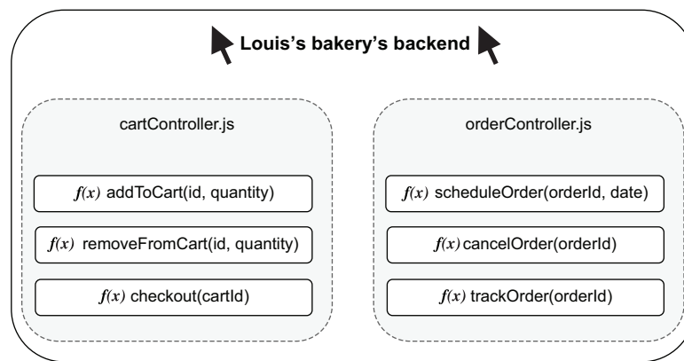
Figure 3.1 The module for placing orders and the module for tracking orders
