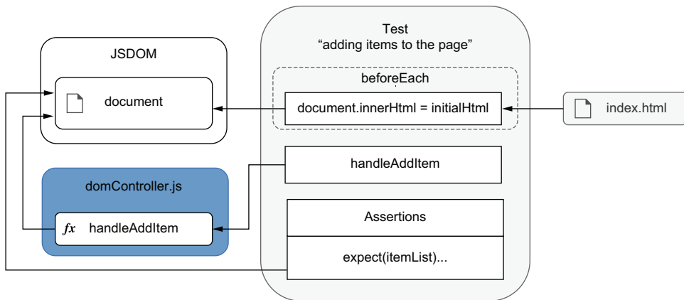
Figure 6.4 The test for handleAddItem invokes it directly, causing it to update the document.
