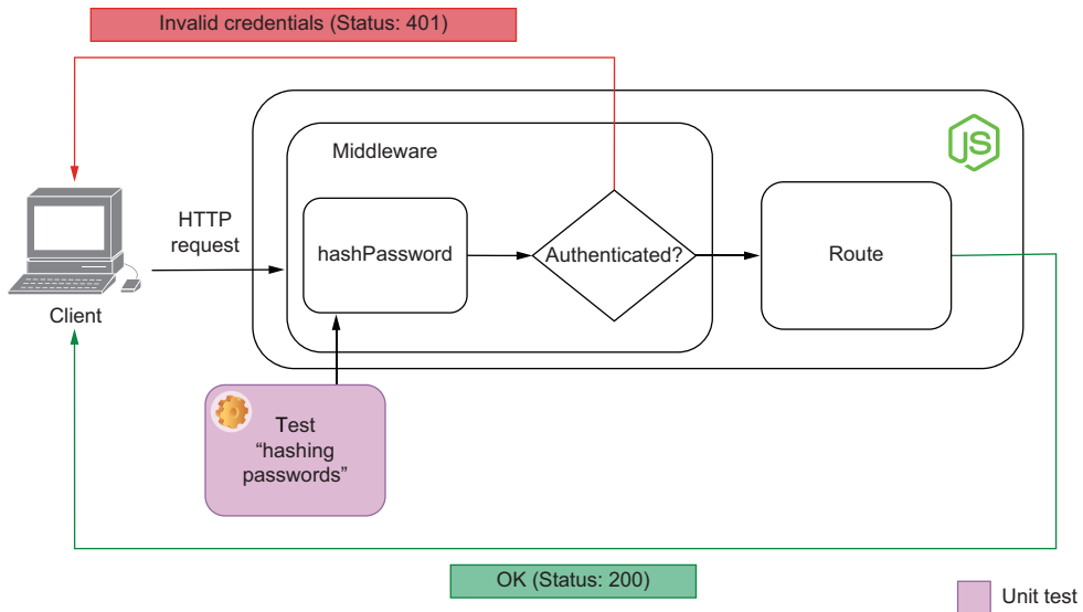
Figure 4.9 The part of the middleware with which this unit test interacts
