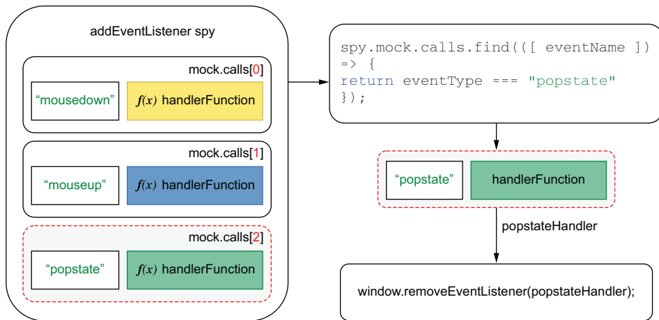
Figure 6.7 To find event handlers, you can spy on the window's addEventListener function and filter its calls by the event name passed as the first argument.
