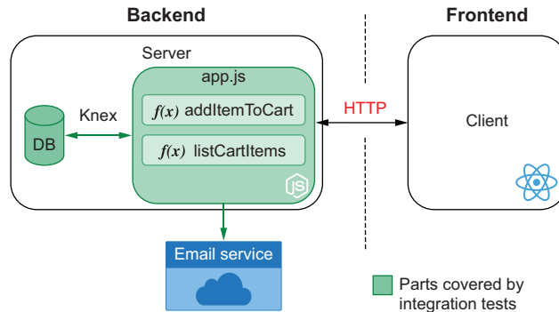
Figure 2.6 Integration tests' scope
