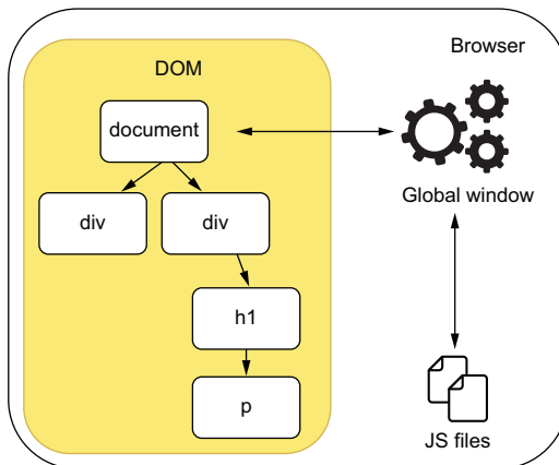
Figure 6.1 The JavaScript environment within a browser
