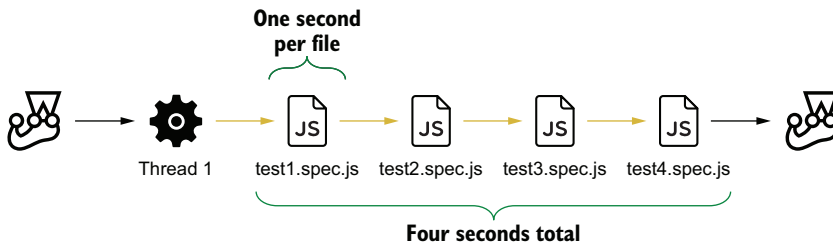
Figure 3.5 What happens when running tests sequentially
