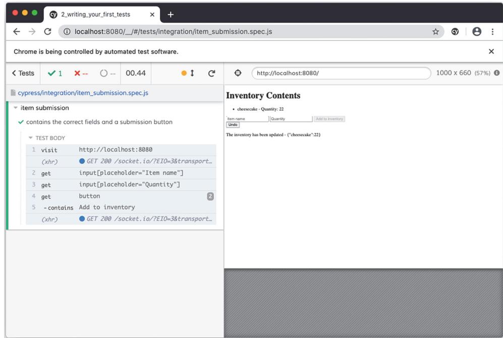
Figure 11.2 Cypress executing the test that checks the inventory management application's elements
