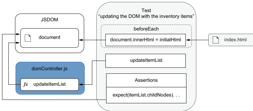
Figure 6.3 How the tests and the unit under test interact with the document
