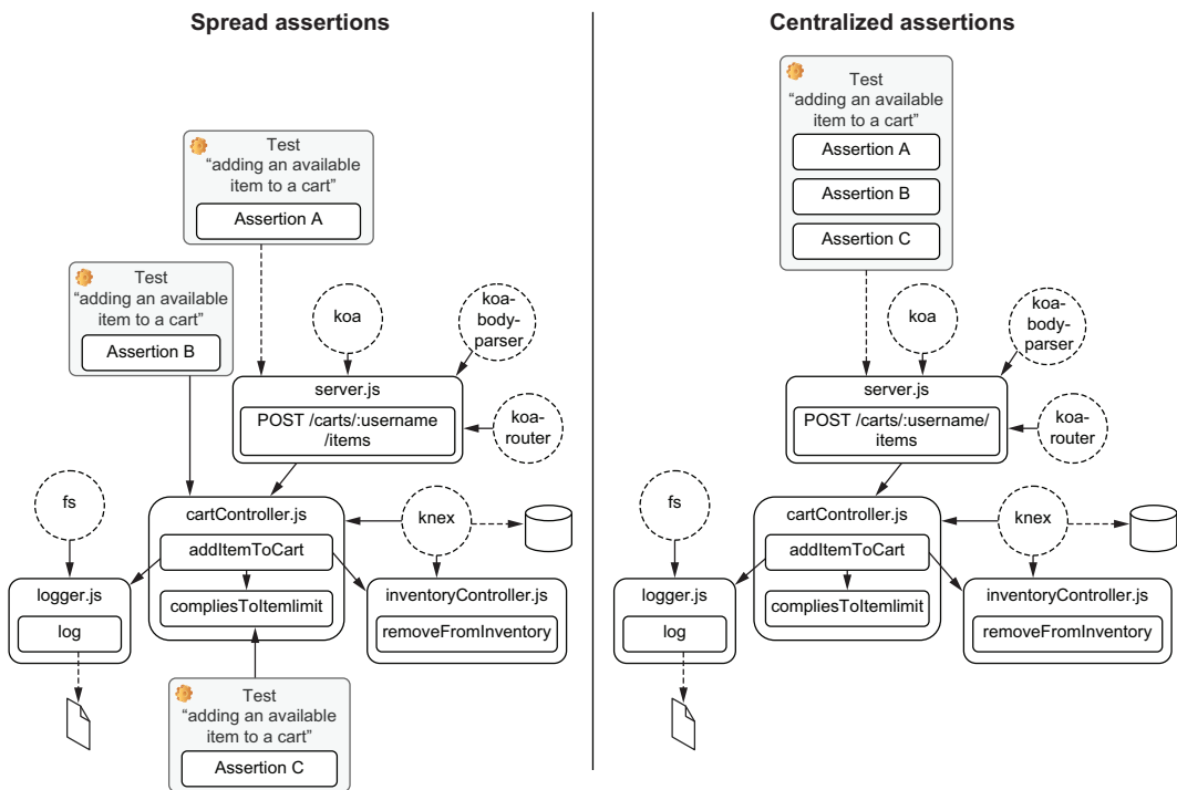
Figure 5.6 When reducing the amount of testing code, centralize your assertions in the test that covers the topmost node.
