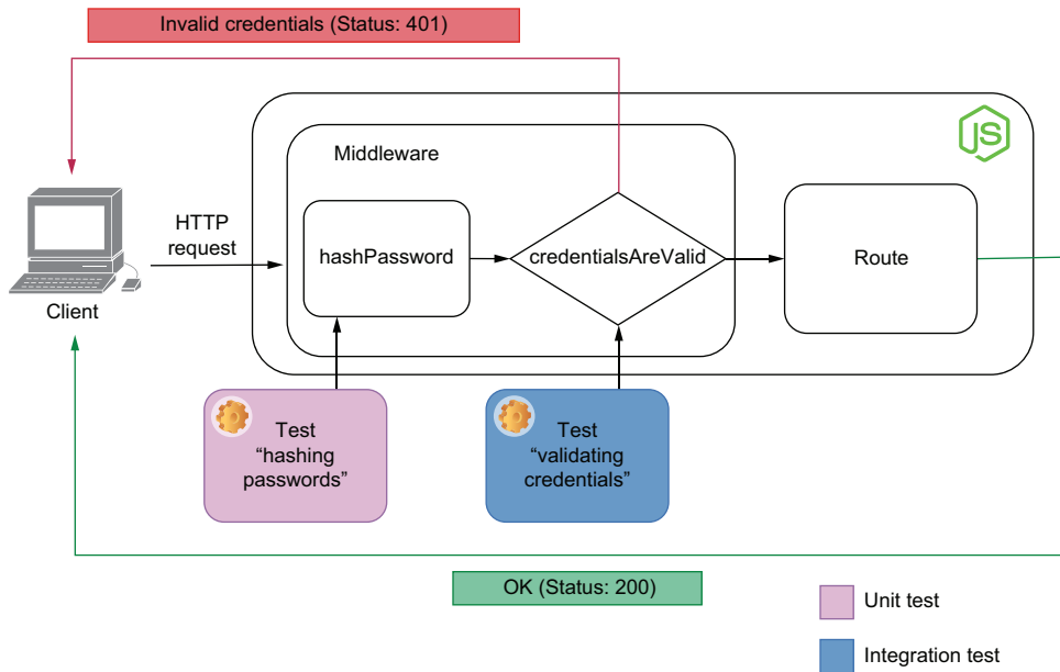
Figure 4.10 The part of the middleware with which this integration test interacts
