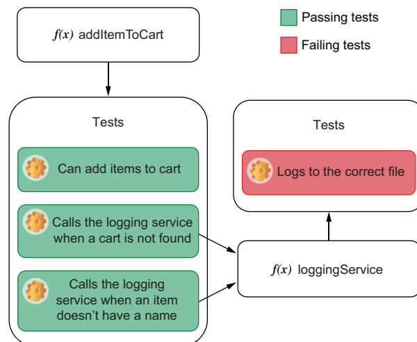
Figure 2.15 If you change the file to which loggingService writes, its tests will be the only ones to fail. The addItemToCart tests will continue to pass because they are doing what you expect: using the logging service. By structuring your tests in this way, you have fewer tests to update and more precise feedback about what piece of your software doesn't comply with the tests.
