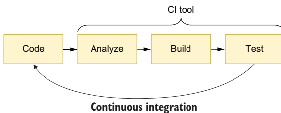
Figure 12.1 When performing continuous integration, your CI server will automatically analyze, build, and test every change you submit.
