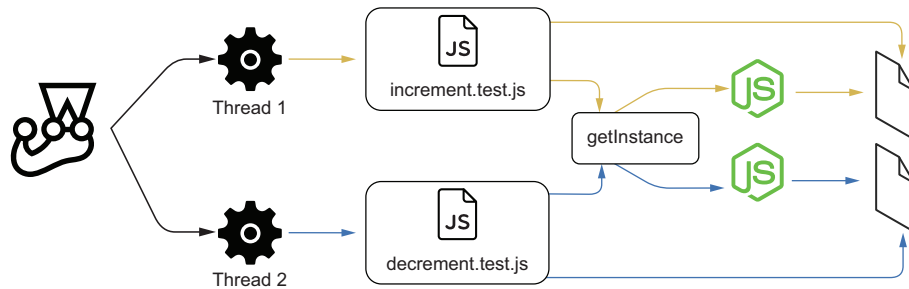
Figure 5.2 Each test obtains a different instance of the module through getInstance and checks a different underlying resource.
