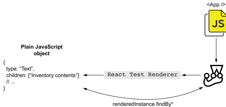
Figure 7.6 React’s test renderer doesn’t render components to a JSDOM instance. Instead, it creates a plain JavaScript object that contains a few methods that you can use to find and inspect rendered elements.
