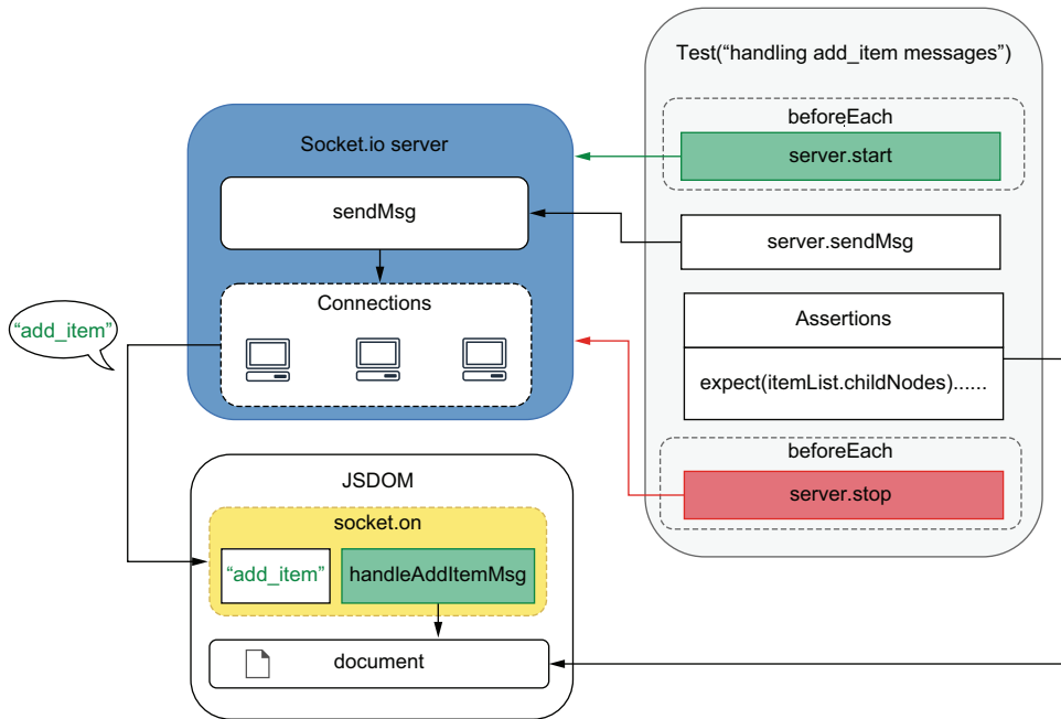
Figure 6.9 How your tests communicate with your Socket.io server, causing it to update the document so that they can perform assertions
