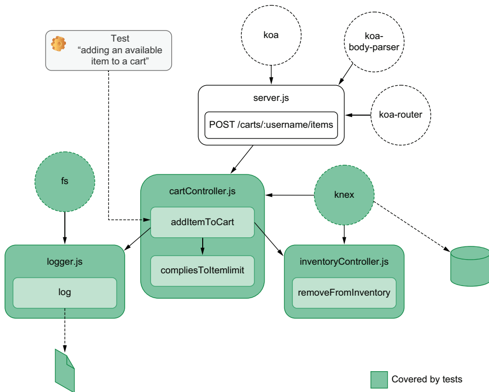
Figure 5.4 An integration test for addItemToCart will also cause compliesToItemLimit , removeFromInventory , and log to be invoked.
