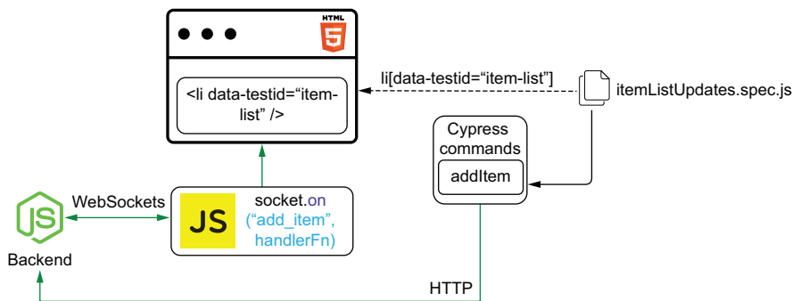
Figure 11.4 Your test adds items through HTTP requests sent directly to the backend. The server then communicates with the client through WebSockets to update the list of products.
