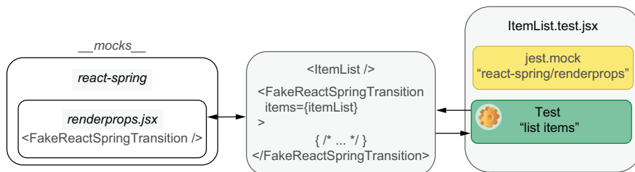
Figure 8.5 How your test double is used by ItemList when running tests
