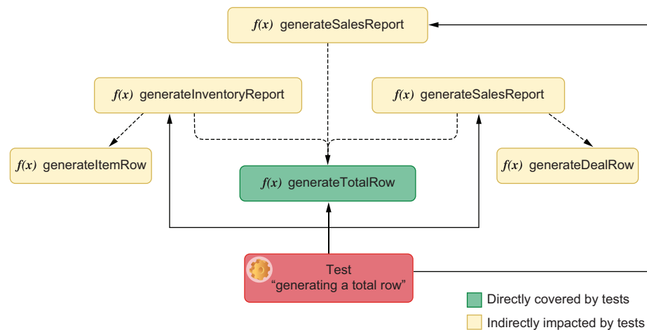
Figure 9.14 A test that covers the generateTotalRow function will indirectly create reliability guarantees that impact all of its dependants.
