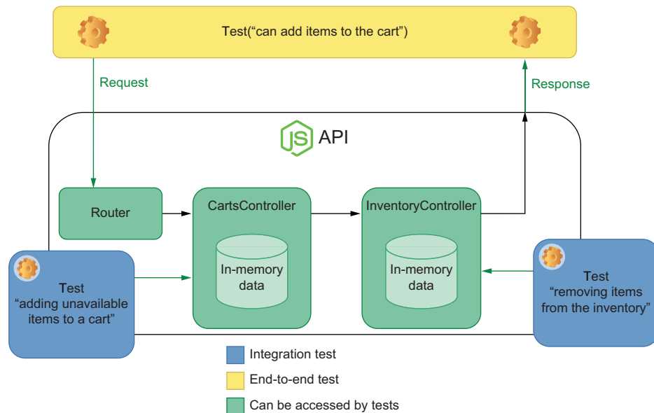
Figure 4.4 Which parts of your application each end-to-end and integration test has access to
