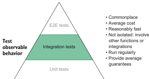
Figure 2.7 Integration tests’ placement in the testing pyramid
