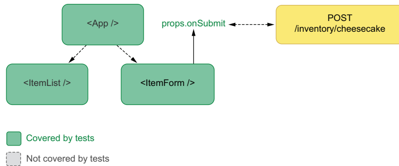
Figure 8.2 The coverage of a test that renders App , interacts with its child form, and verifies the item list's elements
