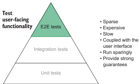
Figure 2.9 End-to-end tests' placement in the testing pyramid
