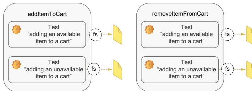
Figure 5.7 In each test that depends on the logger, you will repeat the same code to read the log file and perform similar assertions.
