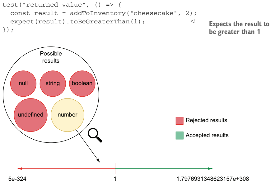
Figure 3.8 The range of results accepted by the toBeGreaterThan assertion
