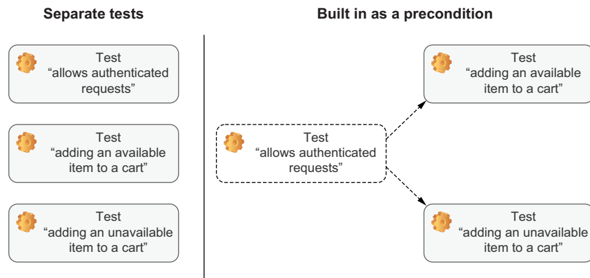
Figure 5.9 By relying on a certain behavior to happen in other tests, you can avoid writing a specific test for it.
