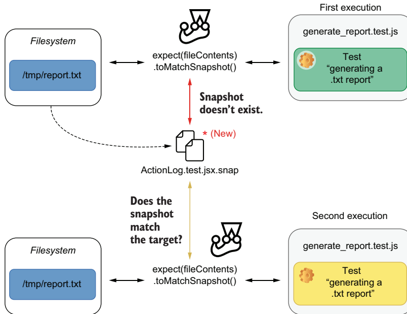
Figure 8.8 Jest creates a snapshot with the report's contents the first time it runs. The second time it runs, it will compare the report's actual content with what it had saved in the snapshot file.
