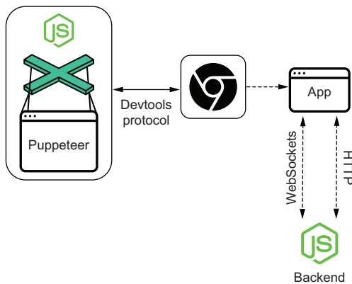
Figure 10.9 Puppeteer directly controls Chrome and Chromium through their DevTools Protocol.
