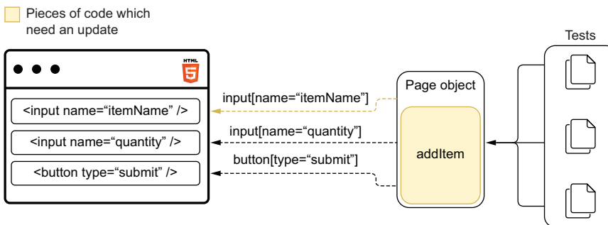
Figure 11.8 By centralizing your selectors into a page object, when your selectors break, you need to update only the page object.
