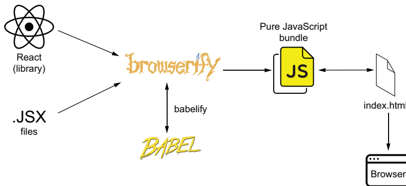
Figure 7.1 Your application's build process, from bundling and transforming your code, to executing it in a browser
