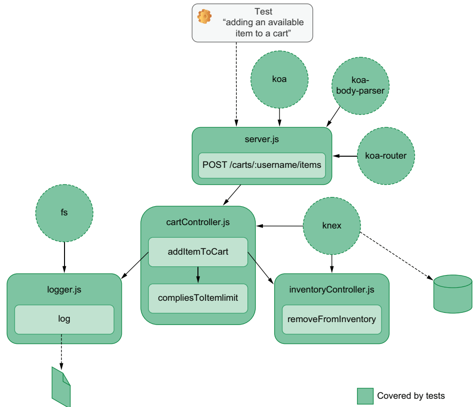
Figure 5.3 An end-to-end test that sends a request to this route will cause functions like addItemToCart , compliesToItemLimit , removeFromInventory , and log to be executed.
