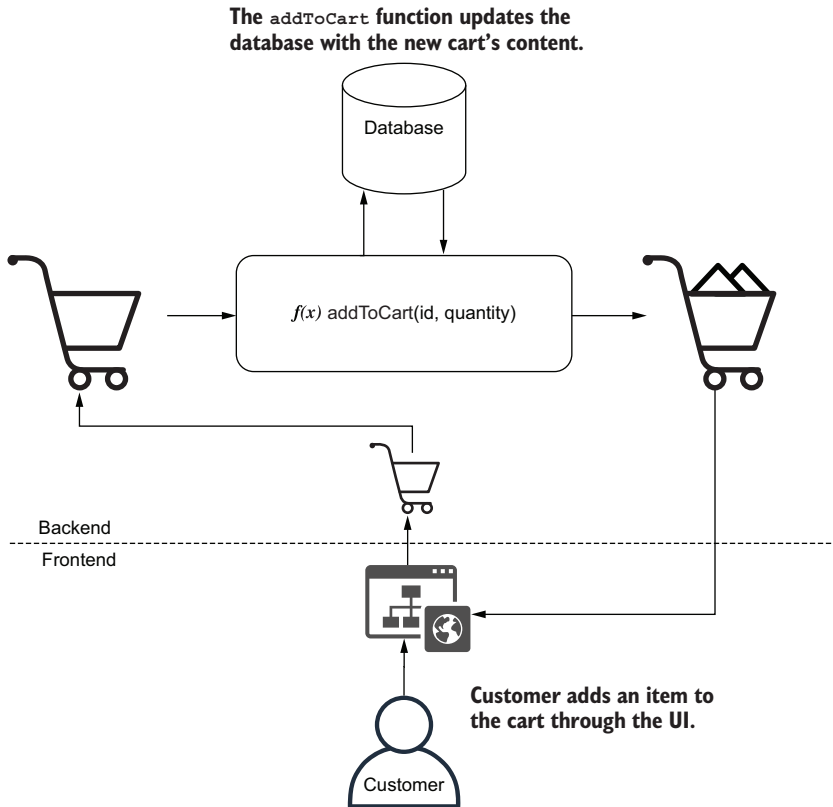
Figure 1.4 The desired action flow for adding only available items to a cart
