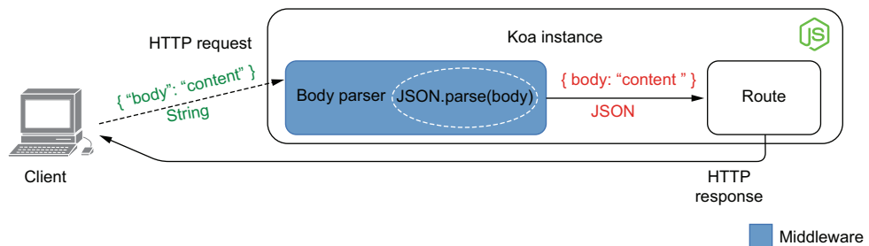
Figure 4.7 How the body-parser middleware works for JSON bodies
