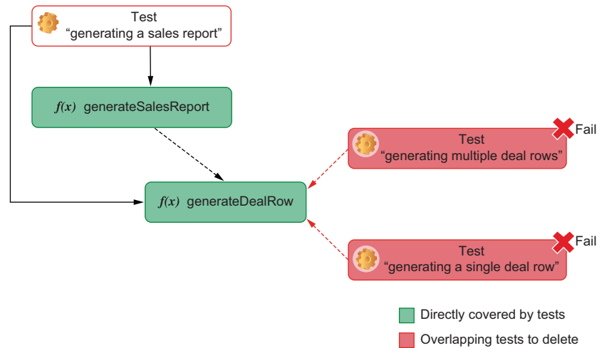
Figure 9.18 You can delete overlapping tests with weaker reliable guarantees during your software’s maintenance phase.
