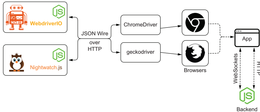
Figure 10.8 Instead of having to set up your own testing infrastructure, you can use libraries like Nightwatch.js or WebdriverIO, which ship with all the tools necessary for writing tests.
