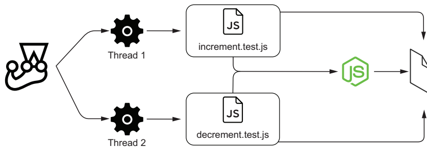
Figure 5.1 Both tests using the same module and the same underlying resource
