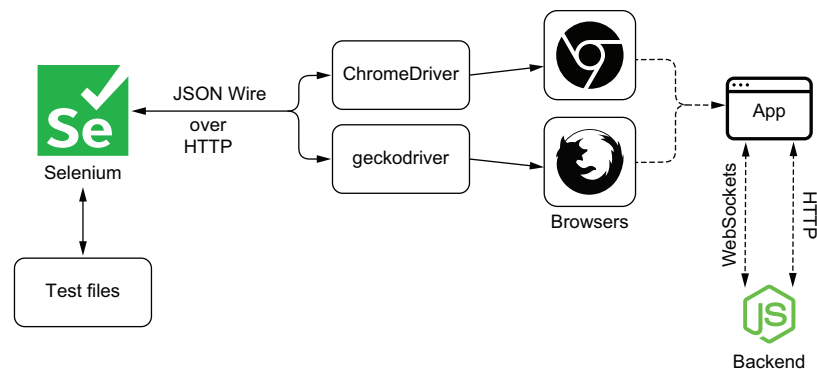
Figure 10.6 Different web drivers control different browsers.
