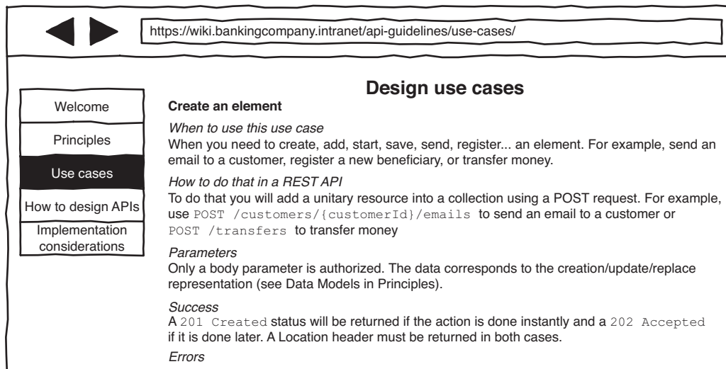
Figure 13.3 A use case description in the Banking Company's API design guidelines
