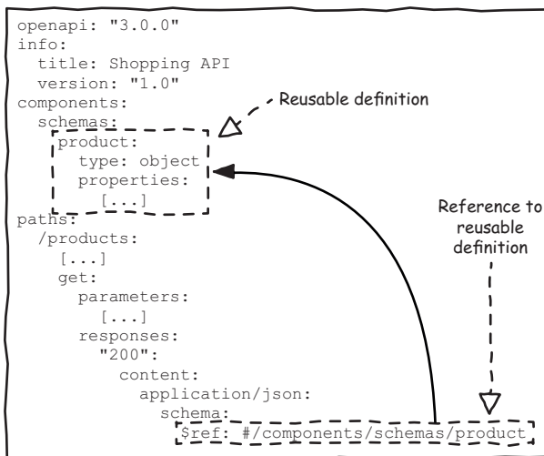
Figure 4.18 Reusable components in the OAS document
