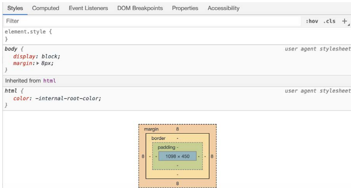
Figure 1.36: The Styles tab of the right-hand panel of the Elements tab
