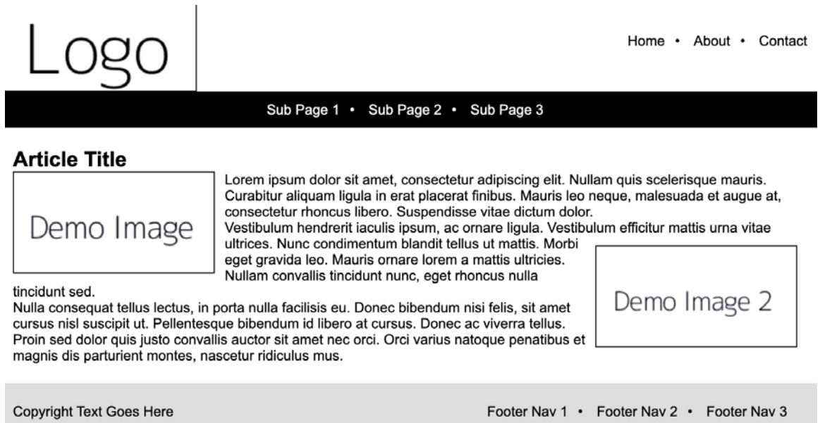
Figure 11.6: Browser output
