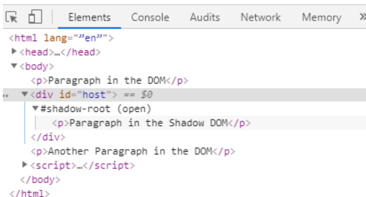
Figure 12.13: Shadow DOM with a style not applied to it
