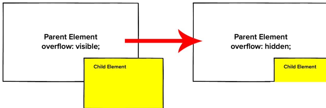
Figure 8.13: Overflow visible and hidden in action
