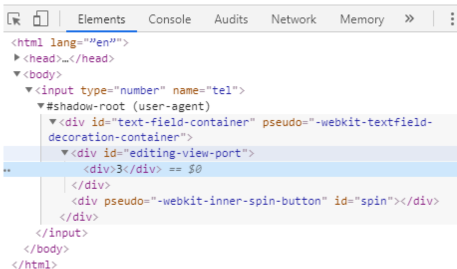
Figure 12.16: Inspecting the Shadow DOM of a number input
