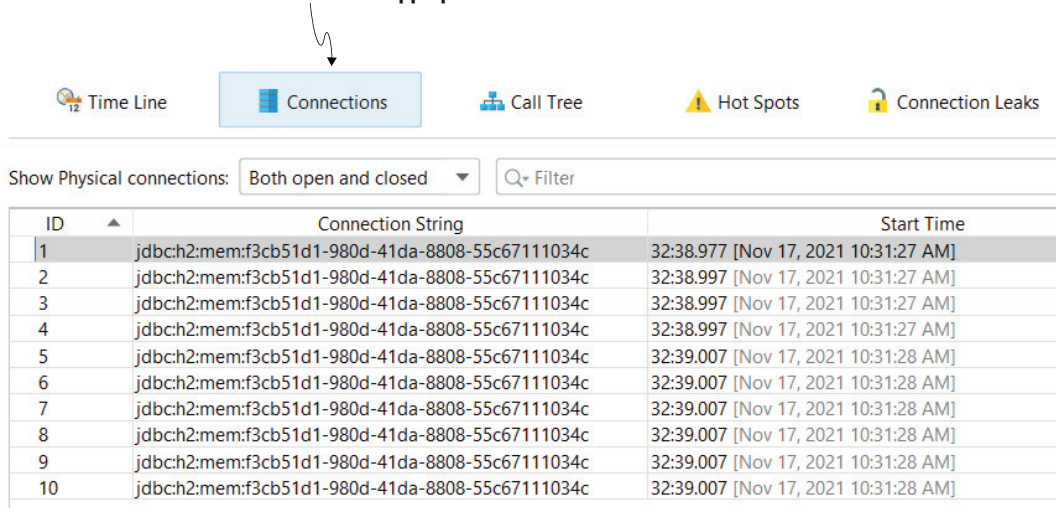
Figure 8.9 By sending a request to the /products endpoint, we see that the app creates many connections. We don't know exactly what the app does, but this can be alarming.
