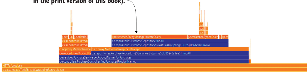
Figure 8.20 Colorizing levels helps highlight specific parts of the flame that you want to focus on. You can use multiple colors at the same time, which can help you to compare execution times.
