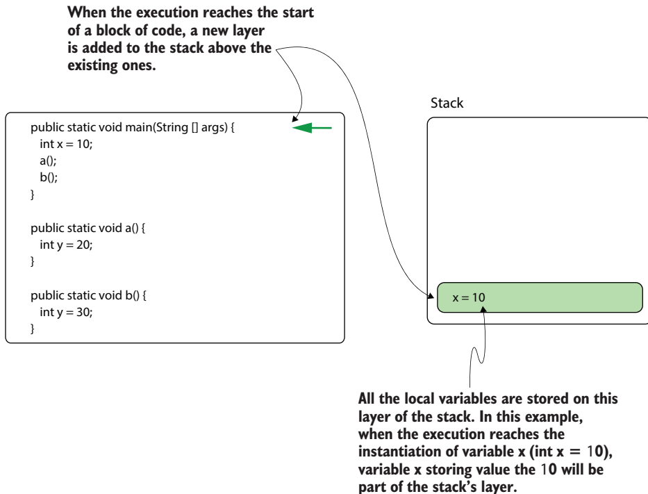
Figure E.5 When the execution reaches the start of a block of code, a new layer is created in the thread's stack. All the variables the block of code defines are stored in this new layer. The layer is removed when the block of code ends. This way, we know that the values in this part of the memory are released when they're no longer needed.
