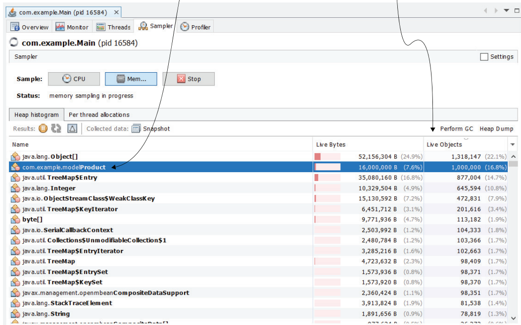
Figure 11.4 We can sort the sampled results by the number of instances (live objects). This gives us clues on whether some capability creates a large number of objects that are negatively affecting the memory allocation.
