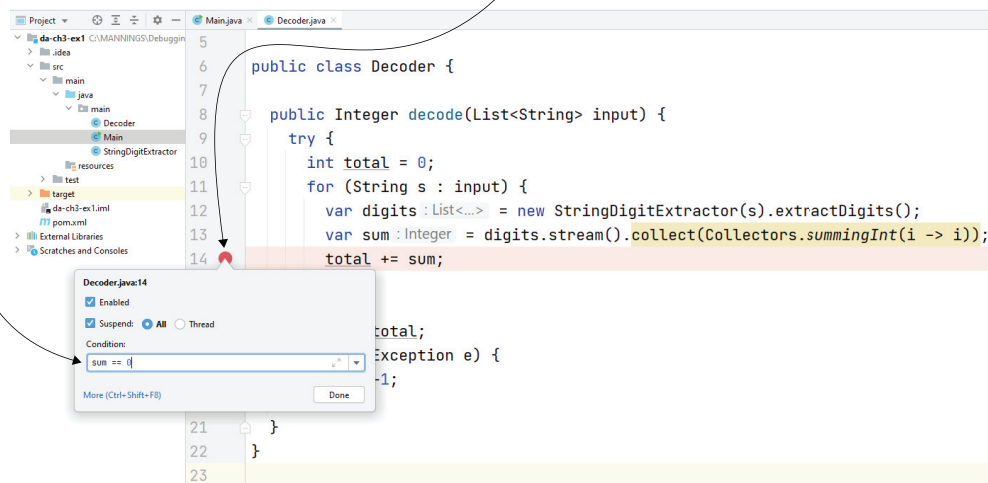
Figure 3.1 Using a conditional breakpoint to pause the execution just for specific cases. In this figure, we want to pause the execution on line 14 only if sum is zero. We can apply a condition on the breakpoint that instructs the debugger to consider that breakpoint only if the given state is true. This helps you more quickly get to a scenario you want to investigate.
