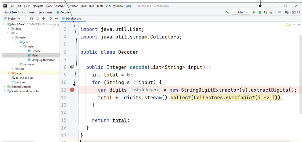
Figure 2.6 Click near the line number to add a breakpoint on a specific line. Then, run the app with the debugger. The execution pauses on the line you marked with a breakpoint and allows you to control it manually.
