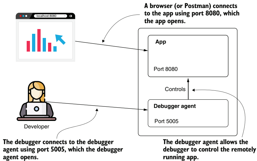
Figure 4.11 The debugger tool that runs on the developer's computer connects to the debugger agent on port 5005. The debugger agent allows the debugger tool to control the app. The app also opens a port, but this port is for its clients (the browser, in the case of a web app).
