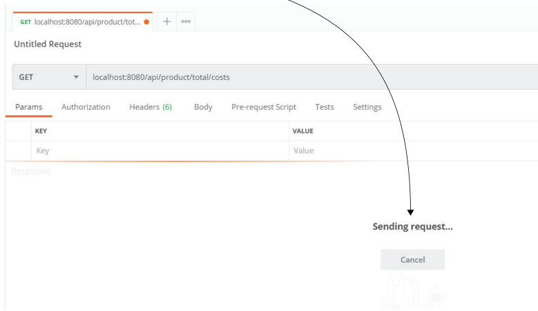
Figure 4.15 When using Postman to send the request, the response doesn't come back immediately. Instead, Postman waits indefinitely for the response because the app paused the execution on the line you marked with a breakpoint.
