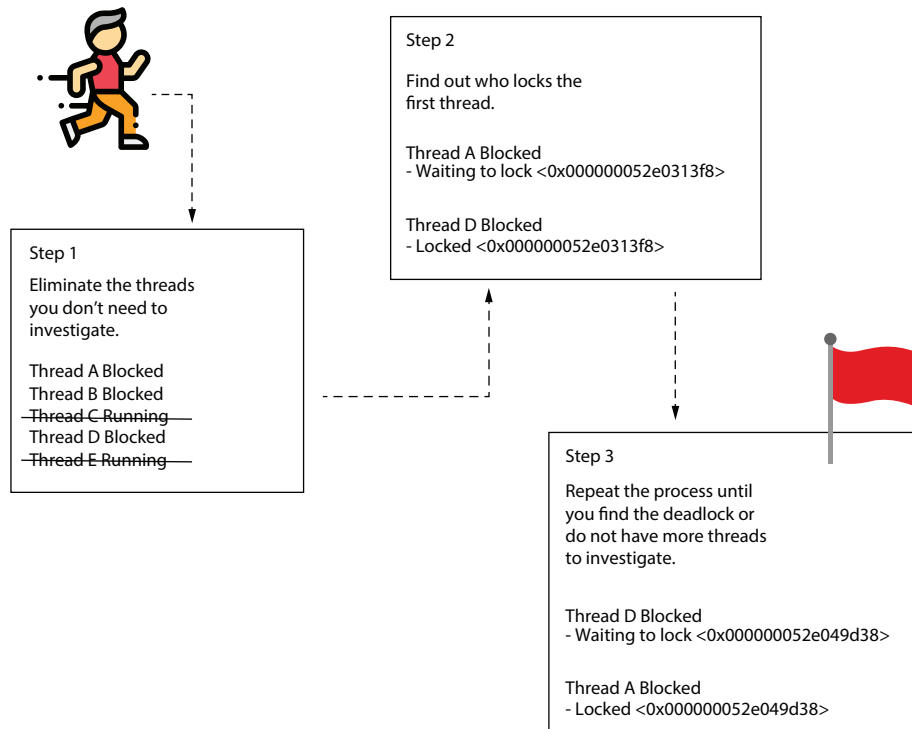
Figure 10.8 To find a deadlock with a thread dump, follow these three easy steps. First, remove all threads that are not blocked. Then, start with one of the blocked threads and find what is blocking it using the lock ID. Continue this process for each thread. If you return to a thread you already investigated, it means you found a deadlock.
