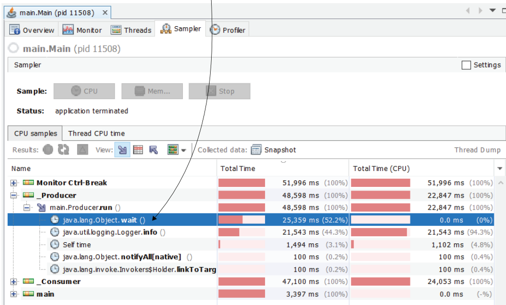
Figure 9.17 By analyzing the details, we can see that the self execution time is not that long, but the thread is blocked and thus waits for a longer time.
