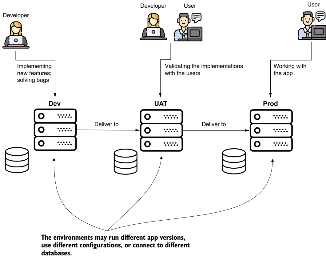
Figure 4.2 When building a real-world app, developers often use multiple environments. First, they build the app in development (dev) environments. Then, once a feature or a solution is ready, they present it to users (or stakeholders of the app) using a user acceptance test (UAT) environment. Finally, after the stakeholders confirm that the implementation works, they install it in a production (prod) environment.
