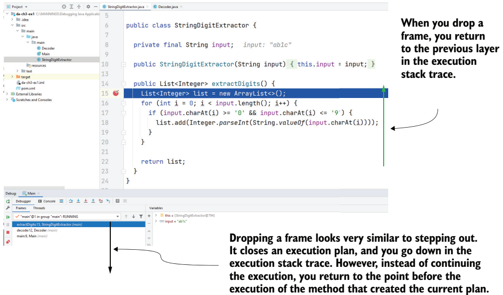
Figure 3.12 When you drop a frame, you return to the previous layer in the execution stack trace before the method call. This way, you can replay the method execution either by stepping into it again or stepping over it.
