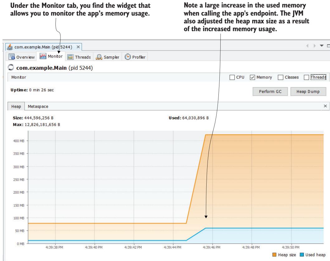
Figure 11.1 The memory widget in the Monitor tab in VisualVM helps you to identify if the app spends more memory than usual at any given time. Often, widgets in the Monitor tab, such as CPU and memory consumption, give us clues on how to continue our investigation. When we see that the app consumes an abnormal amount of memory, we may decide to continue with memory profiling the execution.
