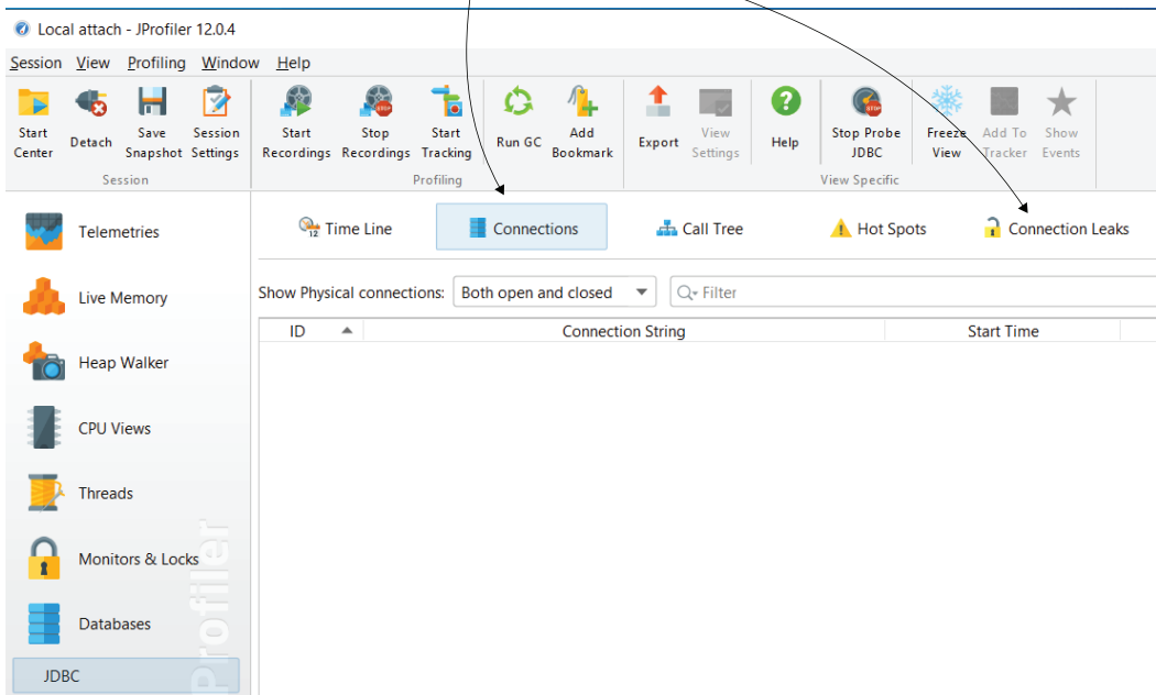
Figure 8.8 The Connections and Connection Leaks tabs show details about the connections the app creates, including potential problematic connections. We'll use these details to understand where the problem in our app comes from.
