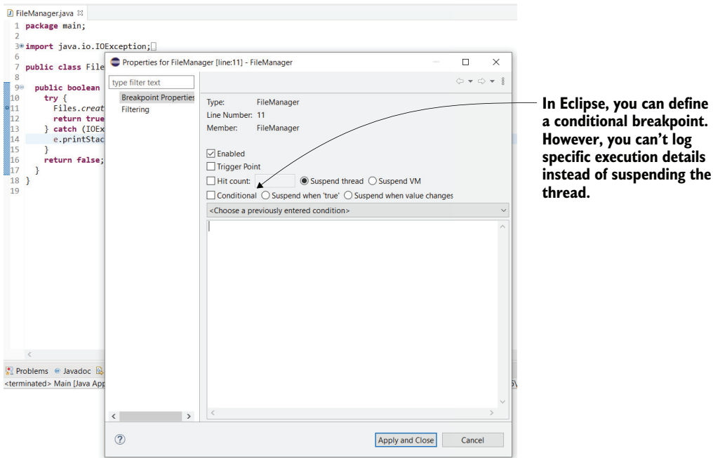
Figure 3.4 Not all IDEs offer the same debugging tools. All IDEs give you the basic operations, but some features, such as logging the execution details instead of pausing the execution, may be missing. In Eclipse, you can define conditional breakpoints, but you can't use the logging feature.
