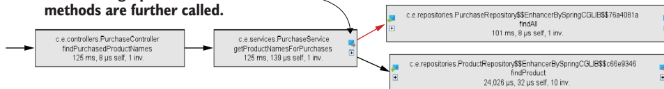
Figure 8.15 A call graph shows the execution, focusing mainly on the relationship between objects and method calls. You can linearly navigate the method execution chain to determine where each method is called from and what that method calls. The call graph also shows objects and methods that are part of the app's codebase and those of libraries and frameworks the app uses.
