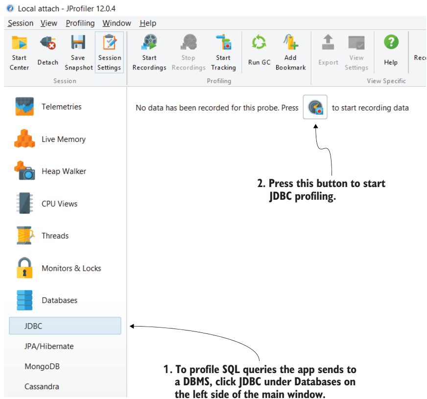
Figure 8.7 You can start JDBC profiling with JProfiler by first selecting JDBC in the left menu; then you begin the profiling process.
