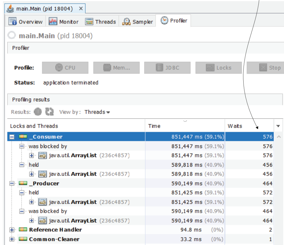
Figure 9.18 The lock pattern is similar to our previous results, but the threads are locked less frequently.
