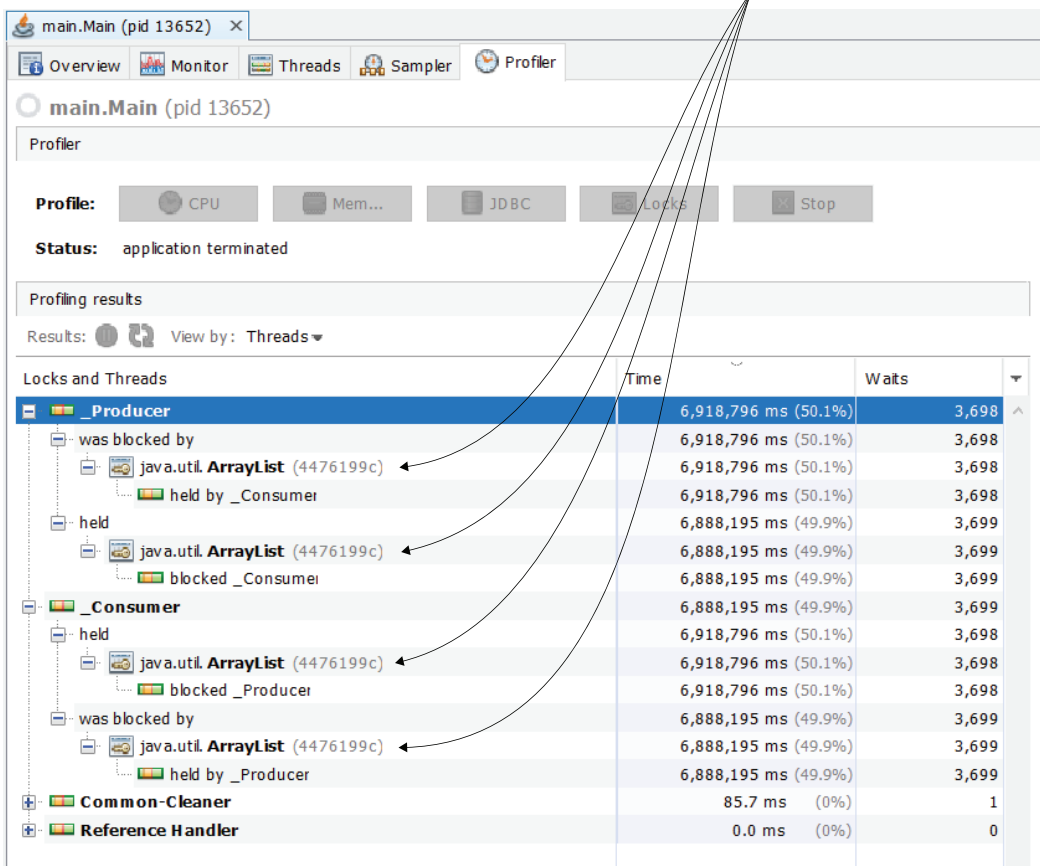
Figure 9.9 Both threads use the same monitor to block each other. While one thread executes the synchronized block with an ArrayList instance monitor, the other waits. This way, one thread is locked for 3,698 times and the other for 3,699.
