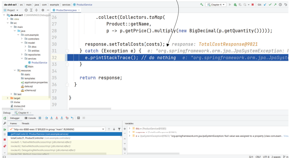
Figure 4.17 The step over operation shows that the app throws an exception. Now you have an idea of what the problem is and can decide how to solve it.
