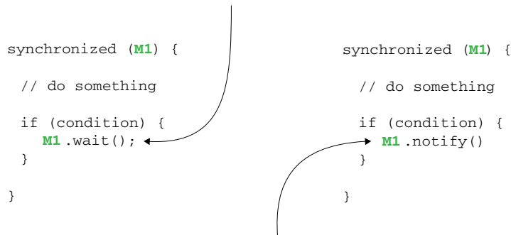
Figure D.8 In some cases, a thread should pause from executing and wait for something to happen. To make a thread wait, the monitor of a synchronized block can call its wait() behavior. When the thread becomes executable again, the monitor can call the notify() or notifyAll() methods.
