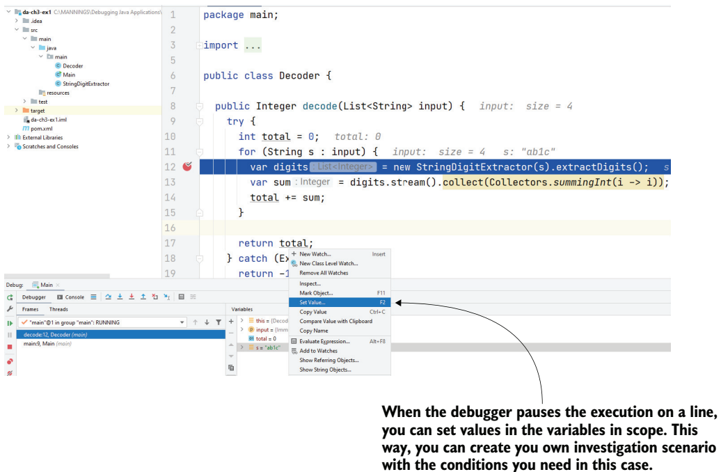
Figure 3.8 Setting a new value in a variable in scope. The debugger shows you the values for the variables in scope when it pauses the execution on a given line. You can also change the values to create a new investigation case. In some cases, this approach can help you to validate your suspicions about what the code does.
