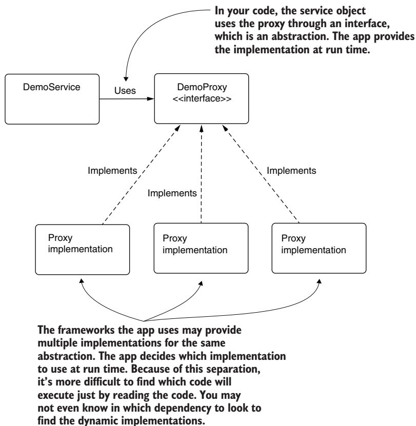
Figure 7.7 The framework keeps the implementations for an abstraction separate and provides them dynamically during execution. Because the implementation is decoupled and the app provides it during run time, it's more difficult to find it by reading the code.
