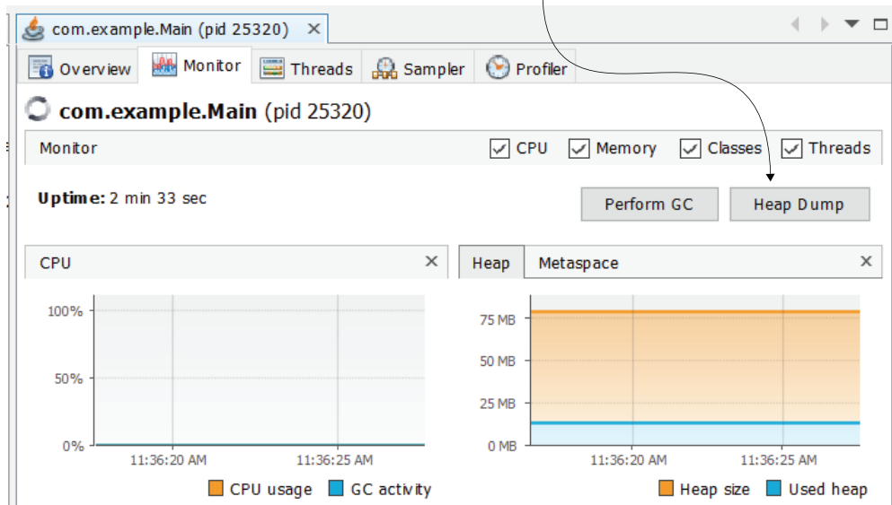
Figure 11.9 Press the Heap Dump button in VisualVM's Monitor tab to get a heap dump for the selected process. VisualVM opens the dump as a tab, and you can further investigate it or save it anywhere you want.
