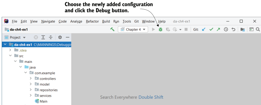
Figure 4.12 You can now run the debugger using the newly added configuration. Click the small bug icon to start the debugger.
