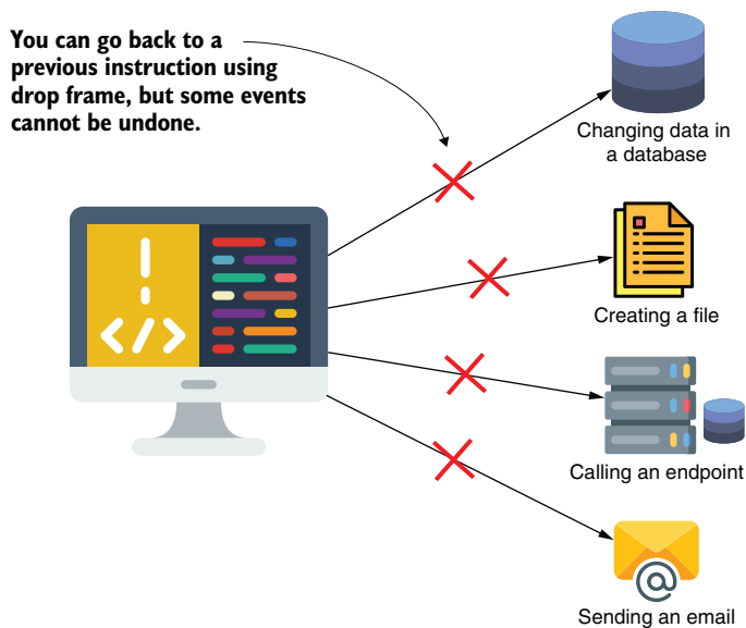
Figure 3.15 Using the drop frame operation can result in some events that can't be undone. Examples include changing data in the database, changing data in the filesystem, calling another app, or sending an email message.
