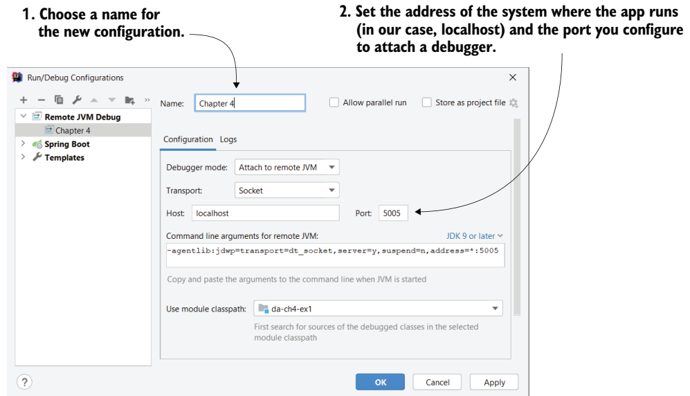
Figure 4.10 Give a name to the new configuration you add and specify the address of the environment and port you configured the debugger agent to listen on (here, port 5005 when starting the app).
