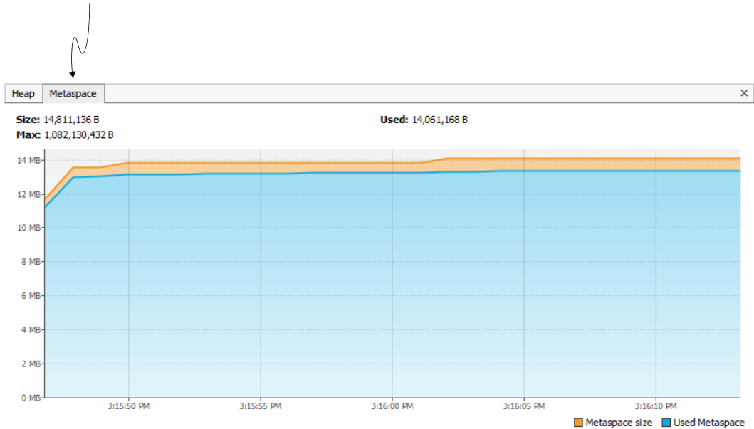
Figure 6.13 The metaspace is a part of the memory used to store class metadata. In particular cases, the metaspace can be overflowed. A VisualVM memory allocation widget also shows the usage of the metaspace.
