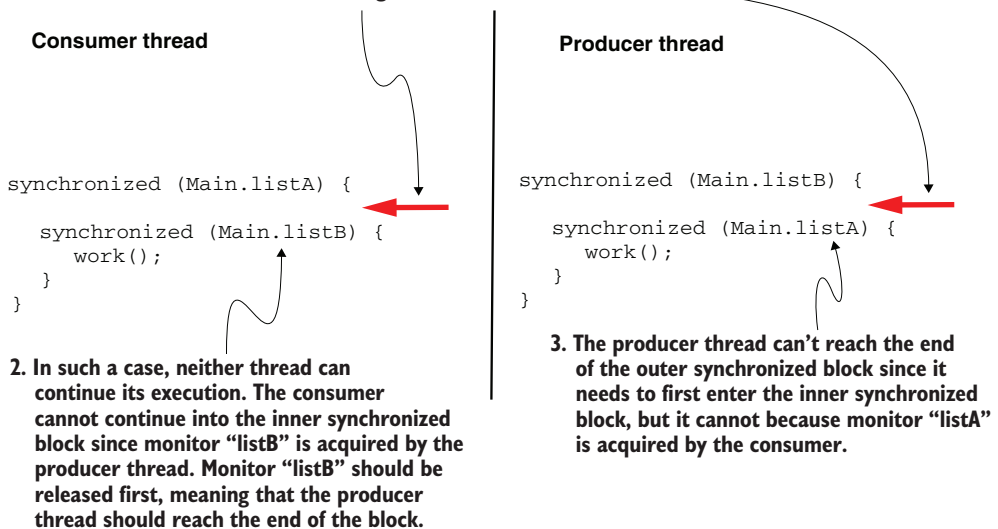
Figure 10.1 If both threads enter the outer synchronized block, but not the inner one, they remain stuck and wait for each other. We say that they went into a deadlock.
