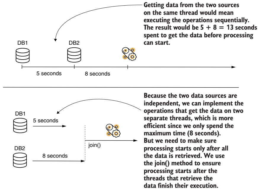
Figure D.10 In some cases, you can improve the app’s performance using multiple threads. But you need to make some threads wait for others since they depend on the execution result of those threads. You can make a thread wait for another using a join operation.
