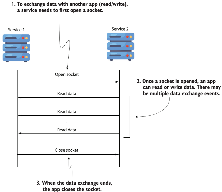
Figure 12.6 When an app starts a data exchange, it first opens a socket. To exchange the data, the app can execute multiple data exchange events (read or write data events). When the data exchange ends, the app closes the socket.
