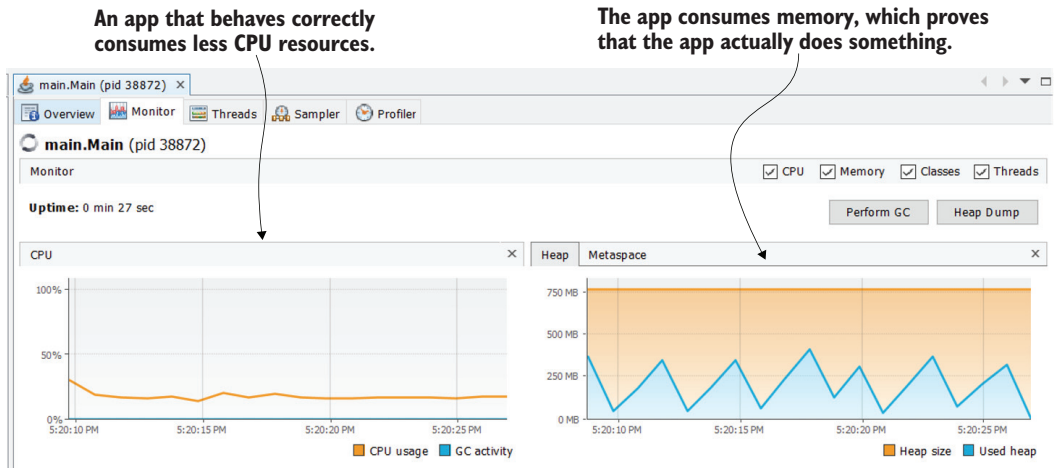
Figure 6.8 After correctly synchronizing the code, the resource consumption widgets look different. The CPU consumption is lower, and the app uses some memory.
