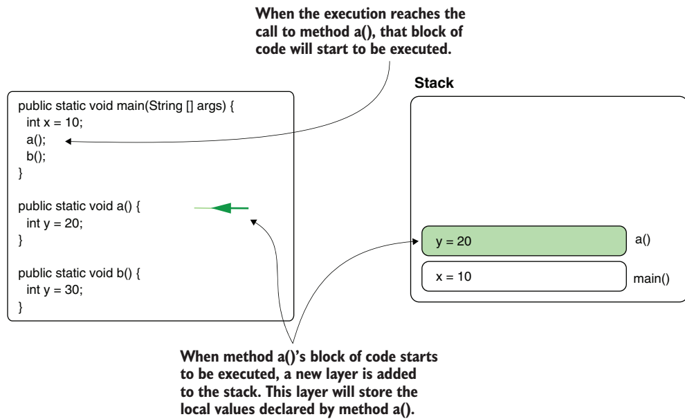
Figure E.6 Another block of code can be called from one in execution. In this case, method main() calls method a() . Since main() didn't finish, its layer is still part of the stack. Method a() creates its own layer where the local values it defines are stored.
