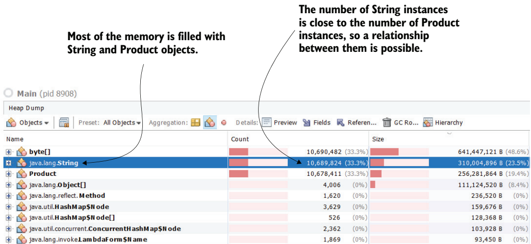
Figure 1.10 A heap dump is like a map of the heap memory. If you learn how to read it, it gives you invaluable clues about how the app internally processes data. A heap dump helps you investigate memory problems or performance issues. In this example, you can easily find which object fills most of the app's memory and that the Product and String instances are related.
