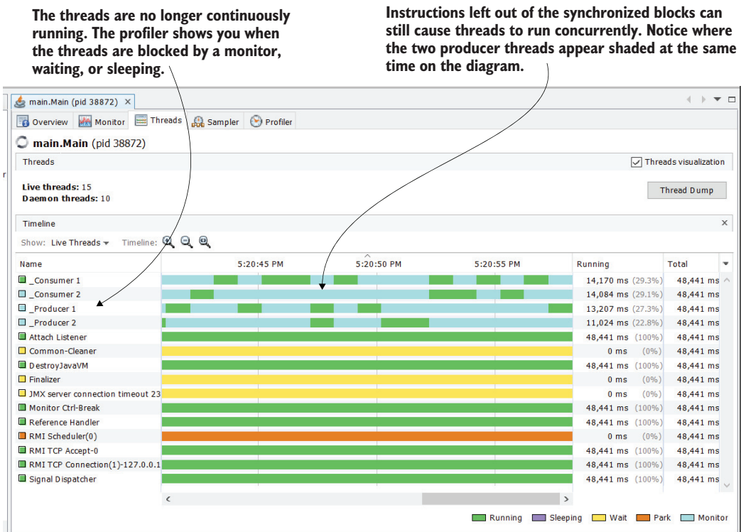
Figure 6.9 The Threads tab helps you to visualize the execution of the threads in your app. Since the threads' names start with an underline, you can simply sort them by name to see them grouped. Notice that their execution is interrupted from time to time by the monitor, which allows just one thread at a time through the synchronized blocks of code.
