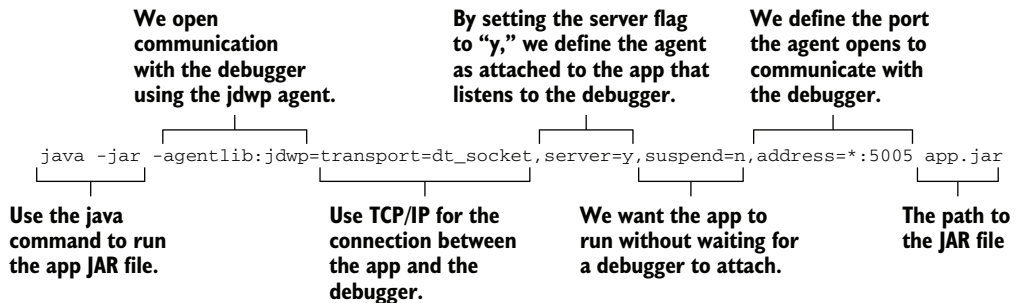
Figure 4.5 When debugging an app locally, the IDE attaches the debugger. But when running an app in a remote environment, you must attach a debugger agent at the app start yourself.
