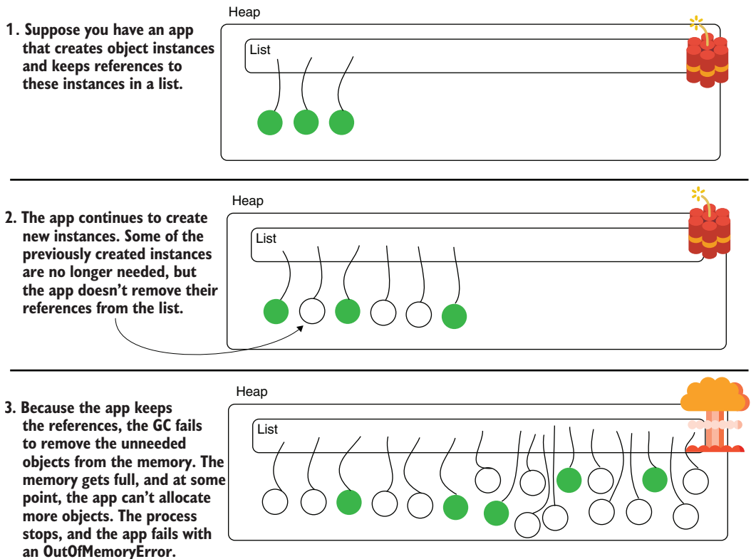
Figure 6.10 An OutOfMemoryError is like a ticking bomb. An app fails to remove references to objects it no longer uses. The GC can't remove these instances from the memory because the app keeps their references. While more objects are created, the memory gets full. At some point, there's no more space in the heap to allocate other objects, and the app fails with an OutOfMemoryError .
