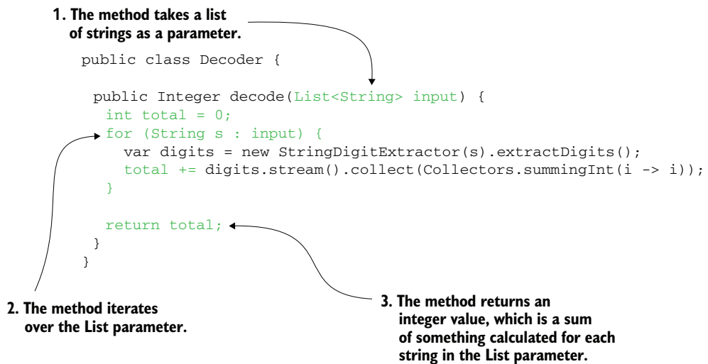
Figure 2.4 Assuming you know the language fundamentals, you can easily see that this code takes a collection as an input and parses the collection to calculate an integer.
