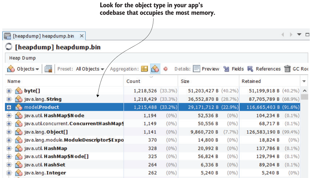
Figure 11.13 Use sorting on columns to identify which type created a large number of instances or takes up a lot of space. Always look for the first object in your app codebase. In this case, both in number of instances and size, the Product type is the first in the list.
