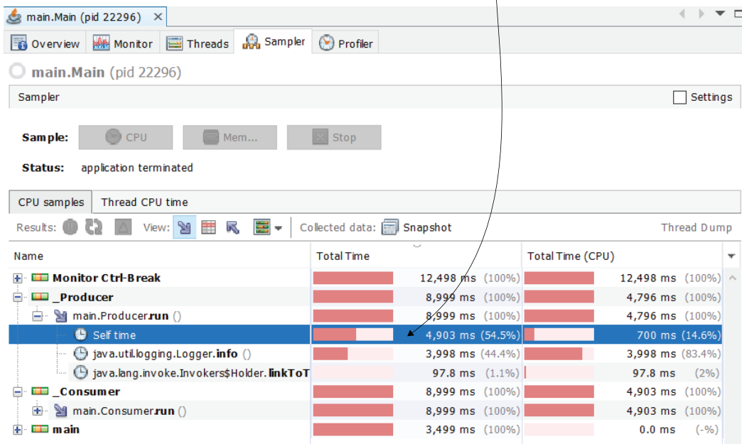
Figure 9.6 The method doesn't wait for something, but instead it waits for itself. We observe that its self-execution time is longer than the total CPU time, which usually means that the thread is locked. The thread could have been blocked by another thread.
