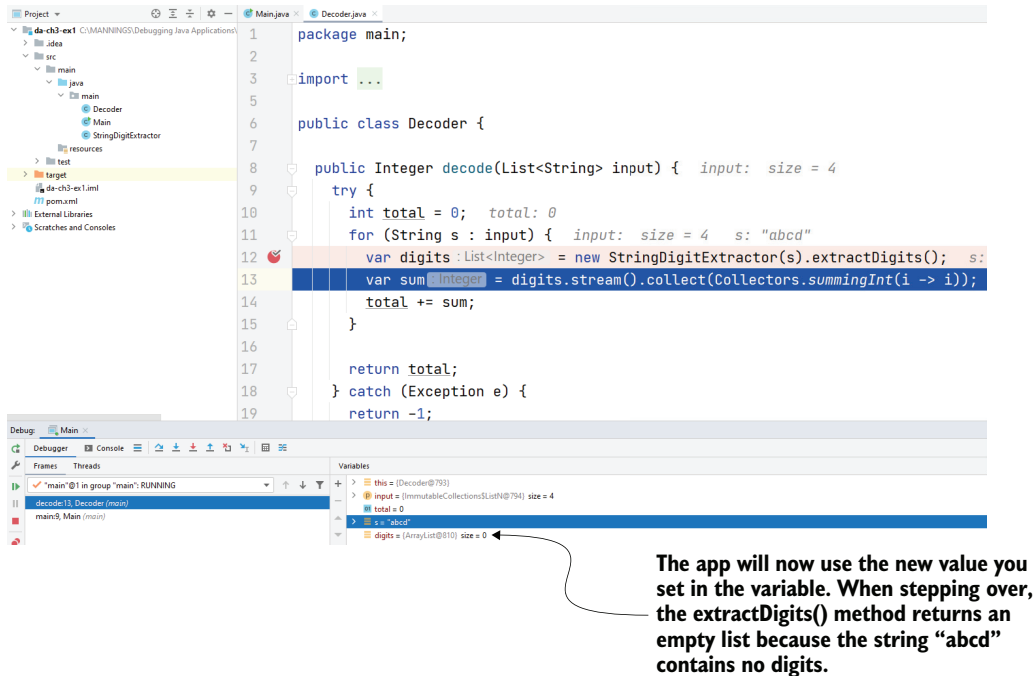
Figure 3.10 When using the step over operation, the app uses the new value you set to the s variable. extractDigits() returns an empty list because string "abcd" doesn't contain digits. Setting values in variables on the fly allows you to test different scenarios even if you don't have the input data you need.
