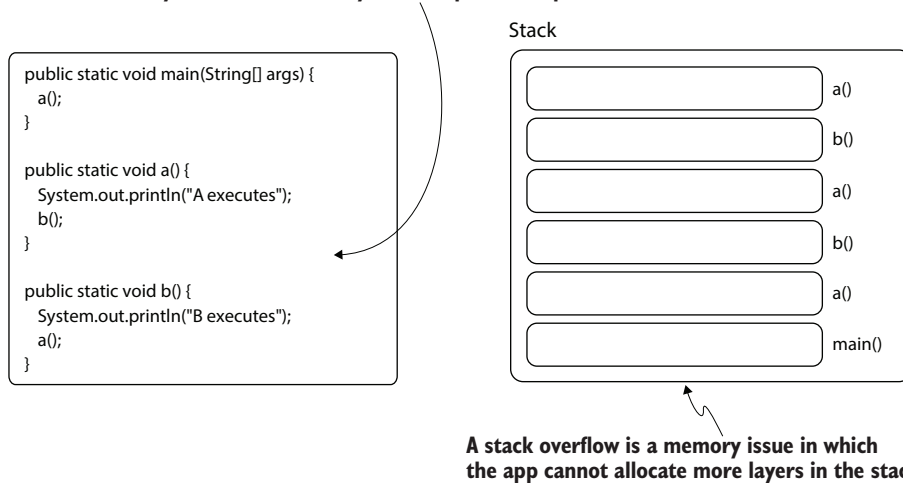
Figure E.9 Every new execution of a method creates a new layer in the stack. In case of a recursion, a method may fill the stack if it's called too many times. When the stack gets full, the app throws a StackOverflowError , and the current thread stops.
