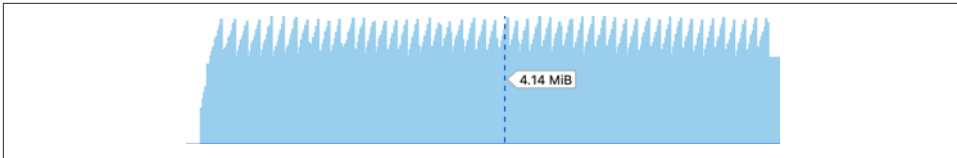
Figure 13-2. Memory usage holds steady with an autorelease pool
