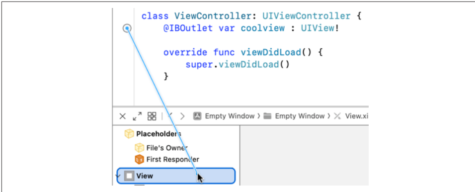
Figure 8-10. Connecting an outlet by dragging from code to nib editor
