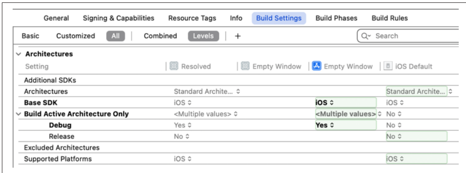
Figure 7-9. Target build settings
