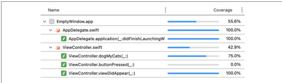
Figure 10-13. The Report navigator displays code coverage statistics
