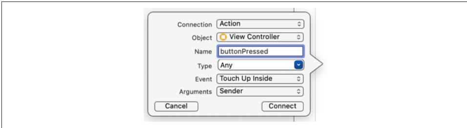
Figure 8-14. Configuring an action method declaration
