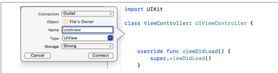
Figure 8-12. Configuring an outlet property declaration
