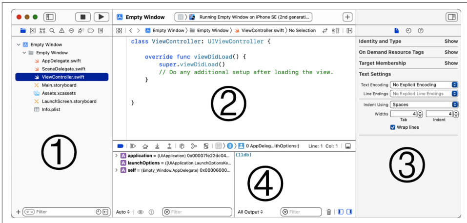
Figure 7-1. The project window
