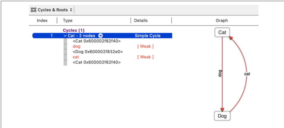
Figure 10-21. Instruments describes a retain cycle
