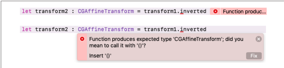
Figure 10-5. A compile error with a Fix-it suggestion
