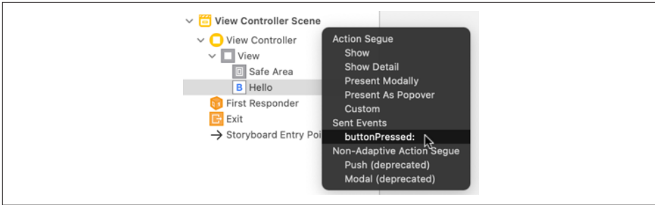
Figure 8-13. A HUD showing an action method
