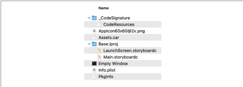
Figure 7-14. Contents of the app package
