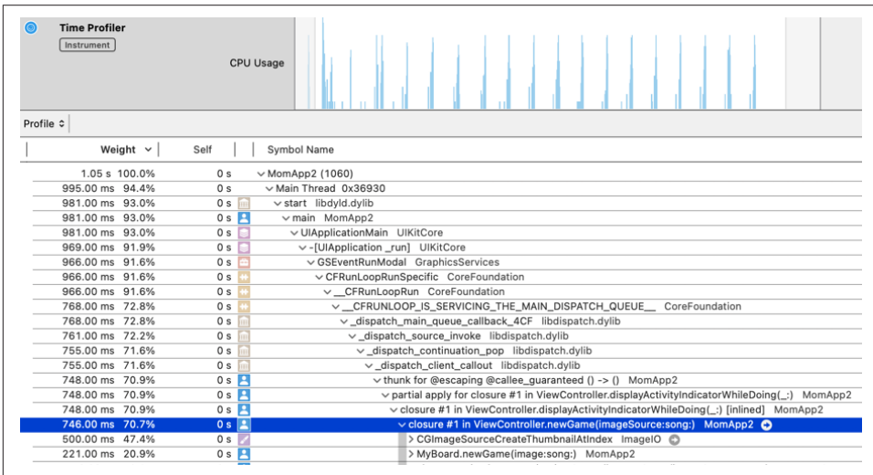
Figure 10-22. Drilling down into the time profile
