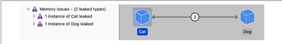
Figure 10-19. The memory graph displays a leak
