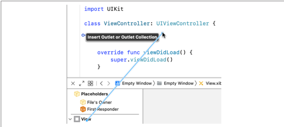
Figure 8-11. Creating an outlet by dragging from nib editor to code
