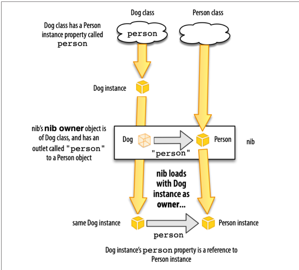
Figure 8-7. An outlet from the nib owner object
