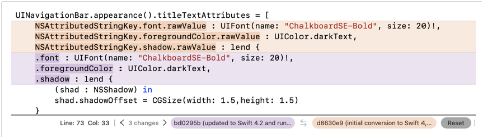
Figure 10-3. Version comparison
