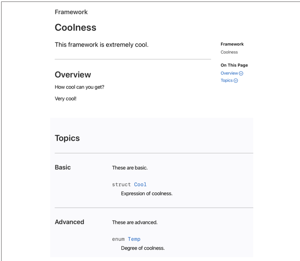
Figure 9-4. Custom framework documentation landing page
