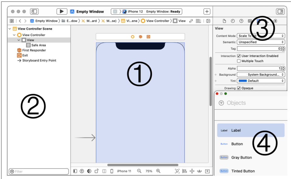
Figure 8-1. Editing a nib file
