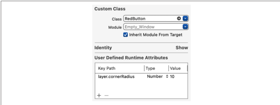
Figure 8-15. Rounding a button's corners with a runtime attribute
