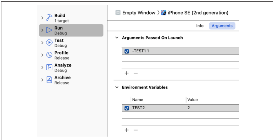
Figure 10-2. The Arguments tab of the scheme's Run action
