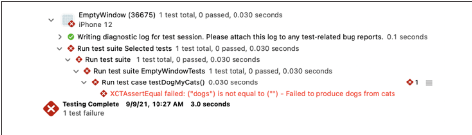
Figure 10-12. The Report navigator details a test failure
