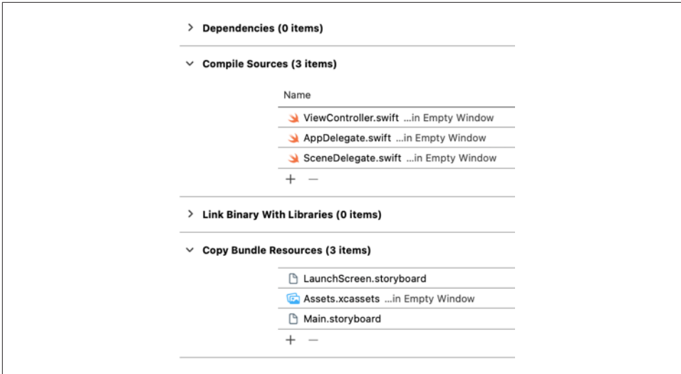
Figure 7-8. The app target's build phases
