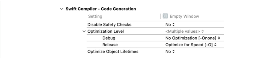
Figure 7-11. How configurations affect build settings
