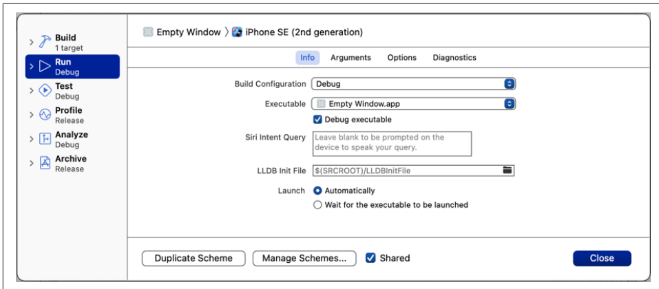
Figure 7-12. The scheme editor
