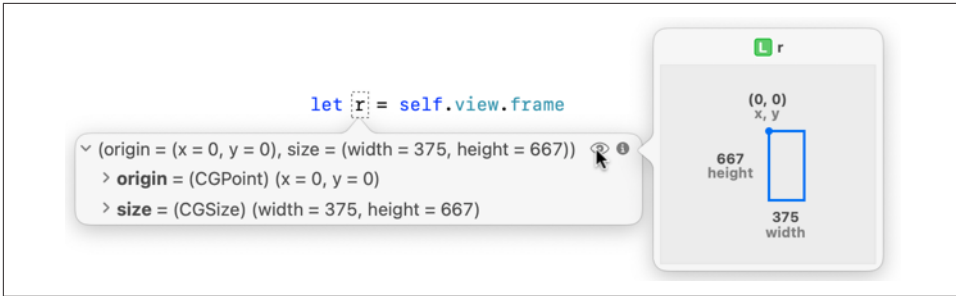
Figure 10-10. A data tip
