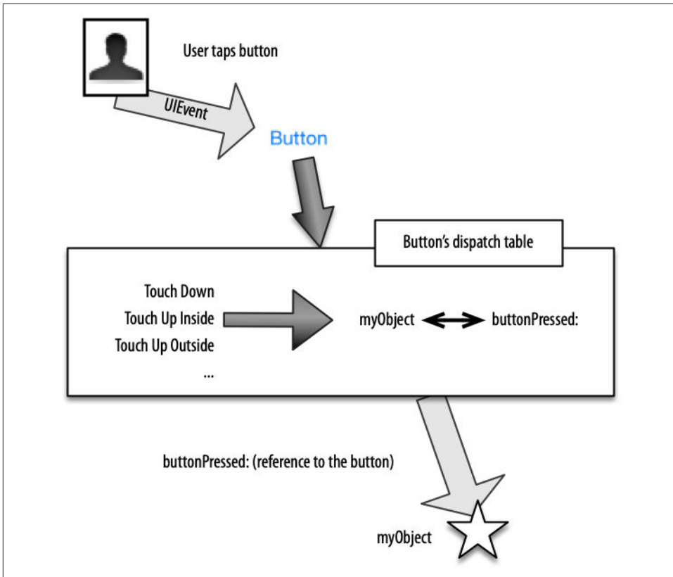
Figure 12-1. The target-action architecture
