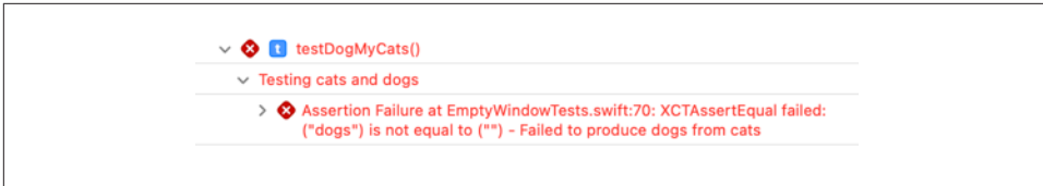
Figure 10-15. A test report with an activity
