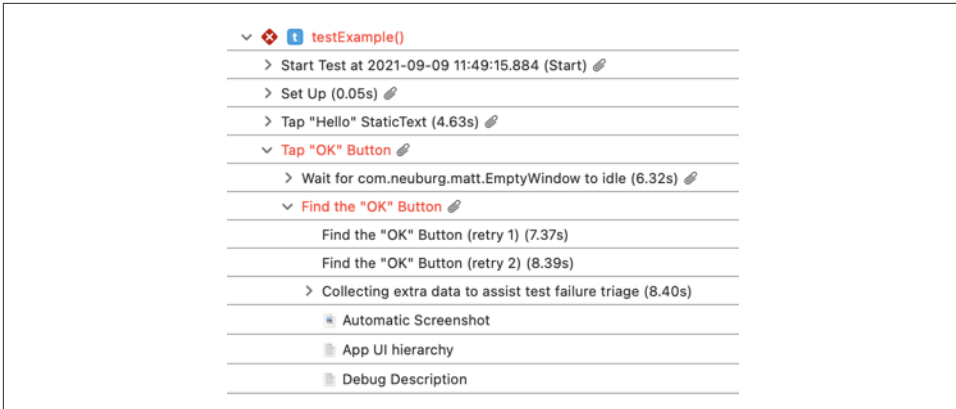
Figure 10-14. The Report navigator displays a failed UI test
