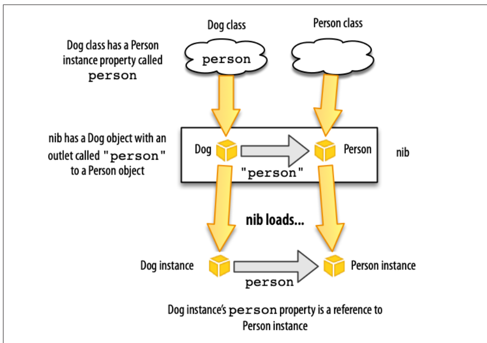
Figure 8-6. How an outlet provides a reference to a nib-instantiated object
