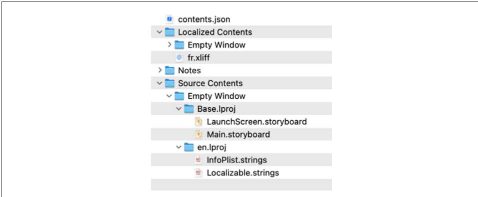
Figure 10-23. An exported xcloc bundle
