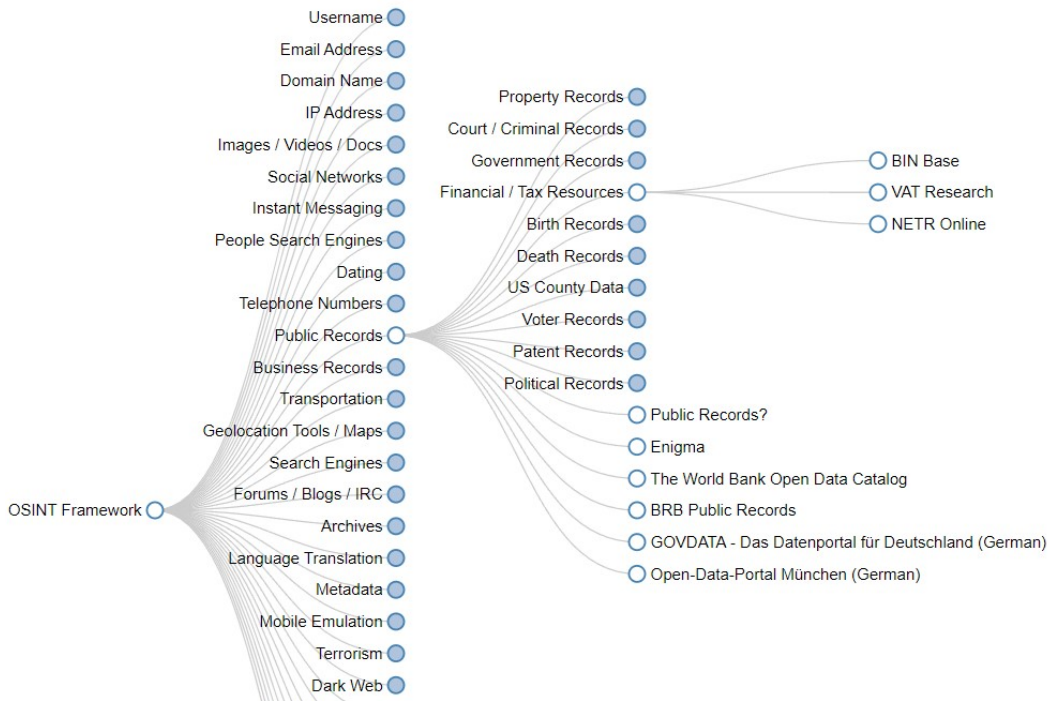
Figure 3.30 – OSINT Framework
