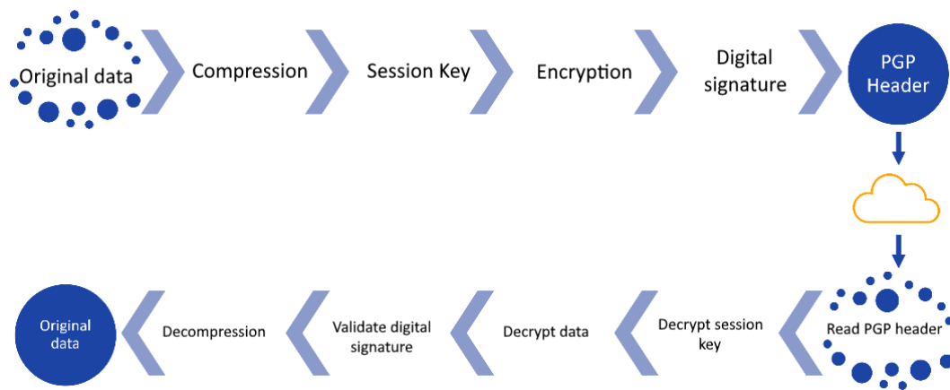
Figure 16.8 – PGP flow
