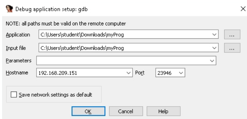
Figure 5-20 IDA debugging options window
