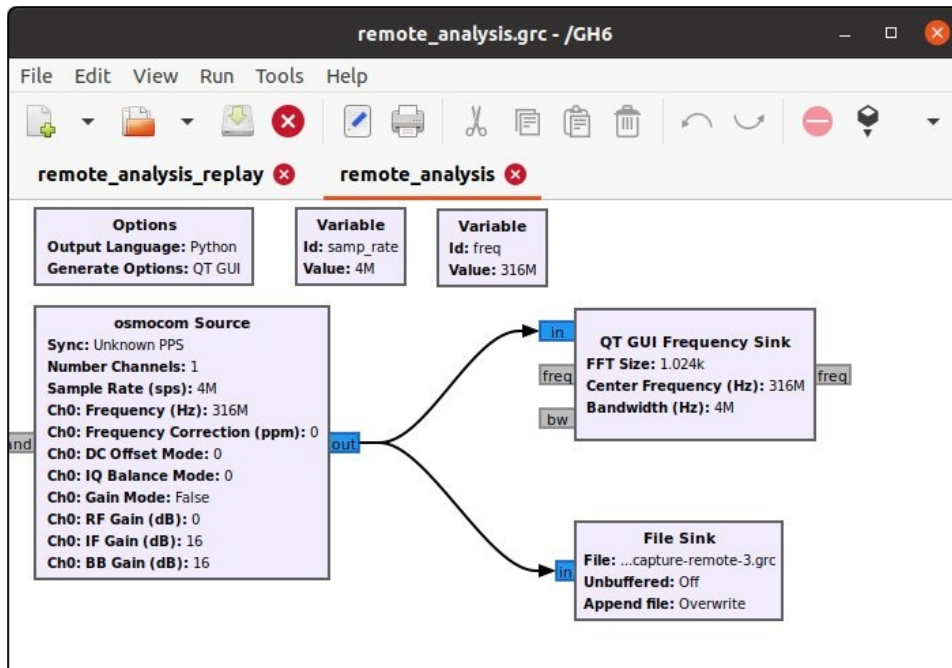
Figure 22-2 Capture flow graph: remote_analysis.grc
