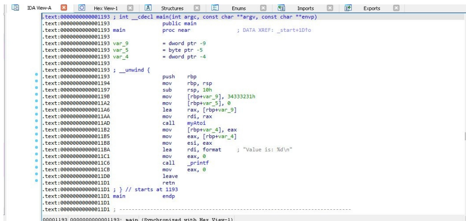
Figure 5-6 IDA Pro text view
