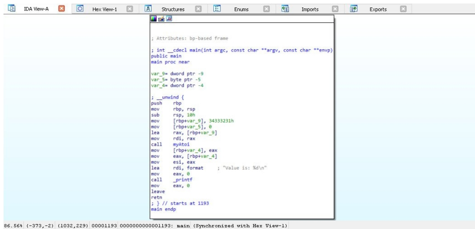
Figure 5-5 IDA Pro graph view
