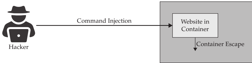
Figure 29-3 Container escape sequence
