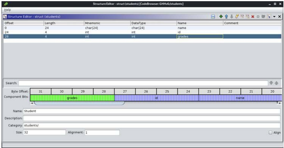
Figure 4-2 Structure Editor window showing the structure to be used
