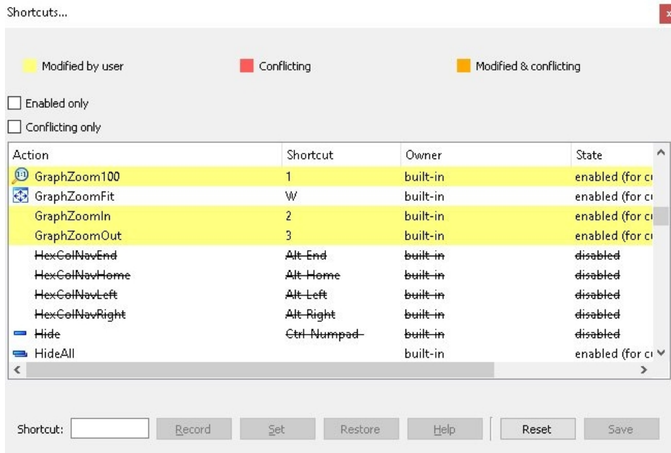
Figure 5-17 Shortcuts menu
