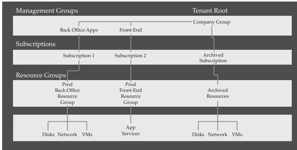
Figure 28-1 Azure subscriptions
