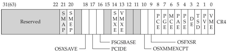
Figure 12-2 CR4 with SMAP bit enabled
