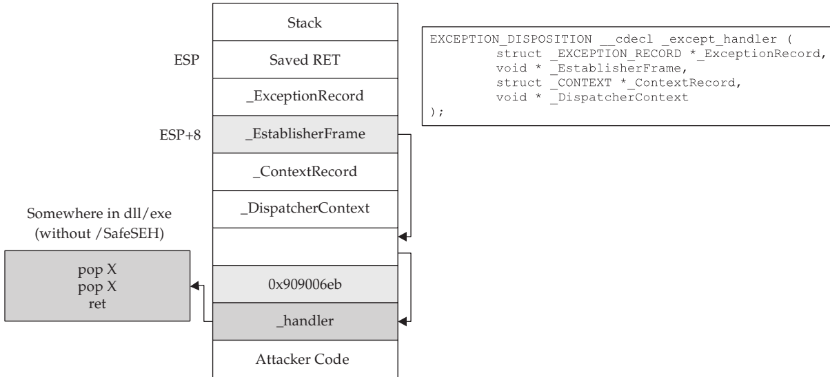
Figure 13-3 The stack when handling an exception
