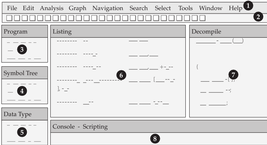
Figure 4-1 The Code Browser's default layout
