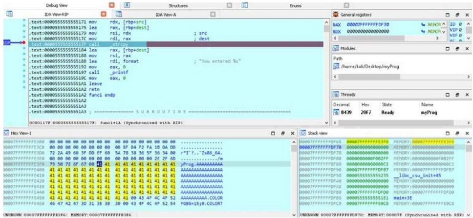
Figure 5-25 Breakpoint on strcpy
