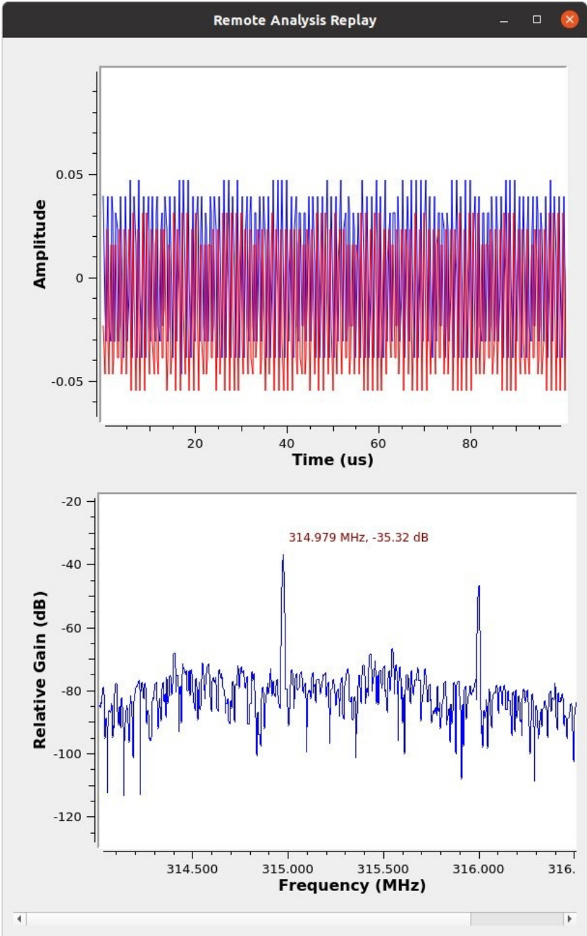
Figure 22-5 Time and frequency plots
