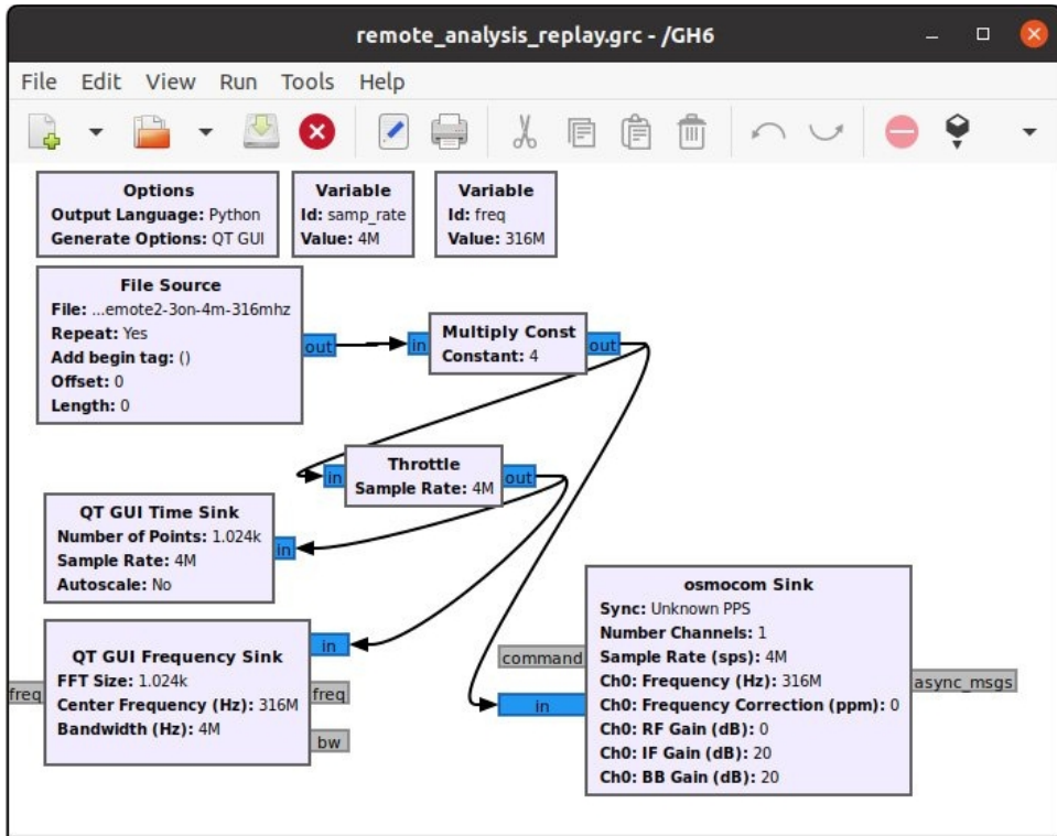
Figure 22-4 Replay flow graph: remote_analysis_replay.grc
