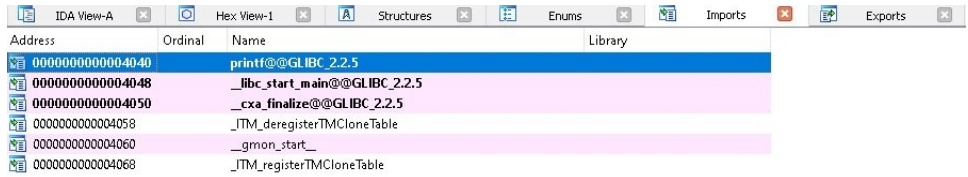
Figure 5-7 IDA Pro Imports tab
