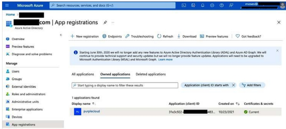
Figure 28-2 App registration page for Azure
