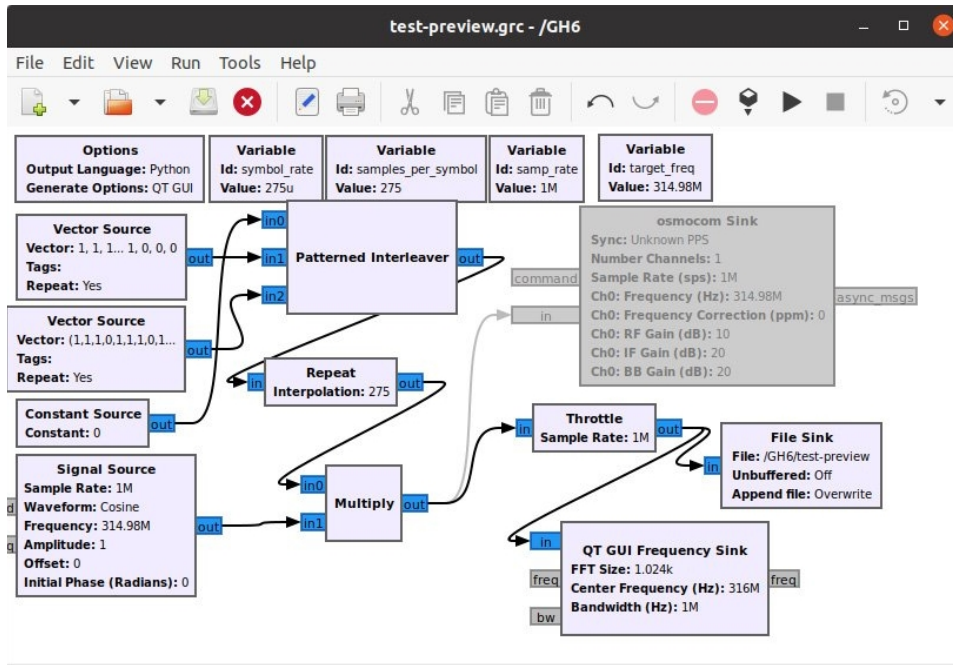
Figure 22-11 Replay flow graph: test-preview.grc
