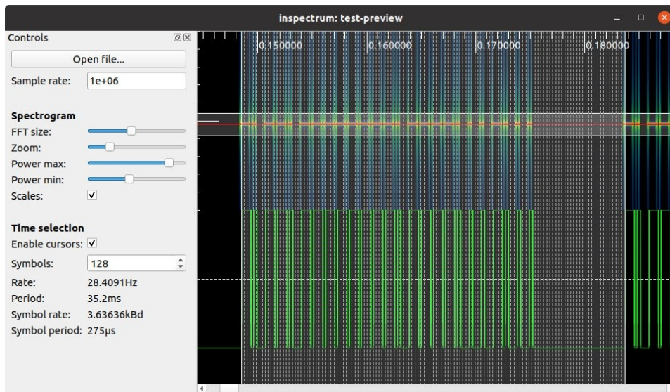
Figure 22-12 Inspectrum diagram of preview
