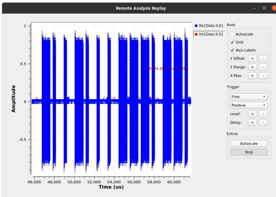
Figure 22-6 Time plot illustrating on-off keying
