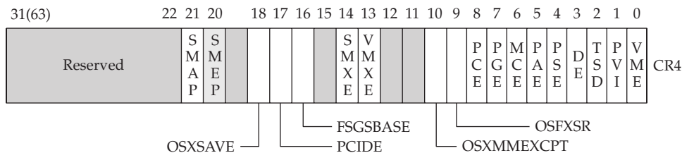
Figure 12-1 CR4 with SMEP bit enabled
