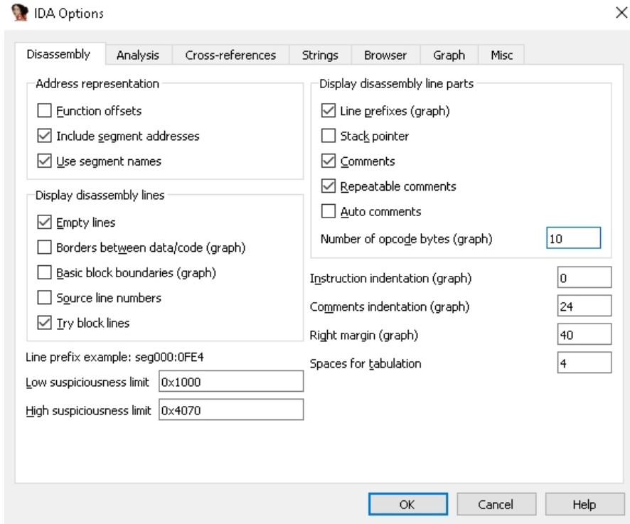
Figure 5-15 General Options menu
