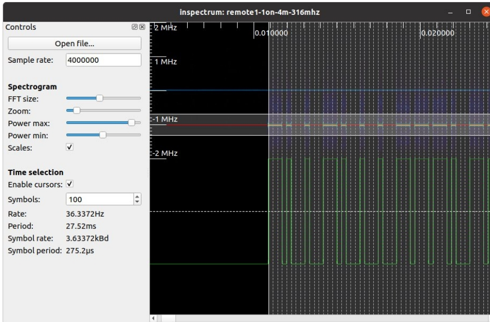
Figure 22-9 Amplitude plot
