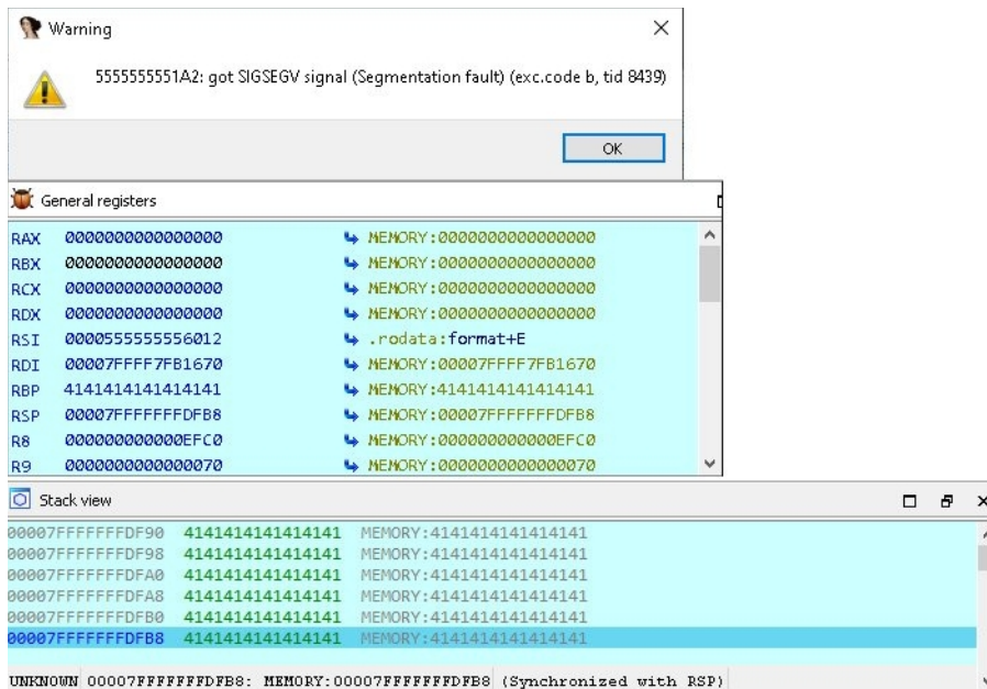
Figure 5-26 Crash caught in IDA Pro Debugger
