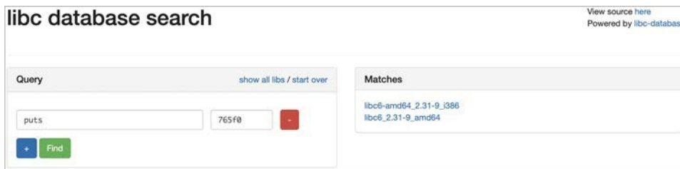
Figure 3-1 The libc-database web wrapper at https://libc.blukat.me
