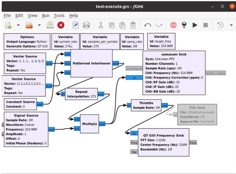
Figure 22-13 Final execute flow graph: test-execute.grc
