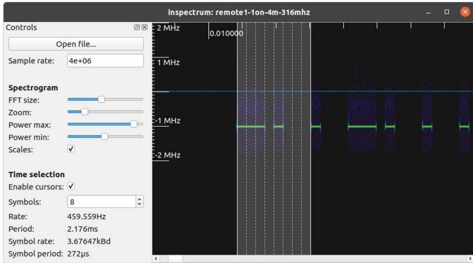
Figure 22-8 Measuring the symbols
