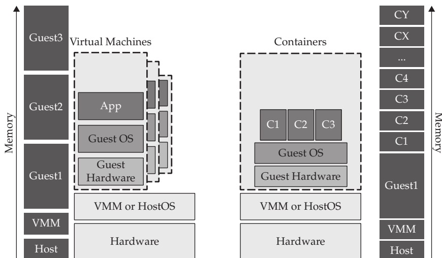
Figure 29-2 Containers vs. virtual machines
