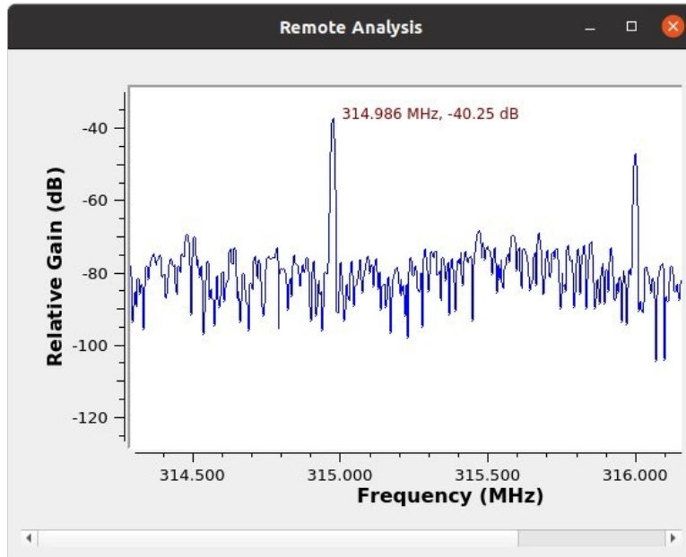
Figure 22-3 Captured signal
