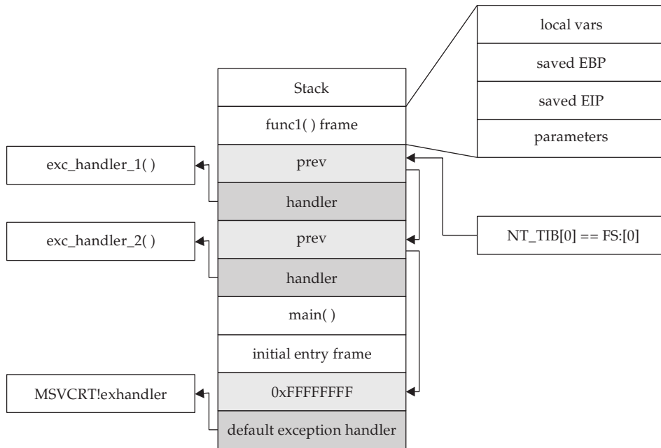
Figure 13-2 Structured Exception Handling (SEH)
