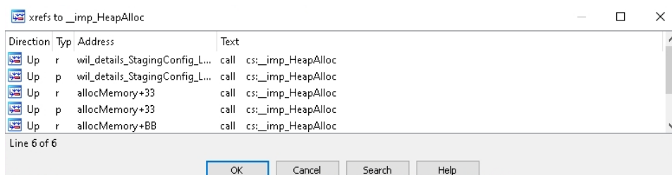
Figure 5-11 Cross-references to HeapAlloc
