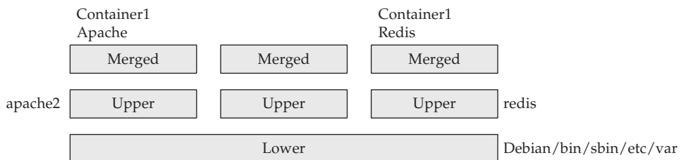
Figure 29-1 OverlayFS
