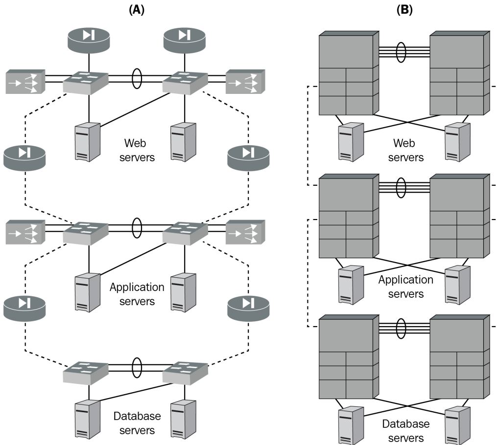
Figure 1.1 – Data center web app architecture
