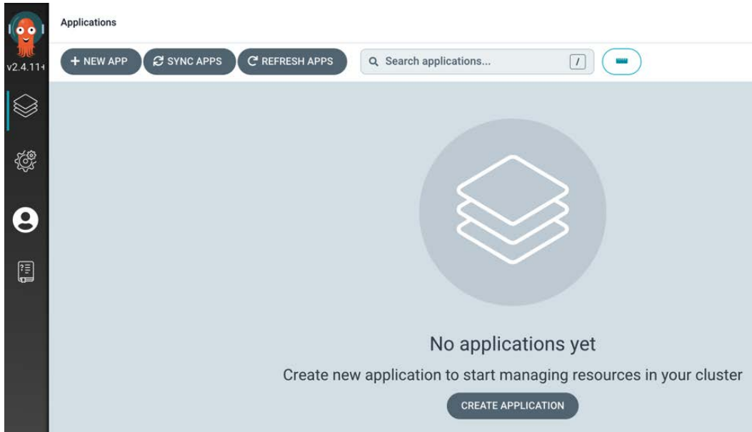
Figure 6.10 – ArgoCD portal
