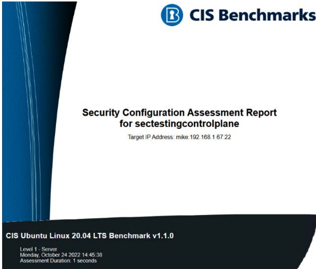
Figure 8.16 – Benchmark report
