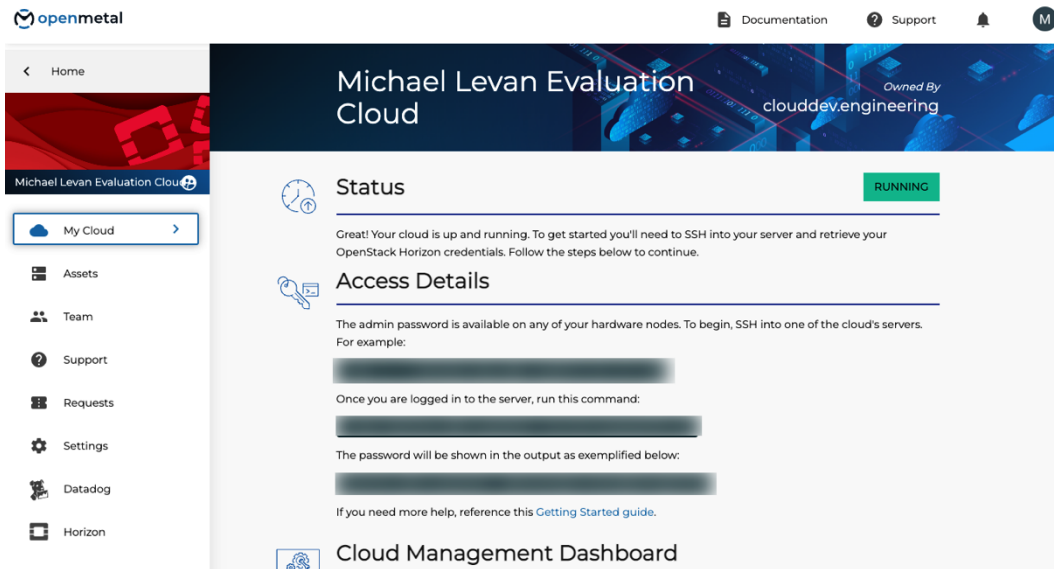
Figure 4.6 – OpenMetal dashboard
