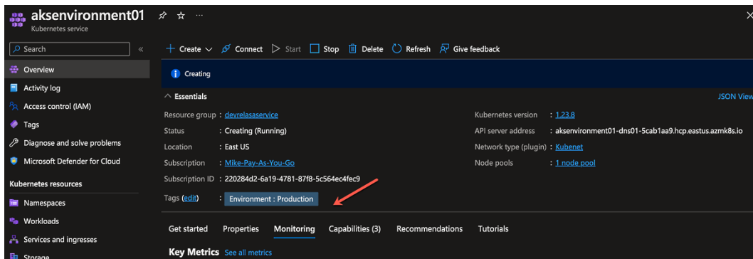
Figure 7.2 – AKS Monitoring
