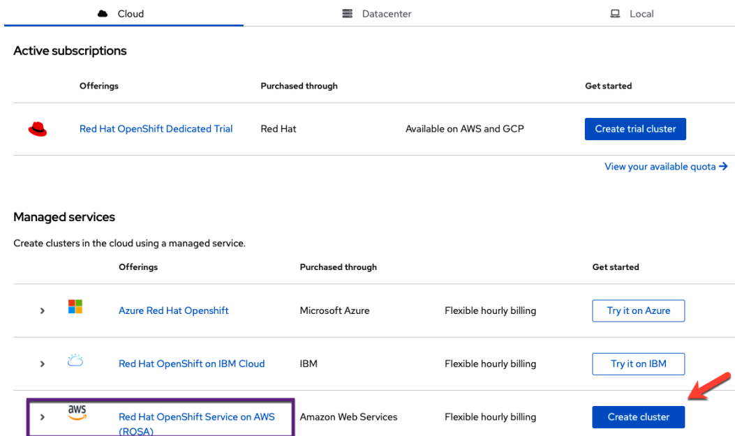
Figure 3.20 – AWS ROSA
