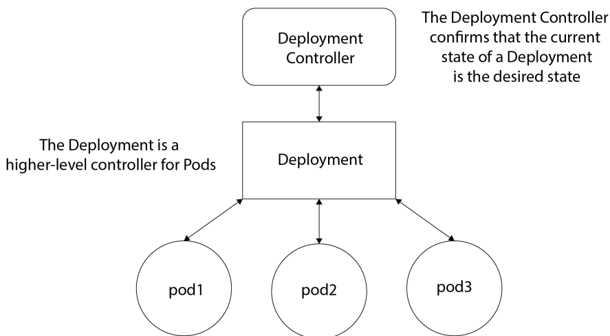
Figure 5.1 – Controllers
