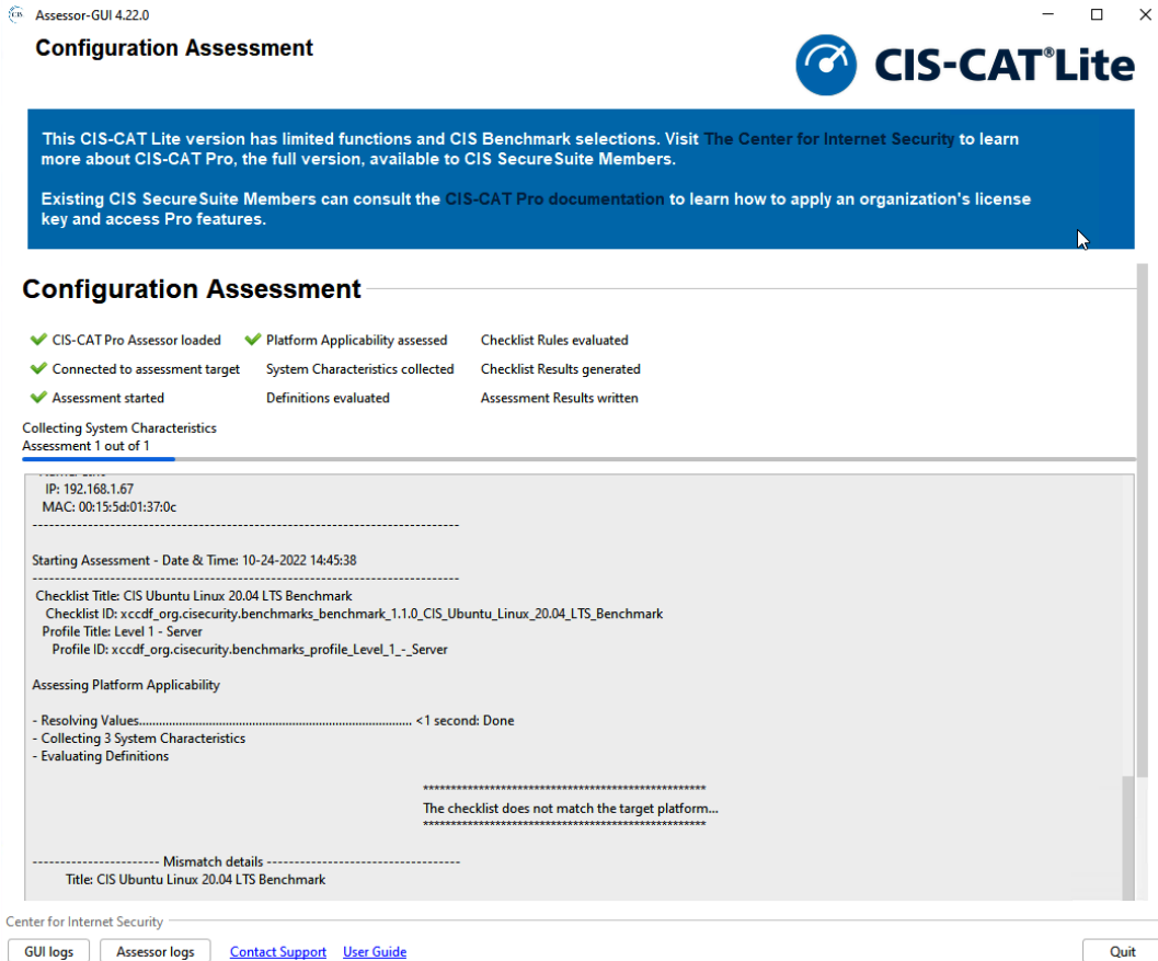
Figure 8.15 – Assessment results
