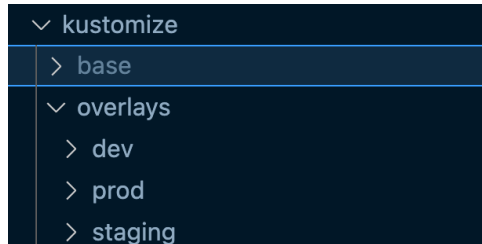
Figure 6.4 – Base configuration
