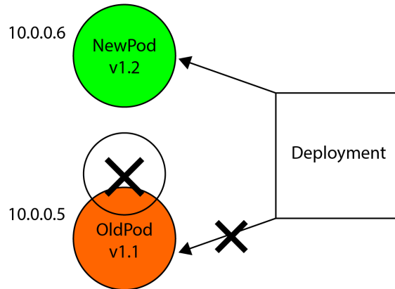
Figure 5.3 – Rolling update
