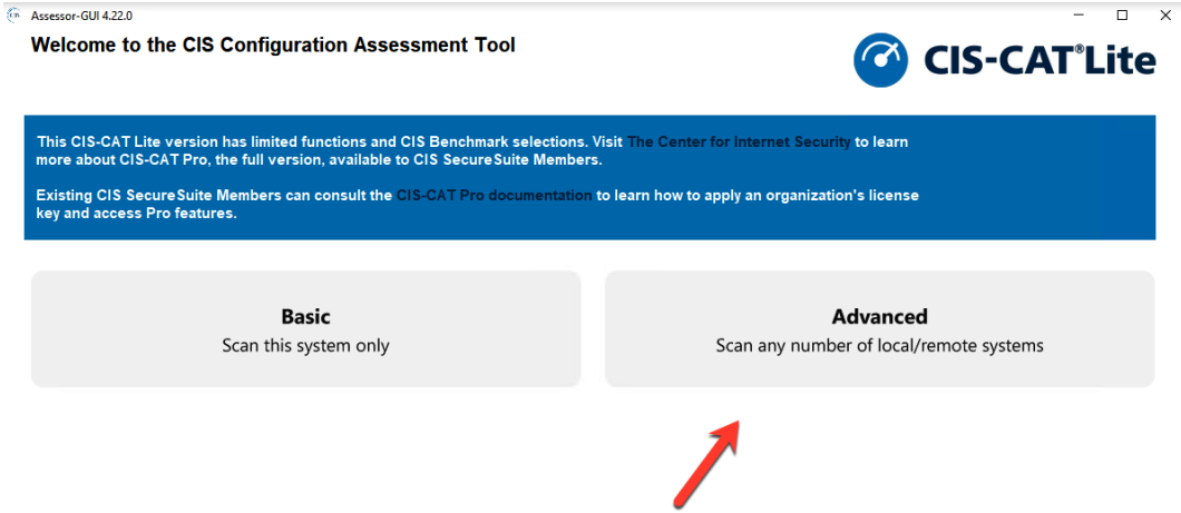
Figure 8.8 – Advanced option
