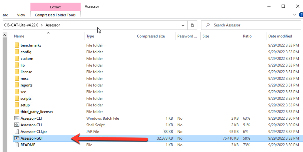
Figure 8.7 – GUI binary
