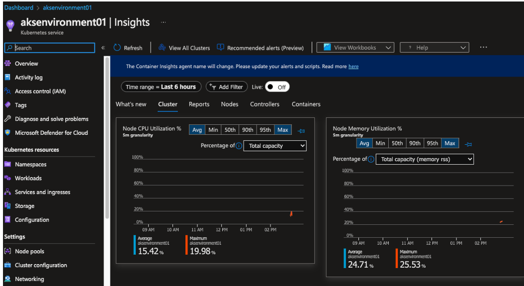
Figure 7.16 – Insights data
