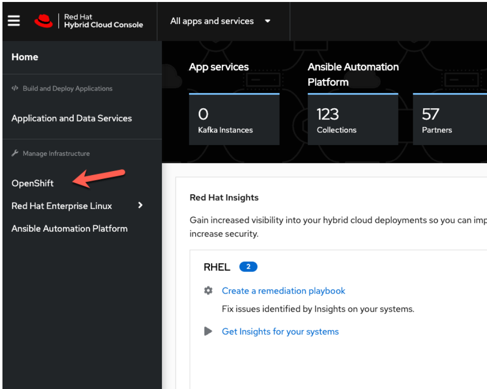
Figure 3.18 – OpenShift manager
