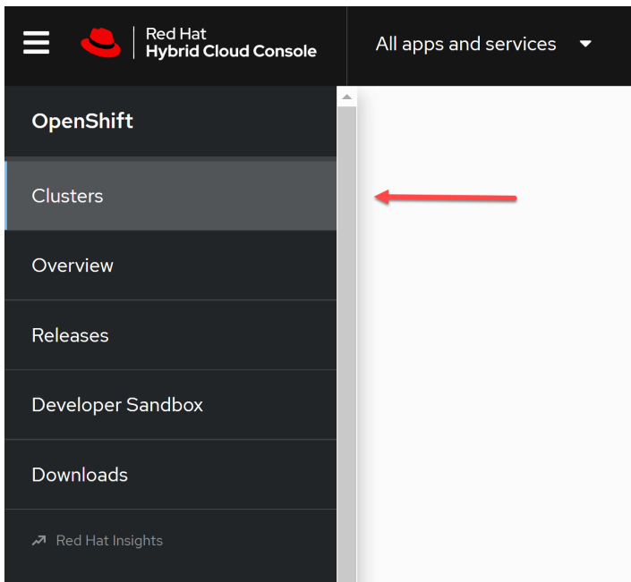
Figure 3.13 – Clusters
