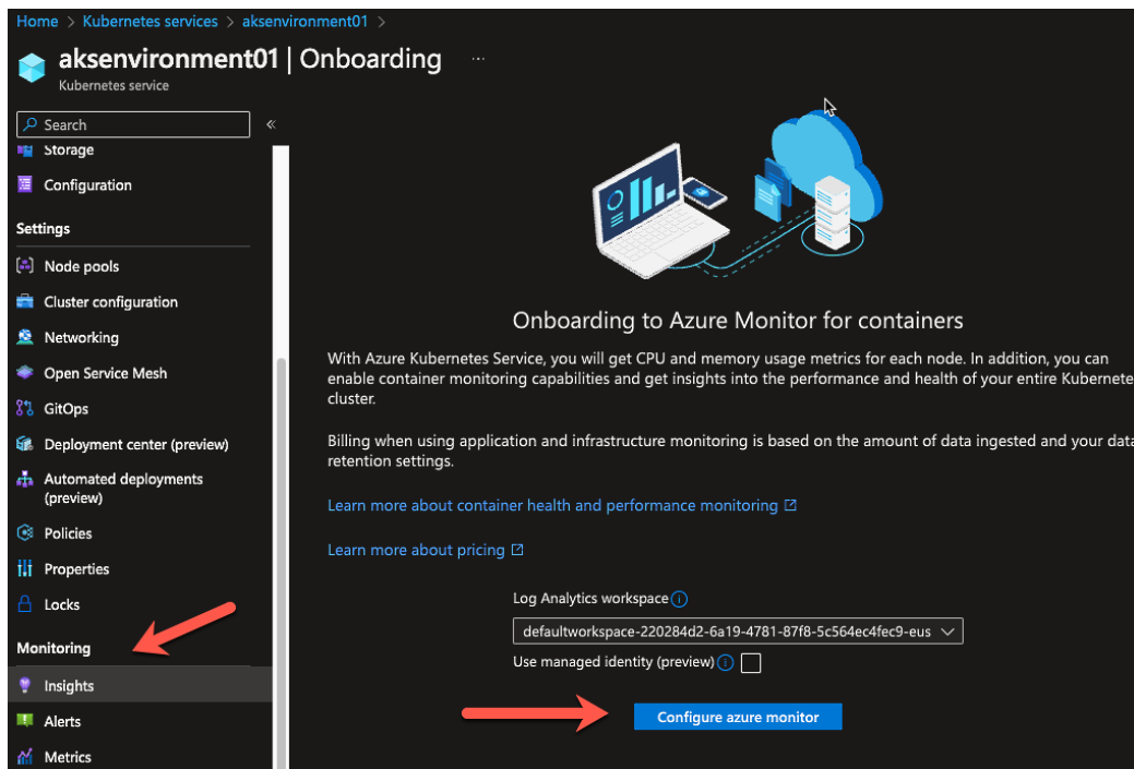
Figure 7.15 – Azure Insights
