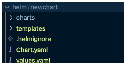
Figure 6.1 – Helm chart
