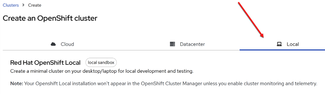
Figure 3.14 – Local cluster
