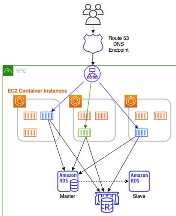
Figure 13.6 – Using an ECS service update for a blue/green deployment
