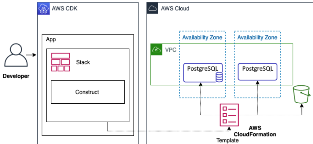
Figure 7.12 – CDK workflow
