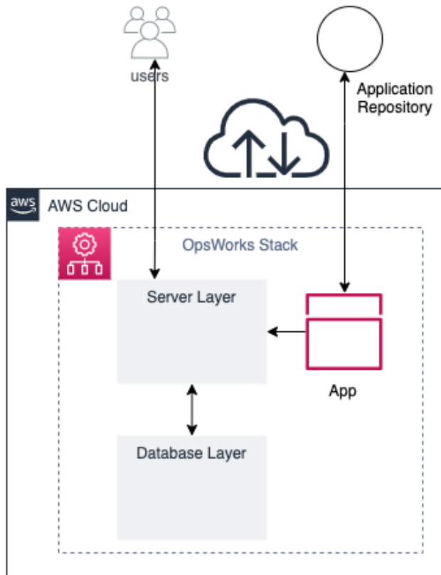
Figure 10.1 – OpsWorks serving users from an app
