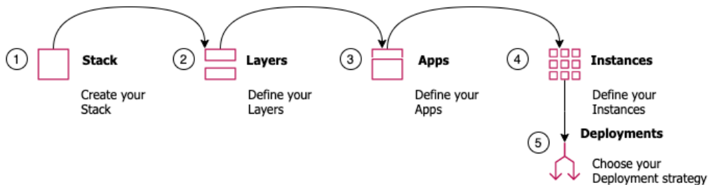
Figure 10.2 – Overview of how OpsWorks operates
