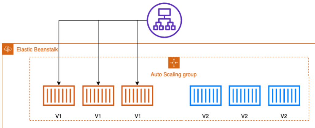
Figure 11.6 – Immutable deployment during deployment
