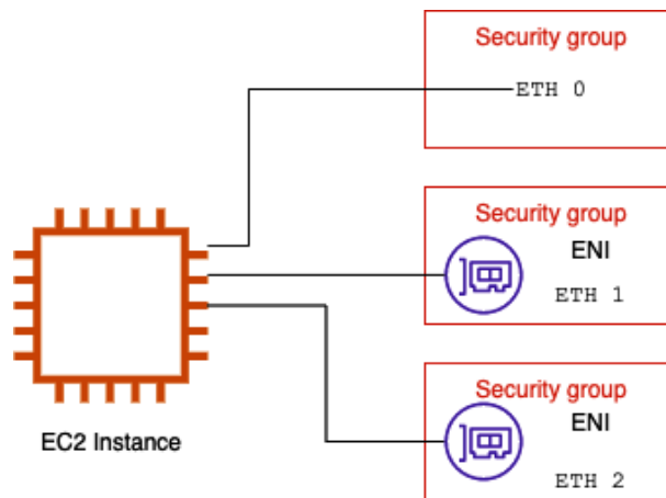
Figure 2.6 – ENIs in separate security groups
