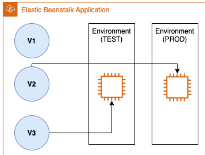
Figure 11.3 – Application versions can only be deployed to a single environment
