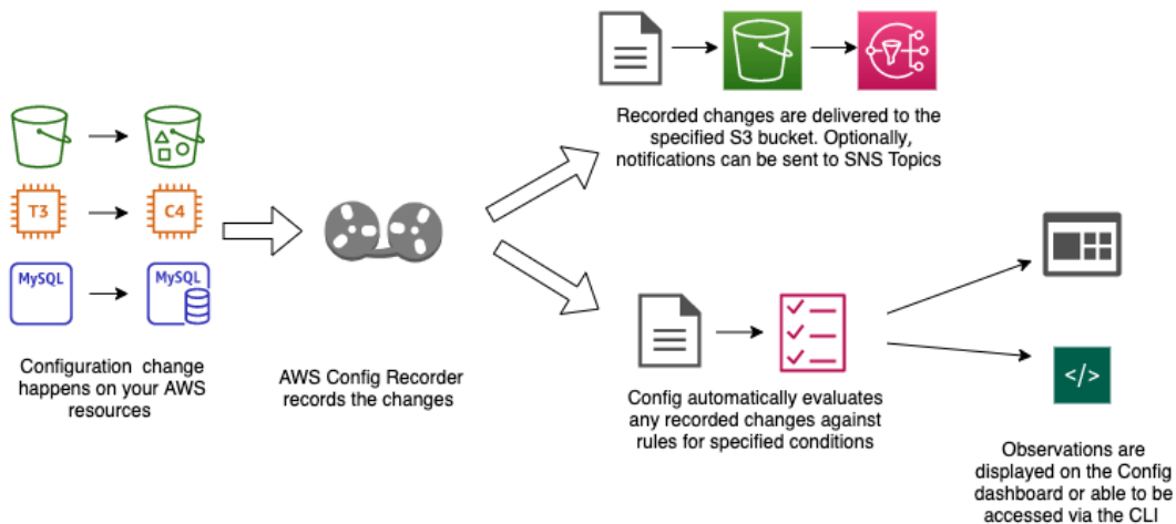
Figure 20.19 – Understanding the workflow of AWS Config
