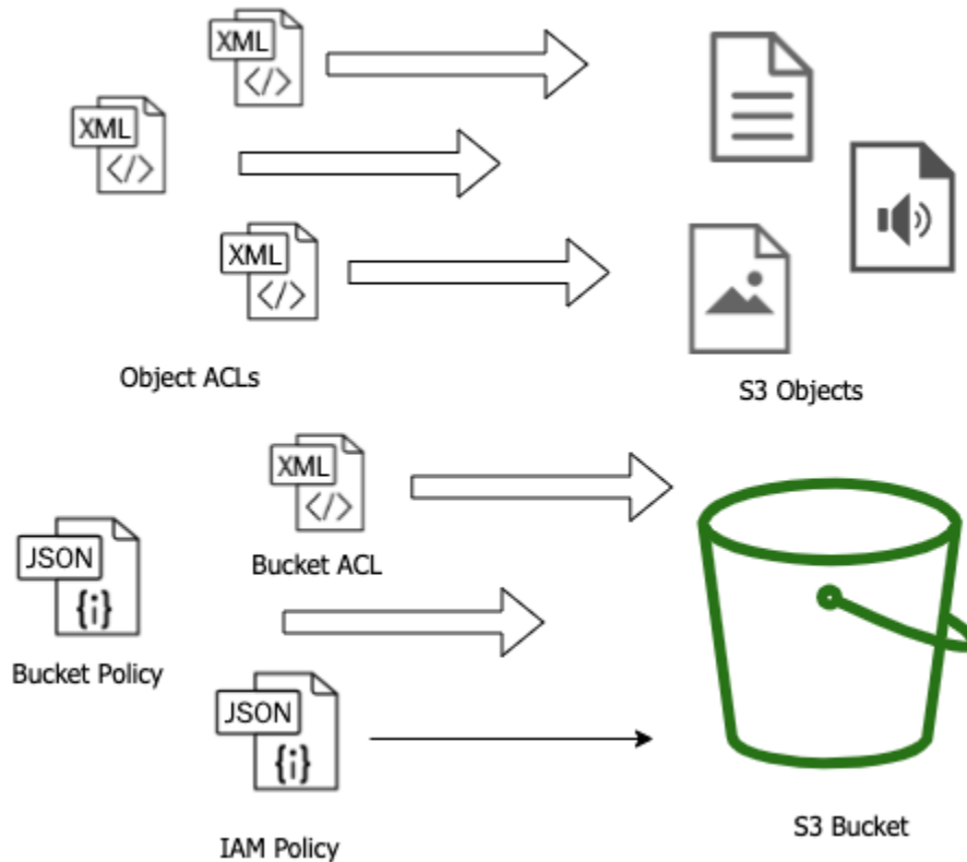
Figure 4.7 – S3 resource versus user-based policies
