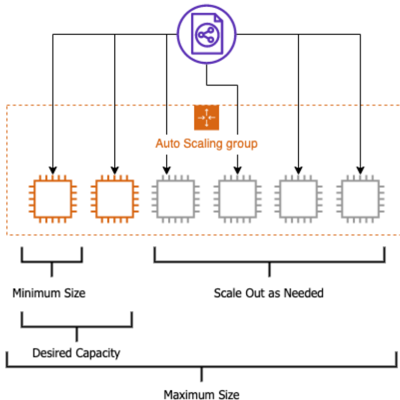
Figure 18.2 – ASG visualization
