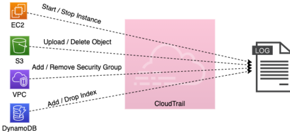
Figure 16.1 – The flow of actions to logs via the CloudTrail service
