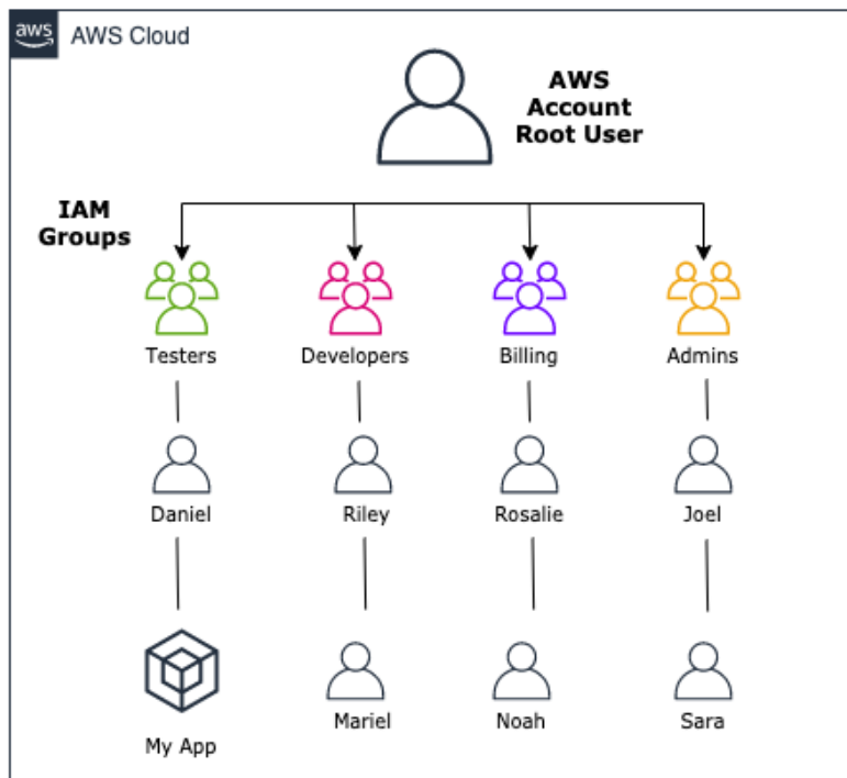
Figure 3.5 – IAM users and groups
