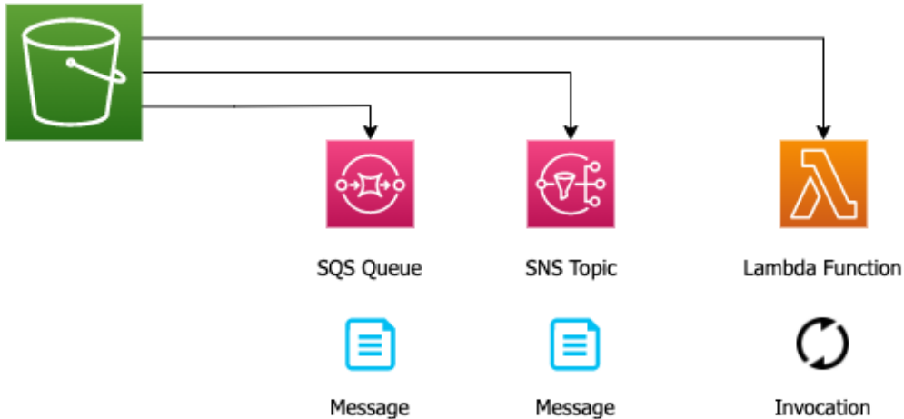
Figure 4.8 – S3 Event Flow
