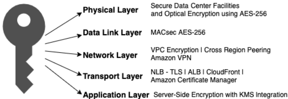
Figure 19.1 – The AWS cryptography stack
