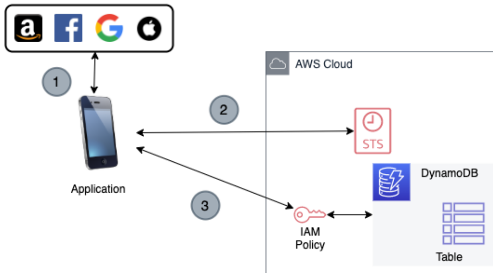
Figure 5.6 – Web Identity Federation to a DynamoDB table
