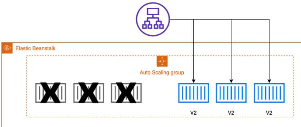
Figure 11.7 – Immutable deployment after deployment
