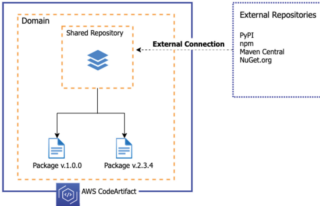
Figure 6.2 – AWS CodeArtifact with connection to external repositories
