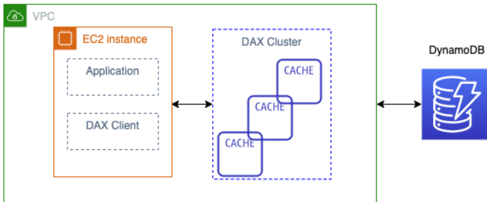
Figure 5.5 – DAX example architecture
