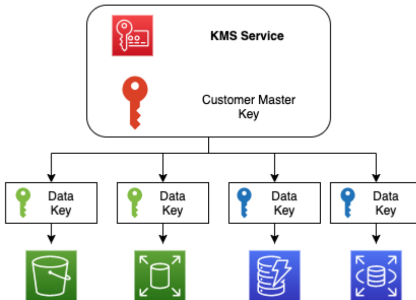
Figure 19.2 – Master and data keys in AWS KMS
