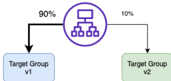
Figure 13.1 – An Application Load Balancer deploying traffic to two versions of an application at once using target groups
