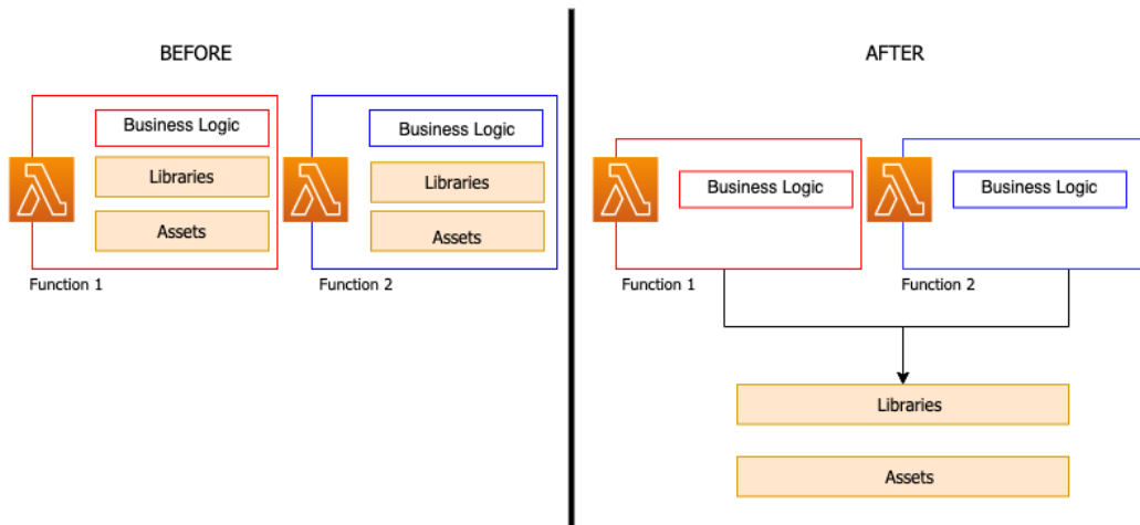
Figure 12.7 – Lambda functions with and without layers
