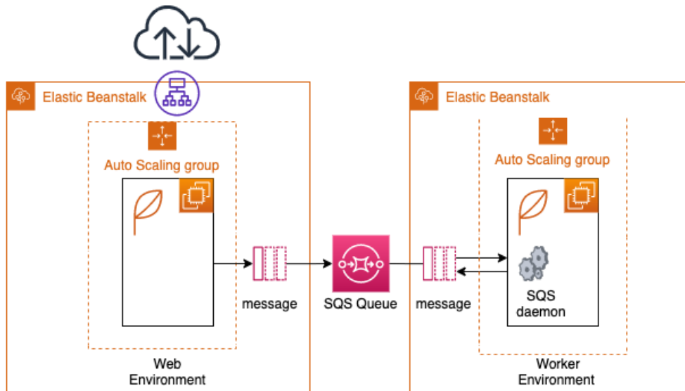
Figure 11.2 – Web server and worker environments in Elastic Beanstalk
