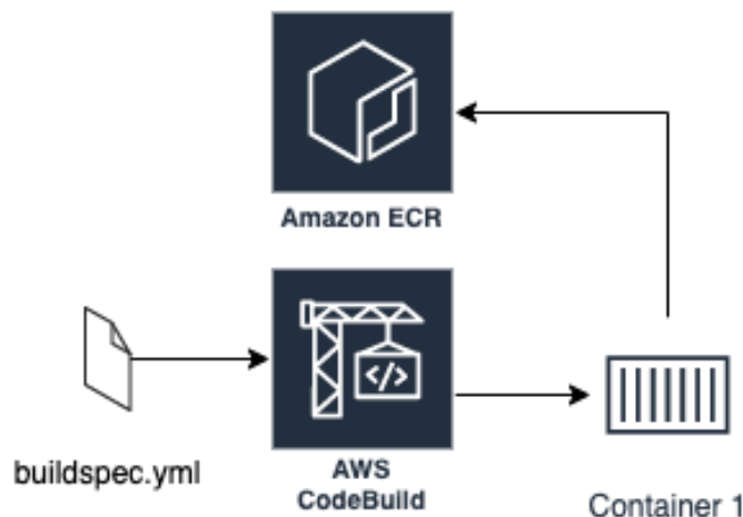
Figure 8.19 – Layout of what the example CodeBuild job does
