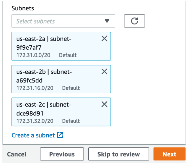
Figure 18.6 – Adding the three subnets from the default VPC to the ASG
