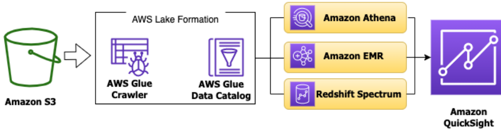
Figure 17.2 – Connecting Amazon QuickSight to a data lake in AWS
