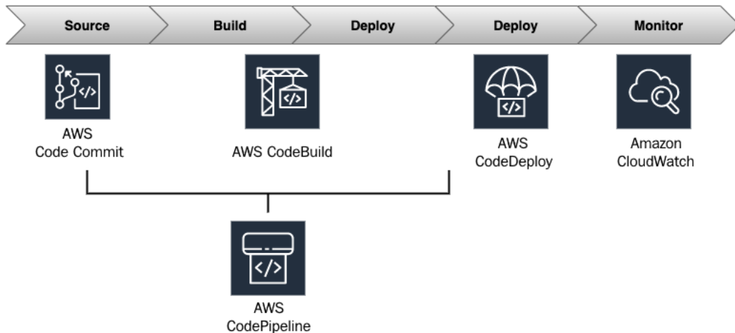
Figure 6.3 – AWS tools used in CI/CD
