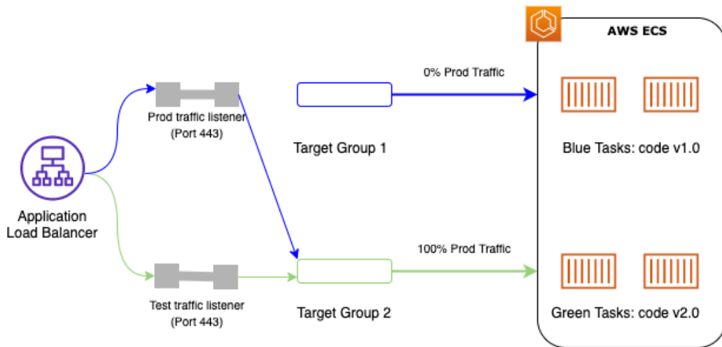
Figure 13.2 – Switching from Target Group 1 to Target Group 2 in ECS using an ALB
