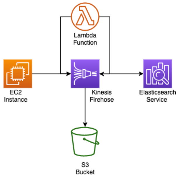
Figure 17.12 – Kinesis Firehose inserting logs into S3 and the Elasticsearch service simultaneously
