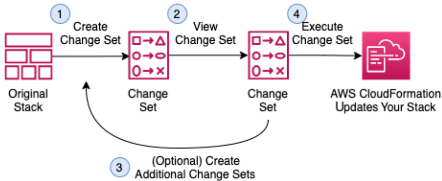
Figure 7.4 – CloudFormation change sets
