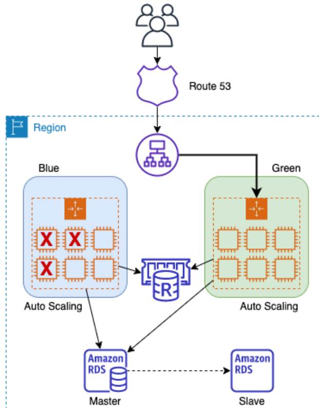
Figure 13.4 – Deploying blue/green environments by swapping Auto Scaling groups
