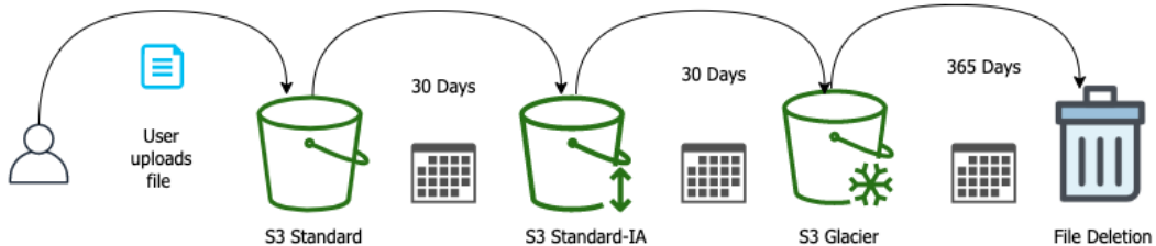
Figure 4.3 – An example S3 lifecycle policy
