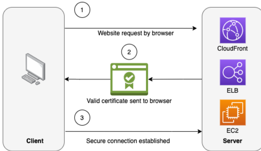
Figure 19.7 – How SSL/TLS works from browser to client
