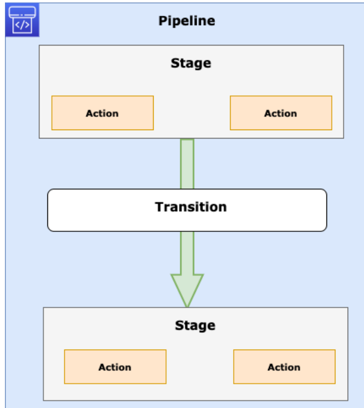
Figure 9.11 – CodePipeline transition representation
