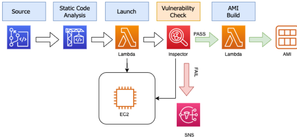
Figure 21.2 – Inspector in a CI/CD pipeline
