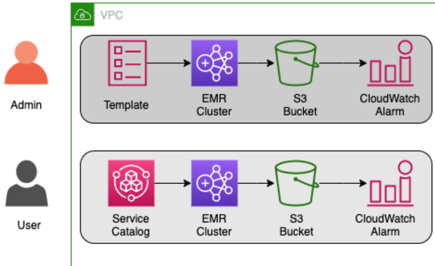
Figure 7.11 – Service Catalog workflows
