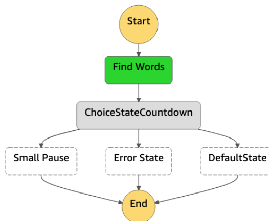
Figure 12.11 – The graphical view of the state machine, as generated by AWS
