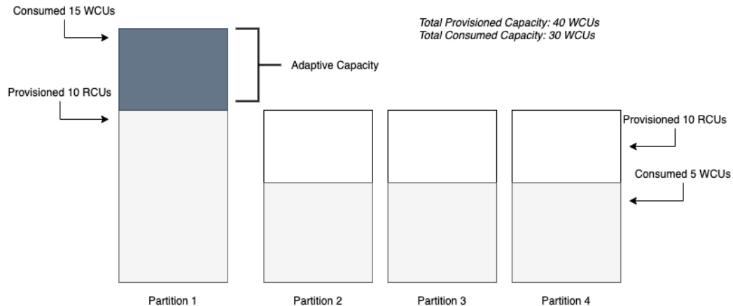
Figure 5.4 – Adaptive capacity example
