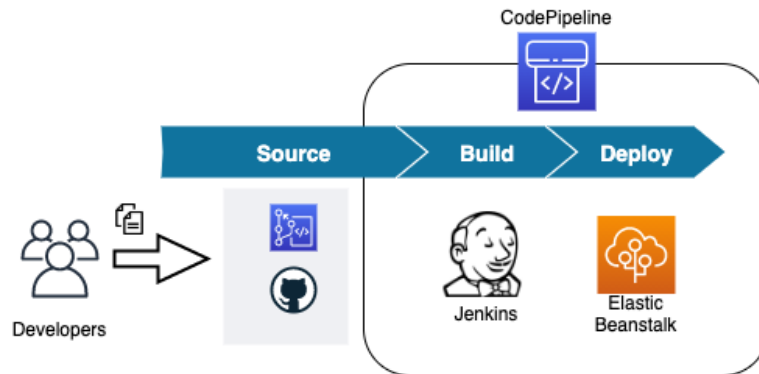
Figure 9.12 – Using Jenkins in conjunction with CodePipeline
