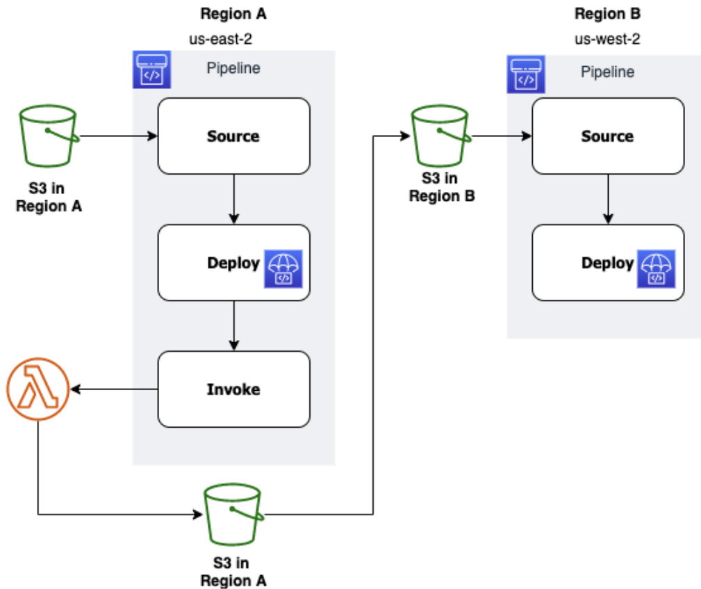
Figure 9.13 – Using CodePipeline and CodeDeploy to deploy to multiple regions
