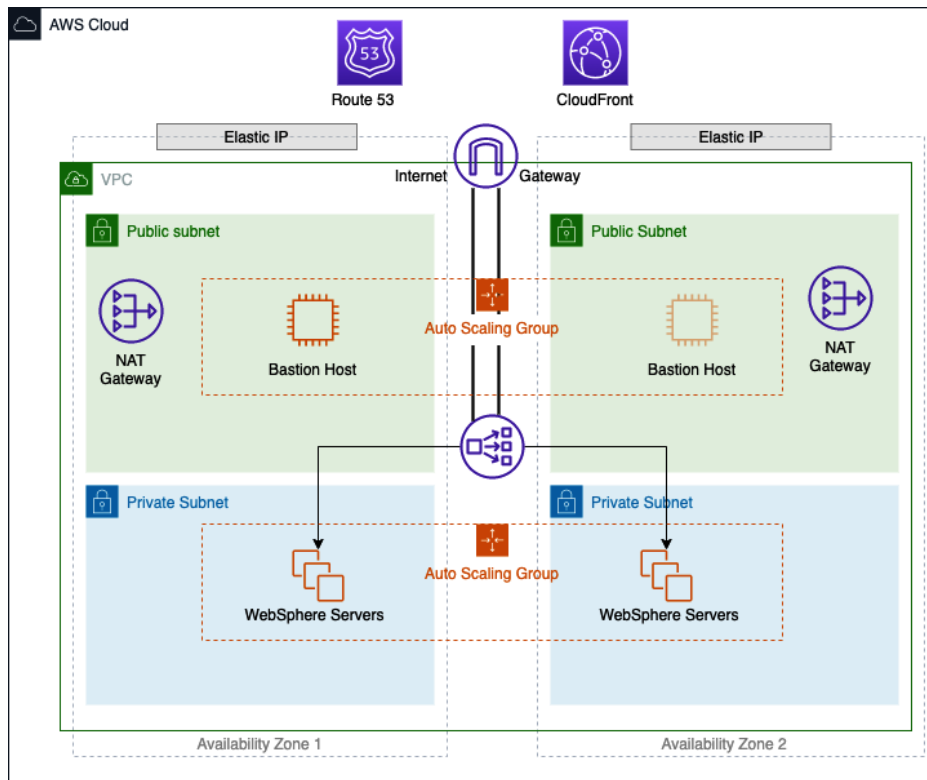
Figure 2.5 – EC2 in a real-world architecture
