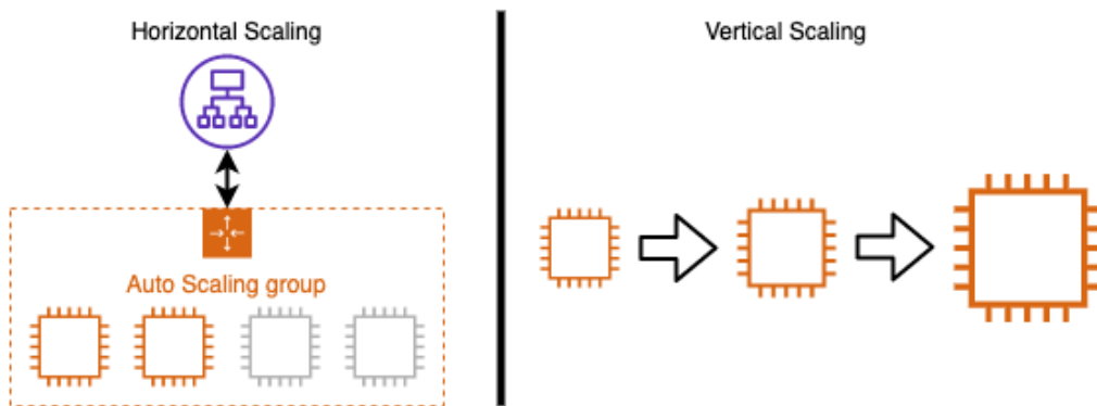
Figure 18.1 – Horizontal scaling versus vertical scaling
