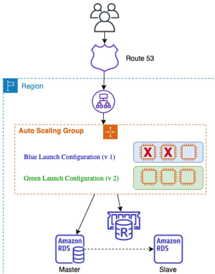
Figure 13.5 – Deploying blue/green environments by swapping launch configurations
