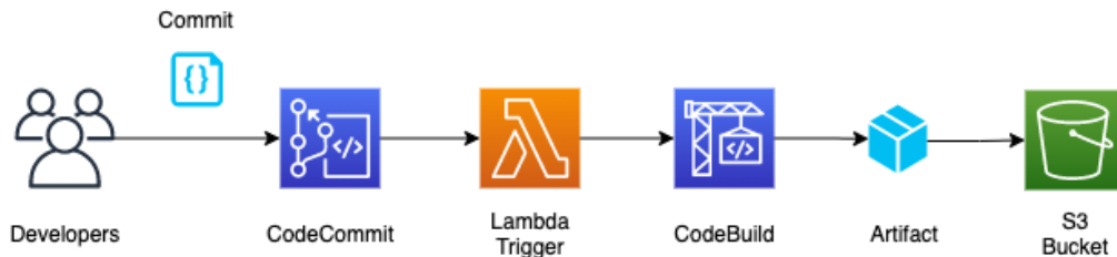
Figure 8.23 – Triggering a CodeBuild job from CodeCommit
