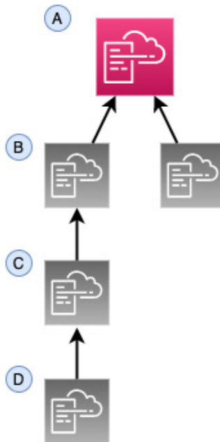
Figure 7.9 – CloudFormation nested stacks
