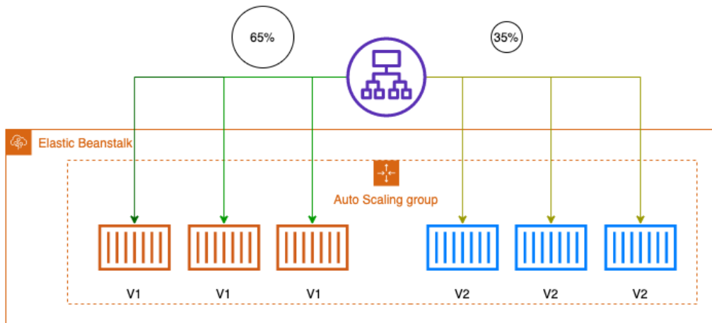
Figure 11.8 – Traffic-splitting deployment showing the percent of traffic
