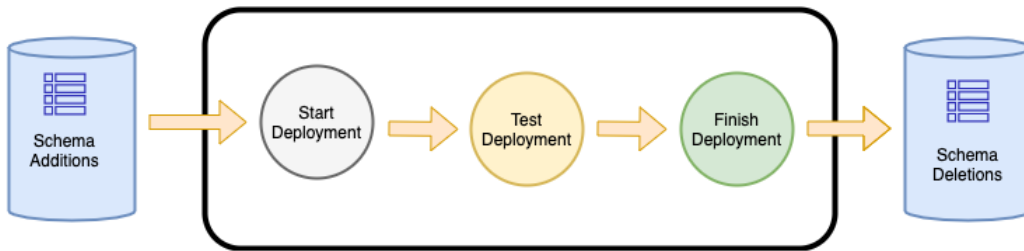
Figure 13.9 – The process for making database schema changes during blue/green deployments
