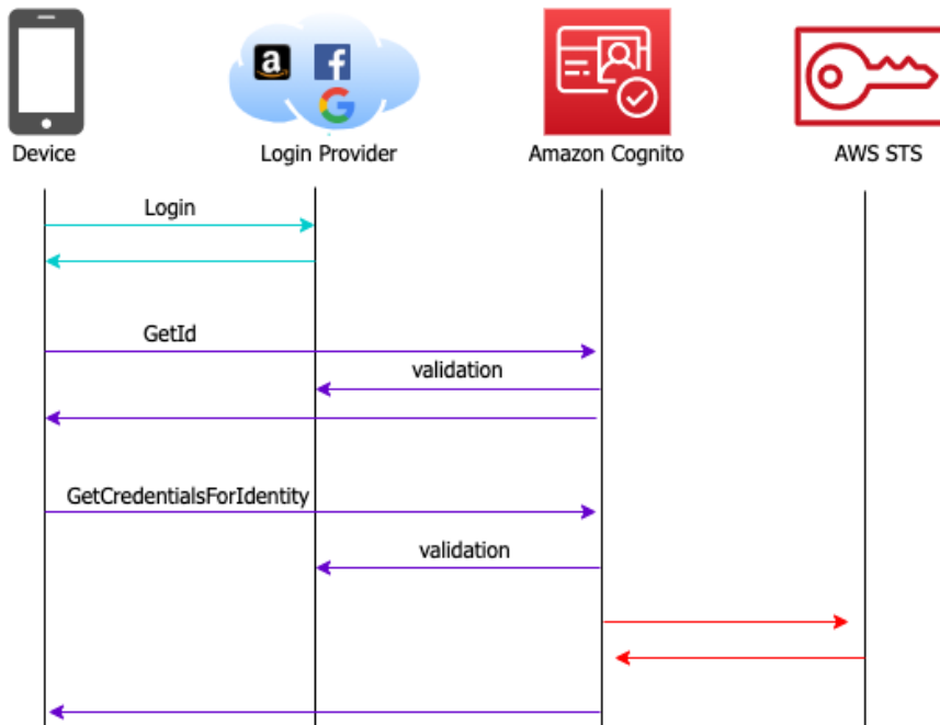
Figure 3.19 – Cognito identity pool authorization flow
