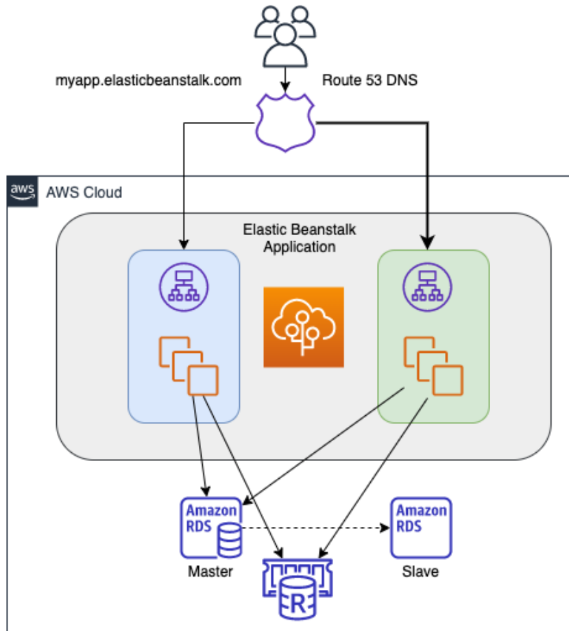
Figure 13.7 – A blue/green deployment by swapping an Elastic Beanstalk application
