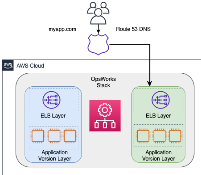
Figure 13.8 – Cloning an OpsWorks stack
