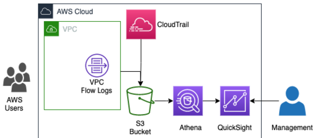
Figure 17.1 – A flow of logs to Athena and AWS QuickSight to create visualizations
