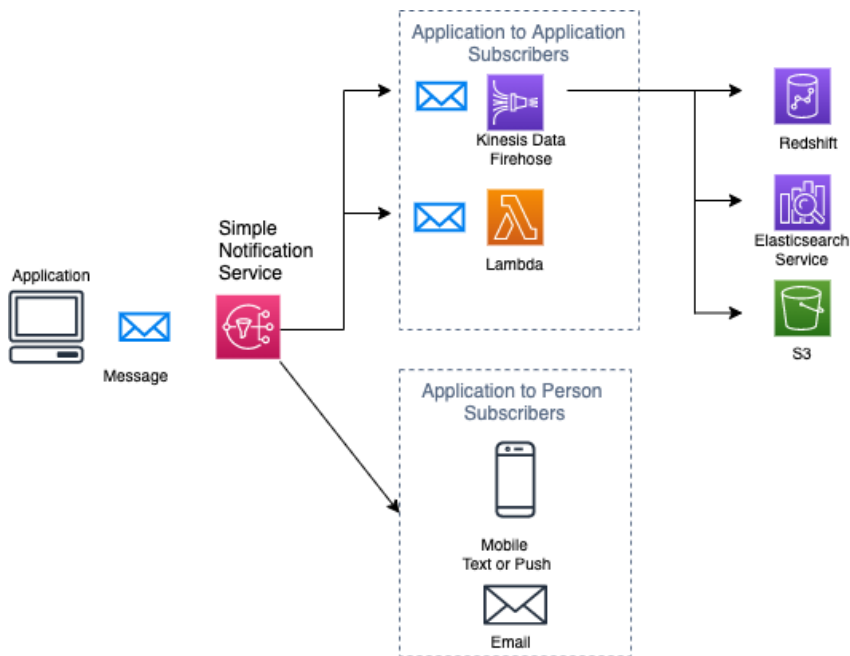
Figure 2.12 – SNS fanout
