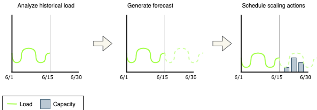
Figure 18.3 – How predictive scaling works to schedule resources in Auto Scaling
