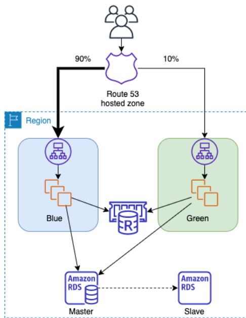
Figure 13.3 – Showing blue/green deployment using Route 53-hosted zones
