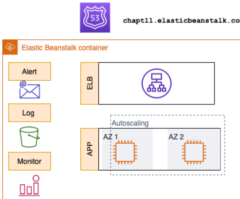
Figure 11.4 – A closer look at an Elastic Beanstalk configuration
