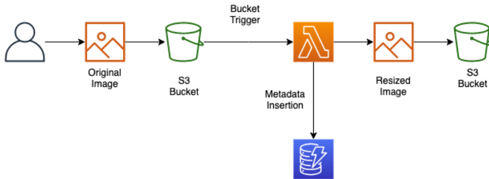
Figure 12.5 – The flow of an image being uploaded to an S3 bucket that triggers a Lambda function for image resizing
