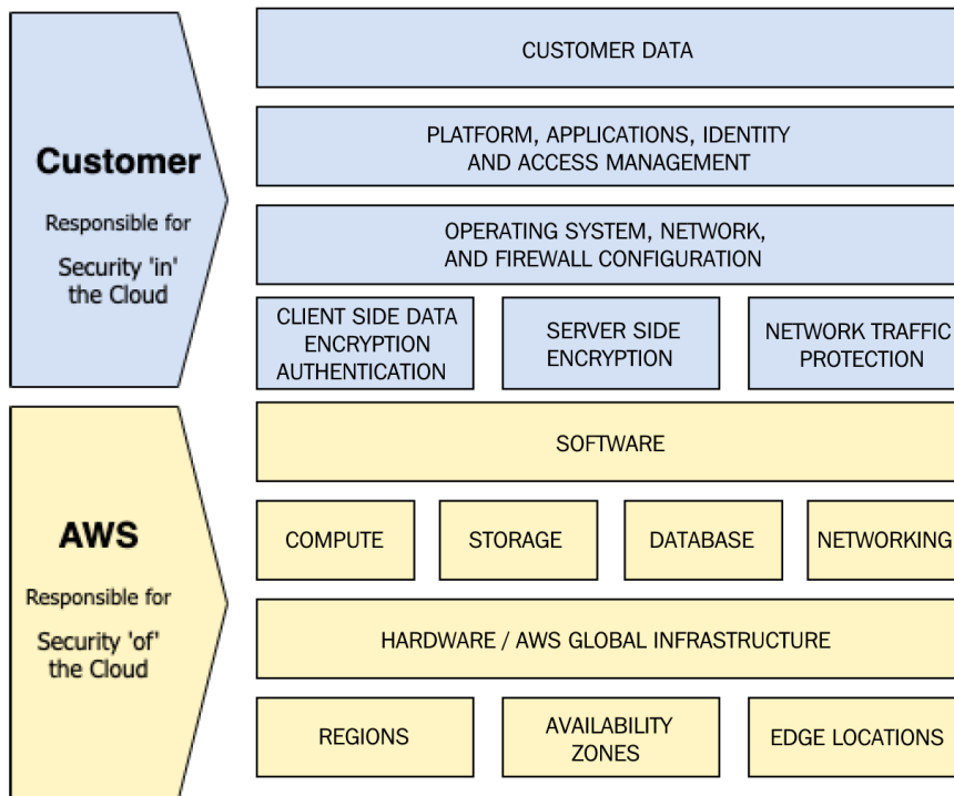
Figure 1.3 – The AWS shared responsibility model
