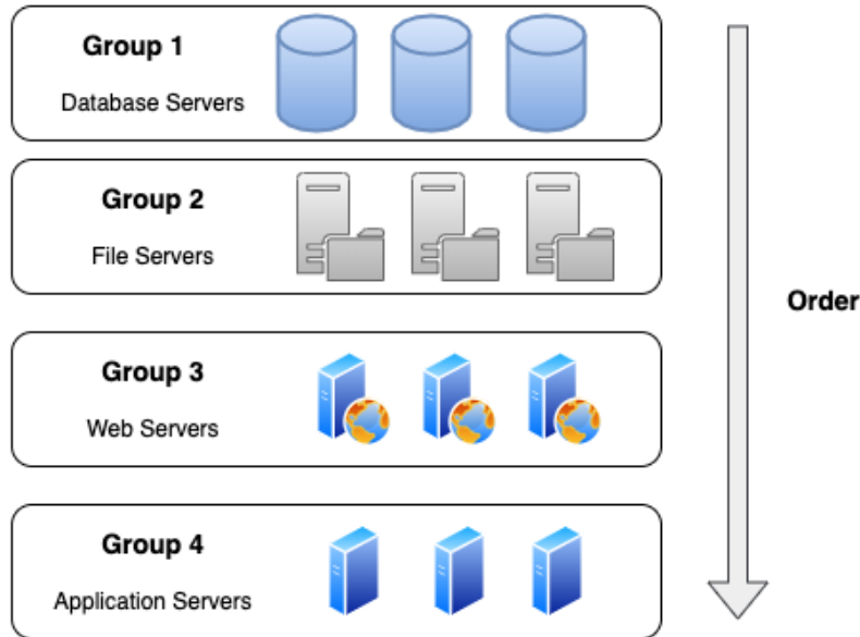
Figure 22.3 – An example of a launch order for an SMS job
