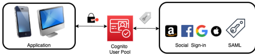
Figure 3.18 – Cognito user pool authentication
