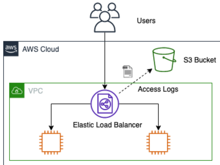
Figure 16.3 – The flow of the access logs from an Elastic Load Balancer to an S3 bucket
