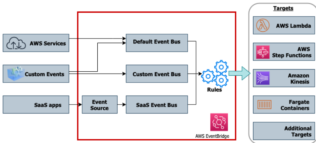
Figure 15.11 – AWS EventBridge flow from events to targets
