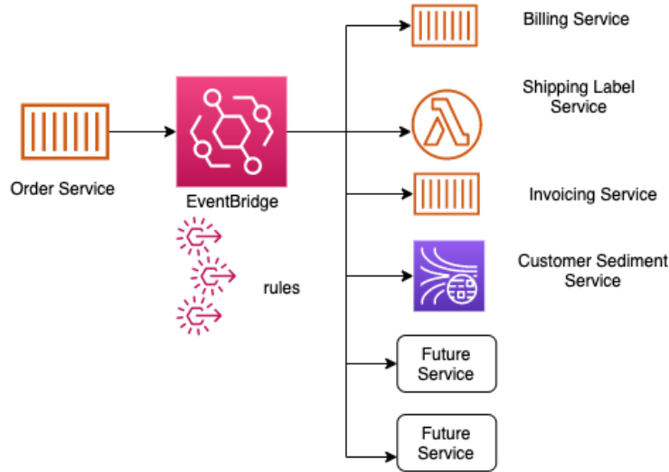
Figure 15.13 – A single service using EventBridge and custom rules to push to multiple targets
