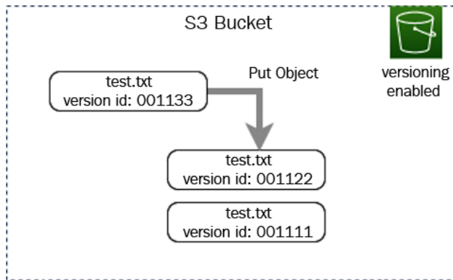
Figure 4.19 – An S3 bucket with versioning enabled showing version ids
