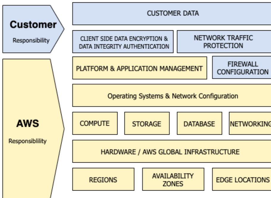
Figure 3.2 – AWS Shared Responsibility Model: container services
