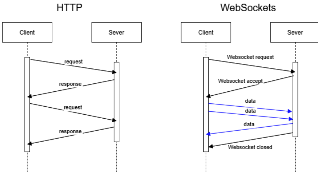
Figure 3.9 – Comparison of HTTP and WebSocket
