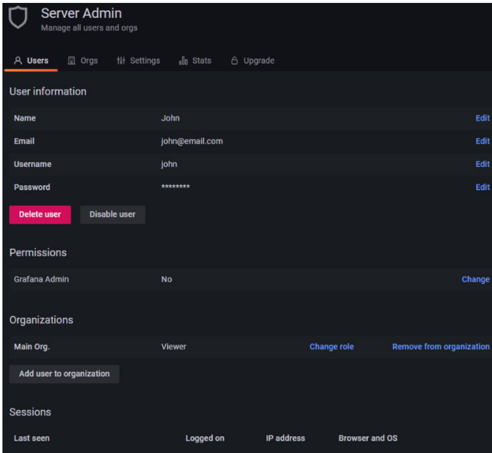
Figure 2.7 – Assigning roles and permissions
