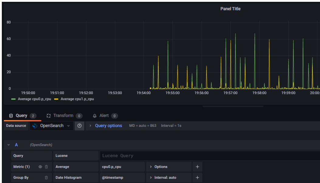
Figure 12.3 – Building queries for an OpenSearch data source
