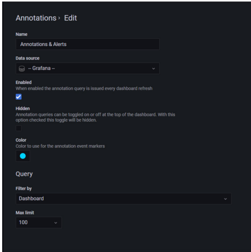
Figure 8.9 – Built-in annotation configuration
