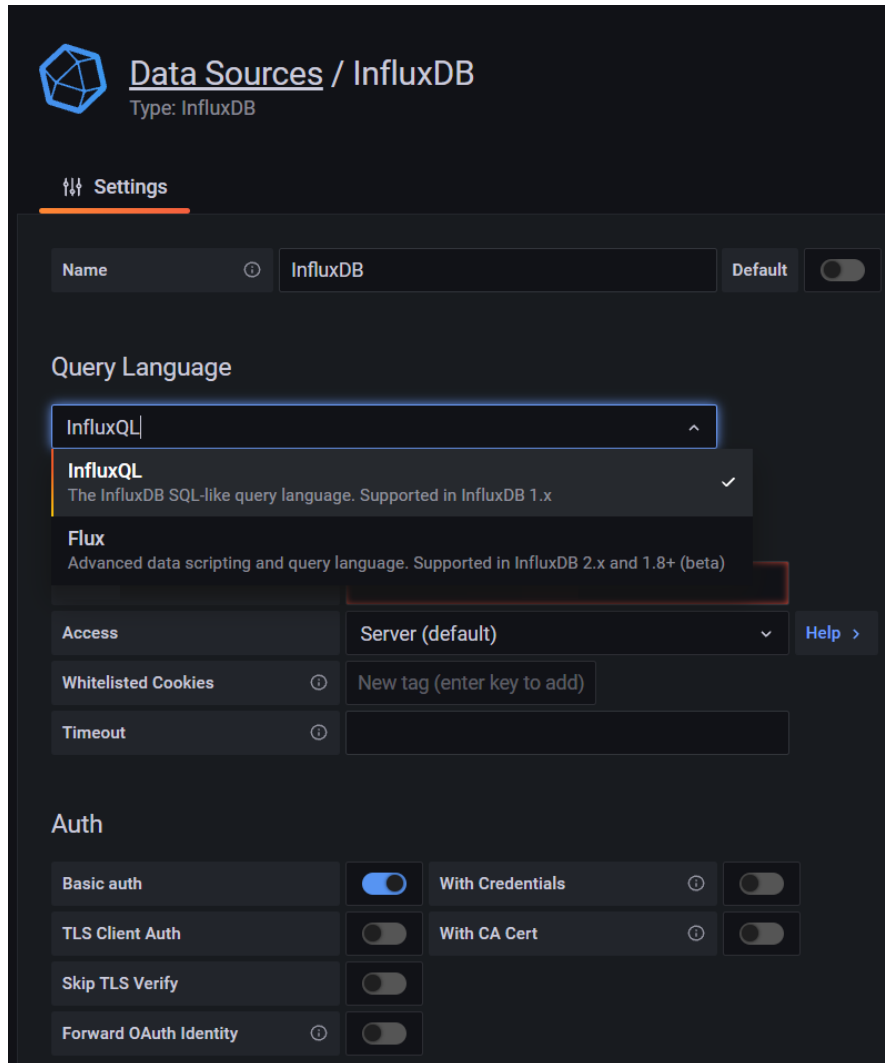
Figure 5.6 – Selecting the query language
