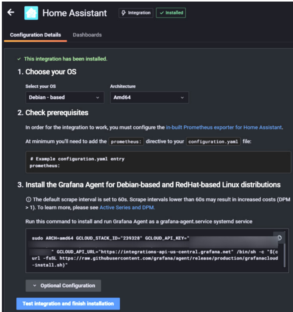
Figure 14.5 – Configuration page of the Home Assistant integration
