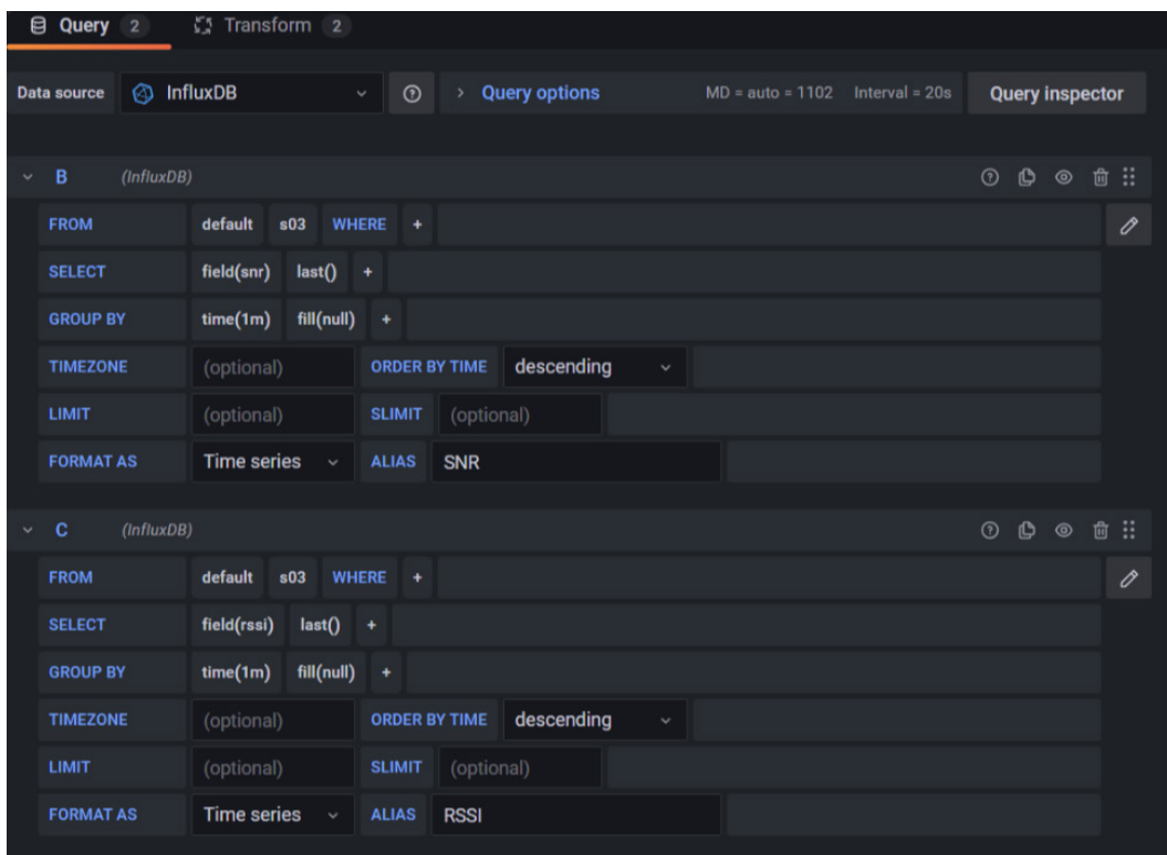
Figure 6.11 – Running two queries
