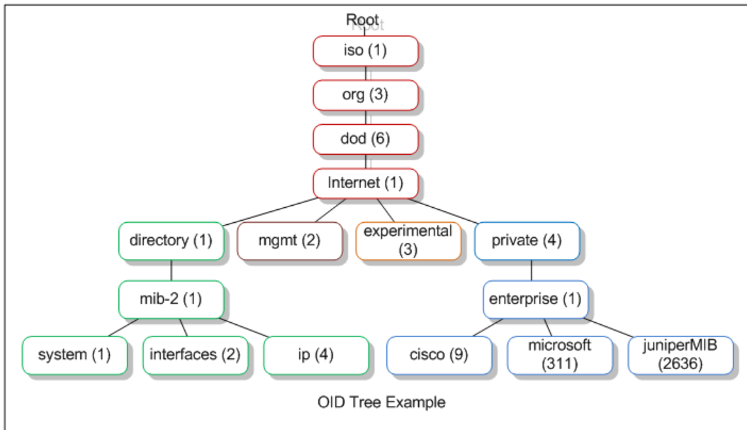
Figure 13.2 – OID tree example
