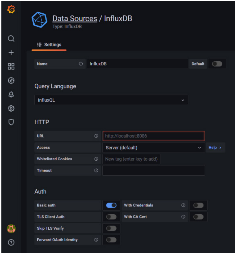
Figure 5.7 – Configuring the InfluxDB data source
