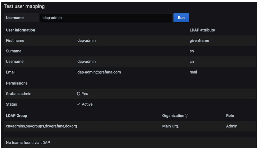
Figure 2.10 – Showing LDAP user information
