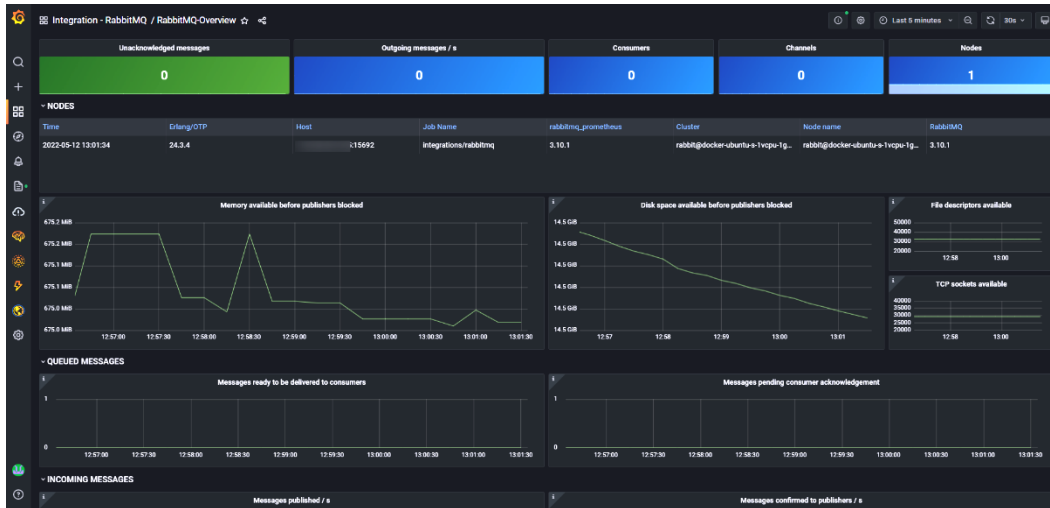
Figure 14.9 – Dashboard of the RabbitMQ integration
