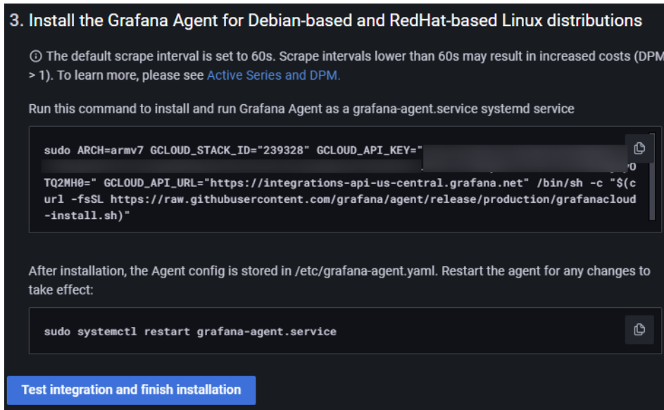
Figure 14.3 – Installing the agent in the Linux node
