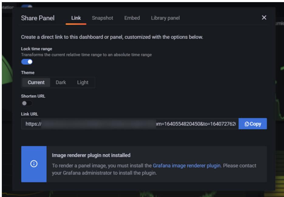
Figure 8.26 – Sharing a panel link
