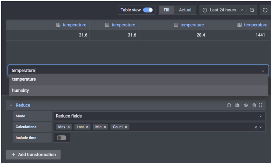
Figure 9.9 – Reduce transformation (Reduce fields)
