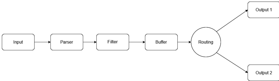
Figure 12.2 – The data pipeline of Fluent Bit
