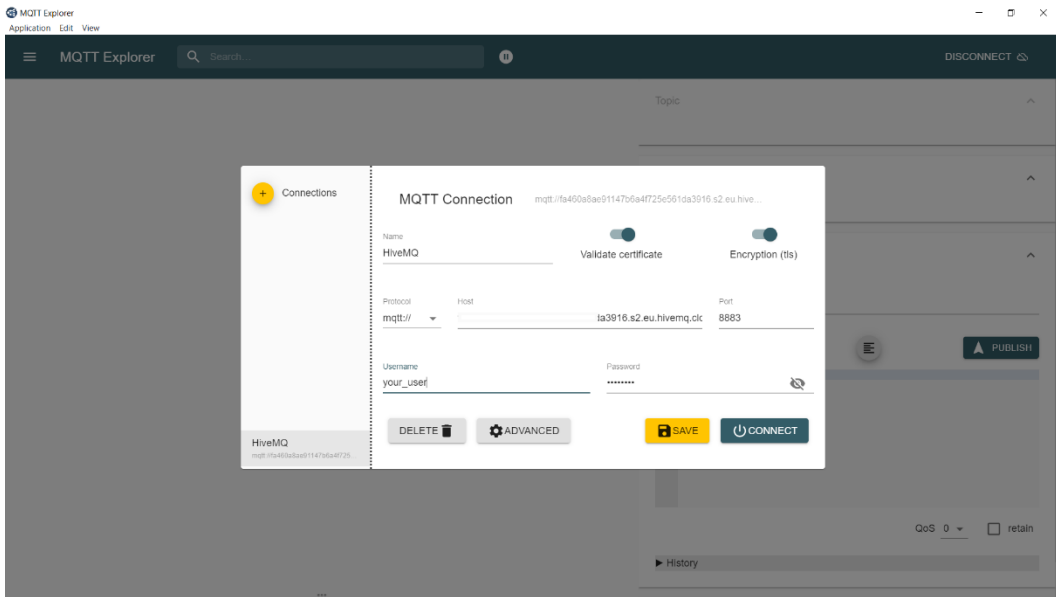
Figure 3.8 – Testing connection with MQTT Explorer
