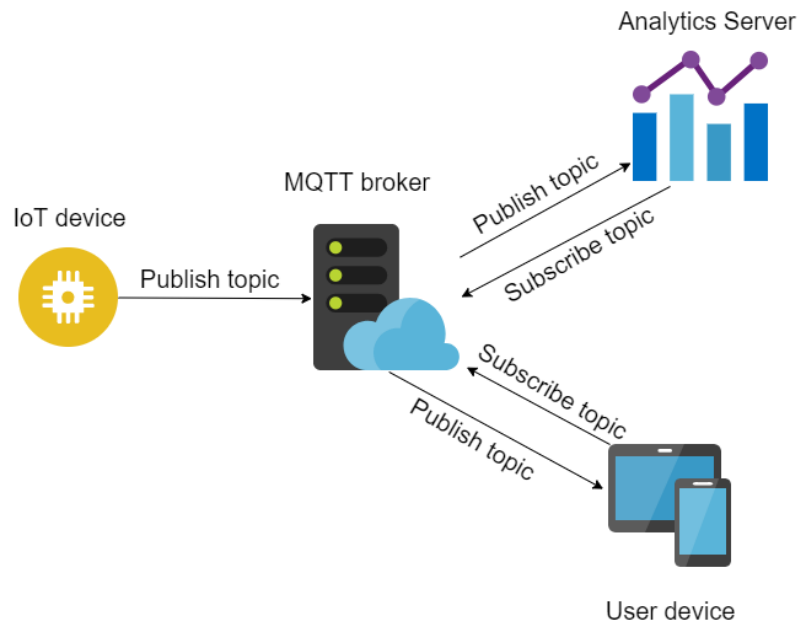
Figure 3.1 – MQTT architecture
