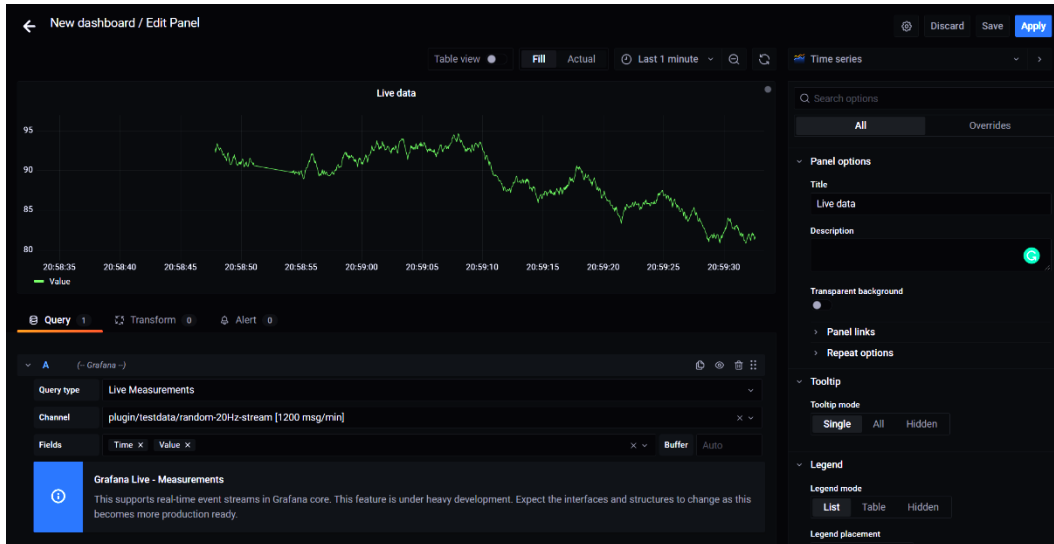
Figure 4.16 – Live data dashboard
