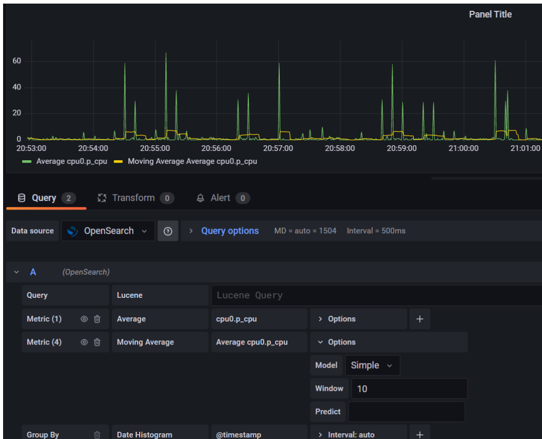
Figure 12.4 – Using aggregations in OpenSearch data
