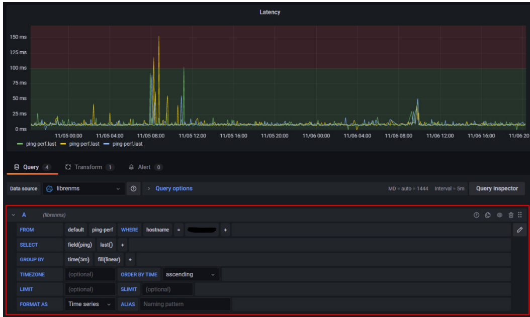
Figure 6.2 – The Query Inspector
