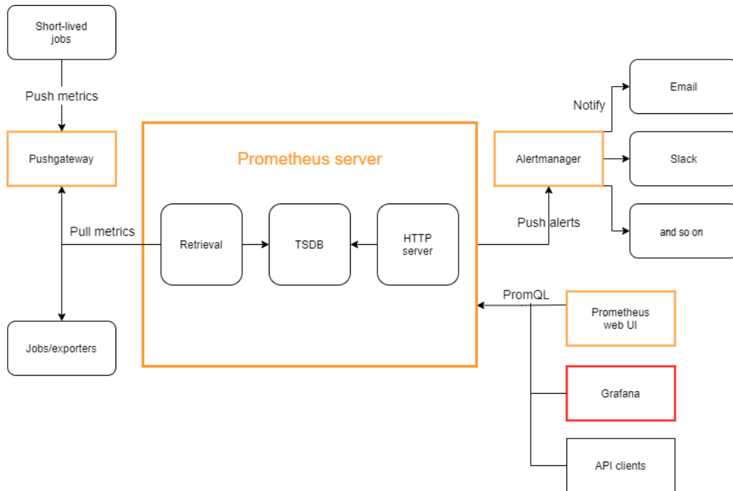
Figure 11.1 – The architecture of Prometheus and its external systems
