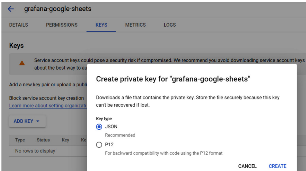
Figure 4.10 – Creating a private key
