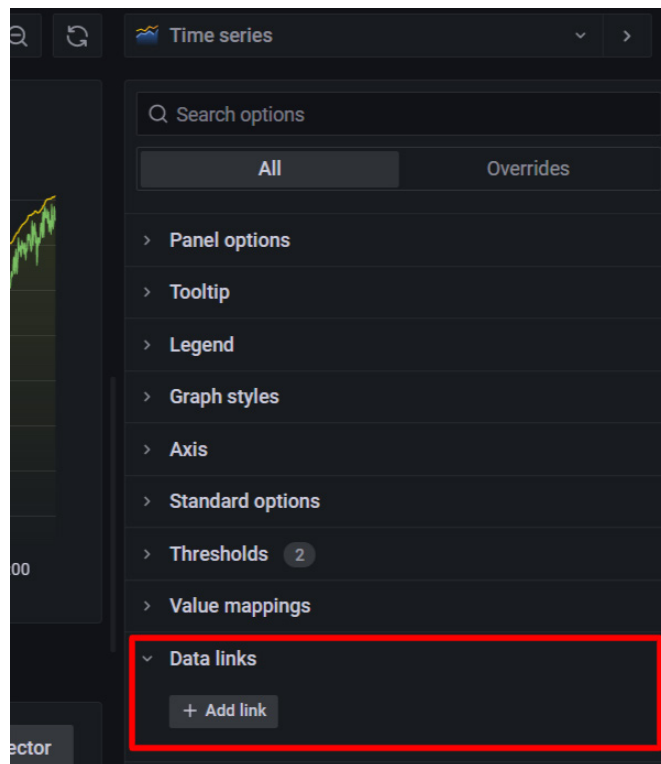
Figure 8.21 – Adding a data link
