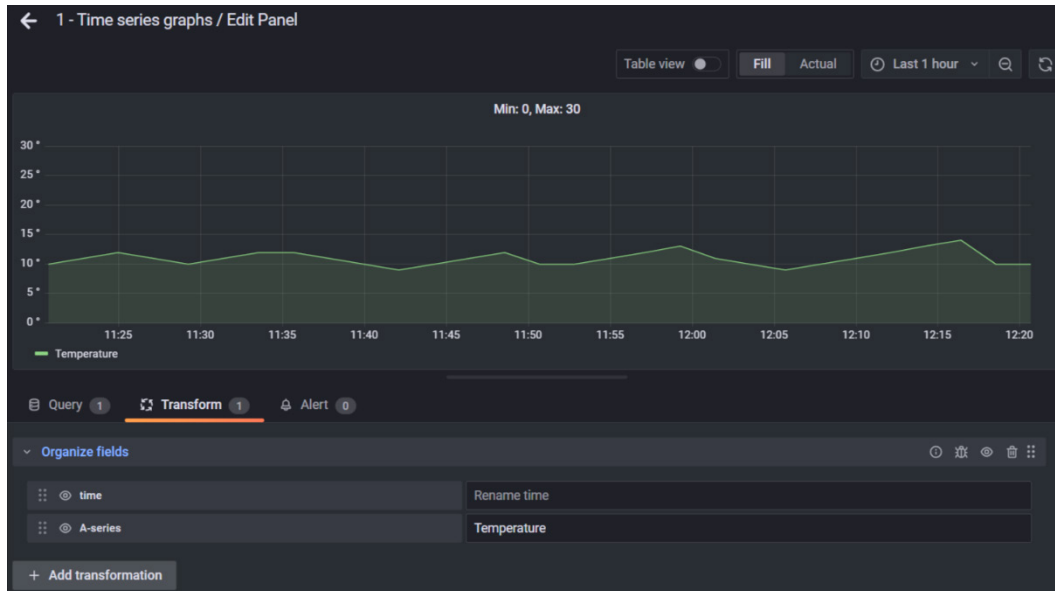
Figure 9.6 – Organize fields transformation
