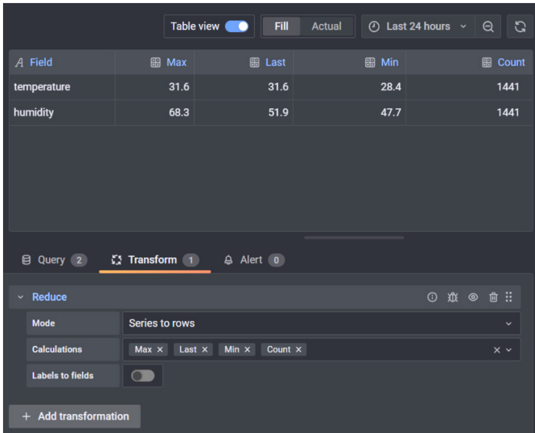
Figure 9.8 – Reduce transformation (Series to rows)
