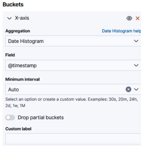
Figure 12.12 – Selecting the aggregation and the field for the X axis
