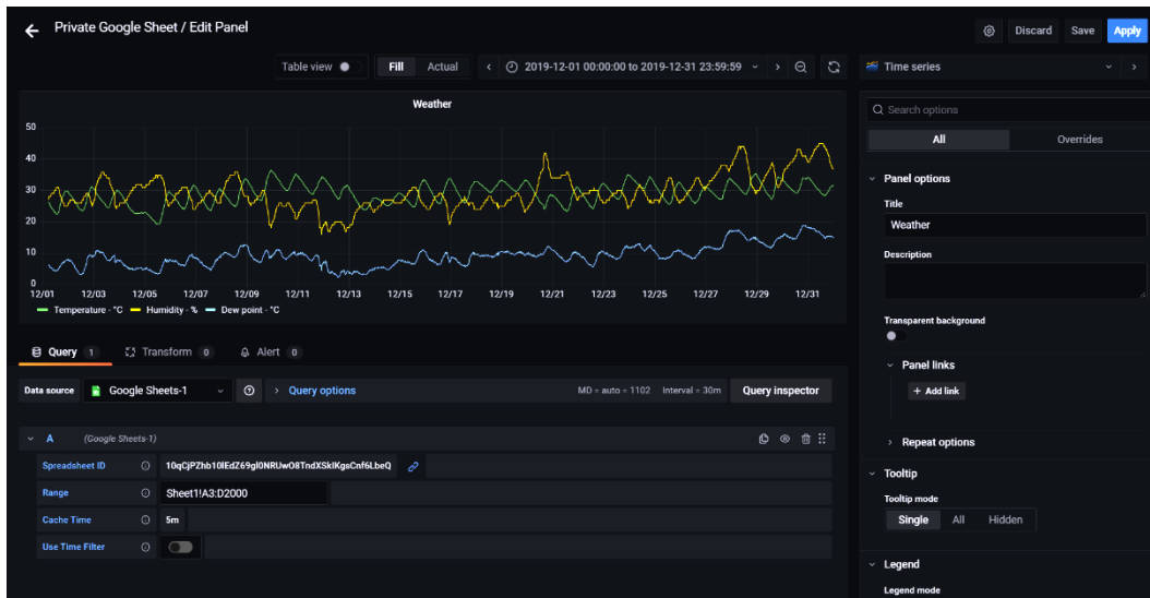
Figure 4.11 – Showing data from private Google Sheets
