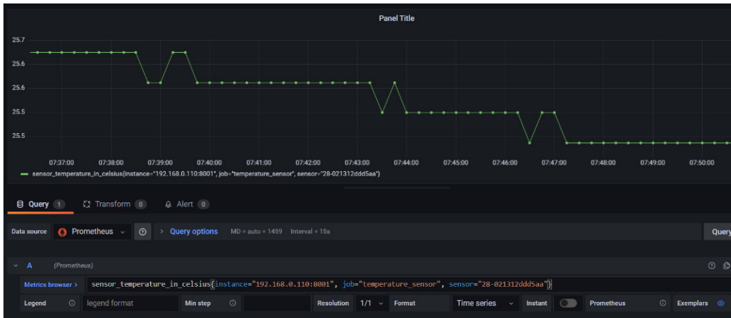
Figure 11.6 – Graphing values in Grafana from Prometheus metrics
