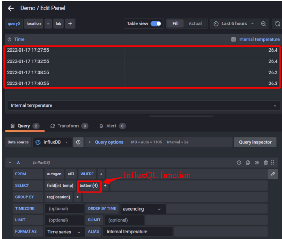
Figure 9.2 – Example of a selector function in an InfluxDB data source
