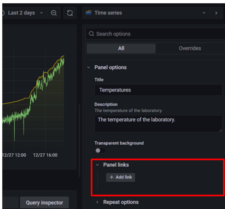
Figure 8.20 – Adding a panel link
