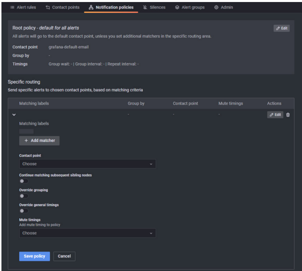
Figure 10.9 – Adding a new notification policy
