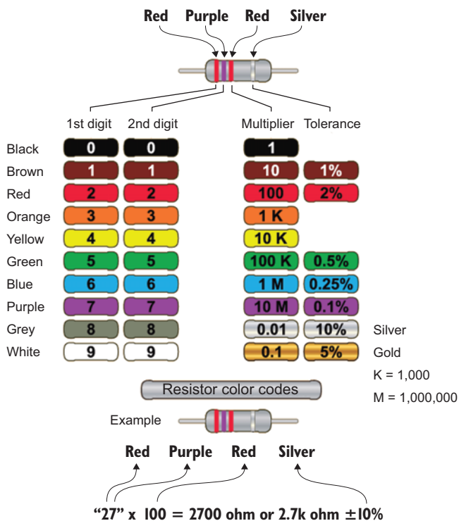
Figure 7.9 The colored bands on a resistor tell you how much resistance the resistor has. For this project, you want a brown (1), grey (8), brown ( \times 10 ) resistor, or 18 \times 10 = 180 ohm resistor. Don't have one? Any resistor between about 100 and 300 ohms should work well.
