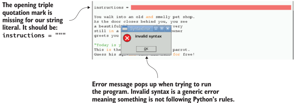
Figure 4.7 A string literal must start and end with a set of triple quotation marks. If you forget, Python will tell you that you have a syntax error. Add the missing triple quotes to fix the error.
