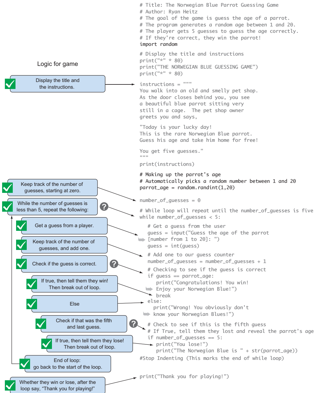
Figure 4.15 To randomly select a number, you need to import the random library and use the randint function to select a random integer between 1 and 20.
