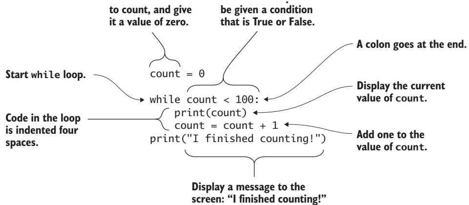
Figure 4.14 You can use a while loop to repeatedly perform a task. Code that is part of the loop is indented four spaces. In this case, this while loop displays the numbers from 0 to 99; when completed, it prints the message, “I finished counting!” Typically, the condition should be such that code in the loop can make it False and thus end the loop.
