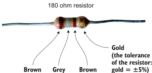
Figure 6.13 The value of a resistor is determined by its colored bands. See the sidebar “Resistor color codes” for a chart; there are also many online color-code charts.
