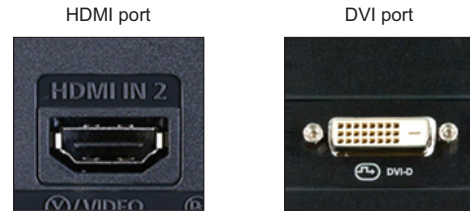
Figure 1.8 HDMI and DVI are common types of video input ports found on modern TVs and monitors. It's easiest to connect a Raspberry Pi to a TV or monitor with an HDMI port. HDMI provides a high-definition picture and doesn't require any adapters or converters—only an HDMI cable, which is included in many Pi kits. The DVI port requires a special adapter to connect with a Pi.
