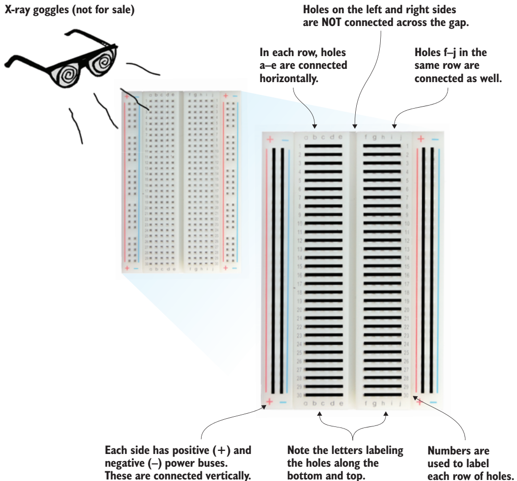
Figure 6.7 Breadboards have internal connections. You need to know about them in order to build circuits. Rows of pins are connected horizontally, but not across the gap in the middle. Long rails called power buses run vertically along the sides of the board.
