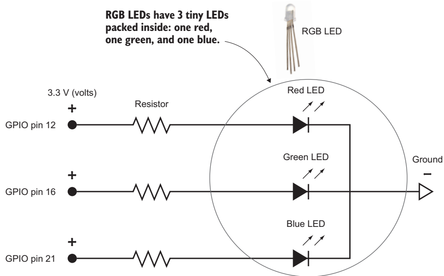
Figure 7.4 Circuit diagram for the Light Up Guessing Game project
