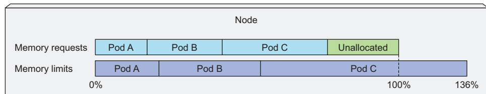
Figure 14.3 The sum of resource limits of all pods on a node can exceed 100% of the node's capacity.
