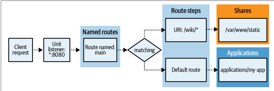
Figure 4-2. Simple NGINX Unit configuration
