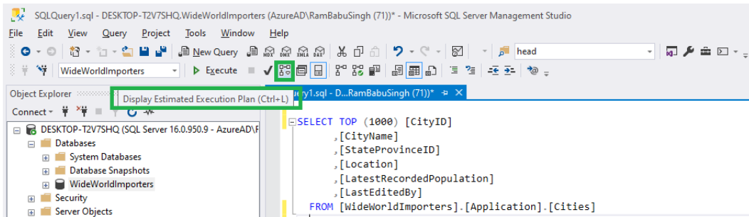
Figure 9.2 – The Display Estimated Execution Plan option on the toolbar
