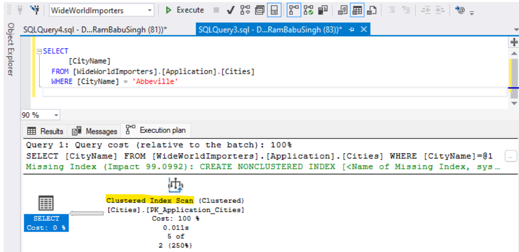
Figure 9.24 – The actual execution plan using a clustered index scan and recommending an index
